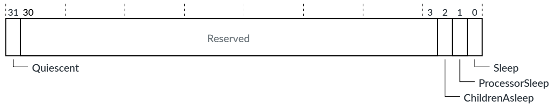
Figure 5-43: GICR_WAKER bit assignments
