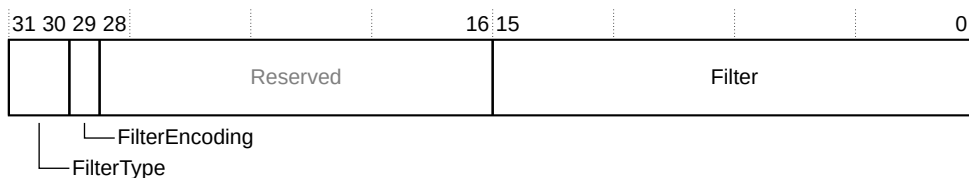
Figure 5-89: GICP_FRn bit assignments
