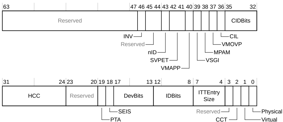
Figure 5-66: GITS_TYPER bit assignments
