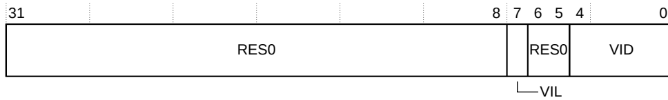
Figure 5-4: GIC_TYPER2 bit assignments
