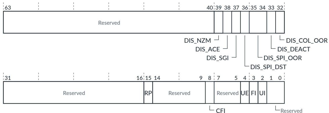
Figure 5-76: GICT_ERR<n>CTLR bit assignments
