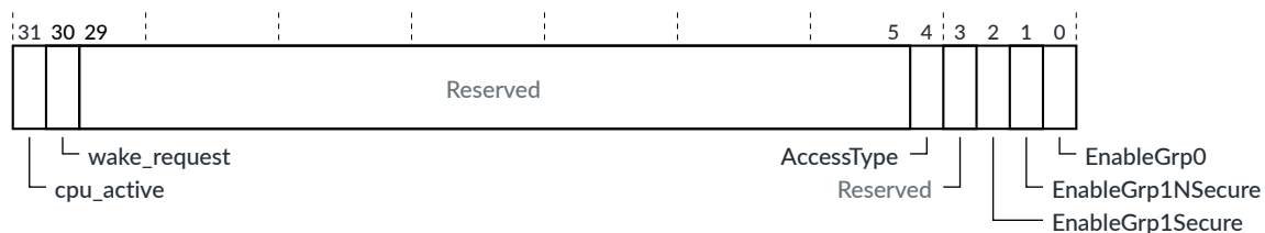
Figure 5-53: GICR_MISCSTATUSR bit assignments
