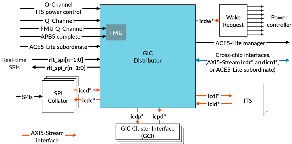
Figure 3-1: GIC-720AE Distributor
