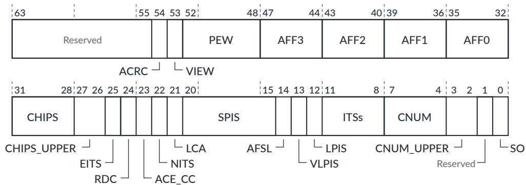
Figure 5-28: GICD_CFGID bit assignments
