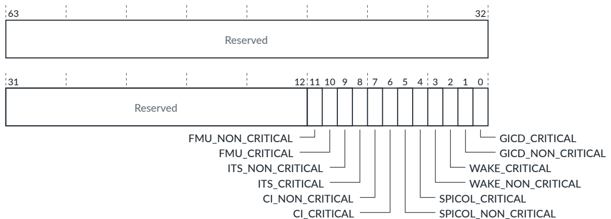
Figure 5-105: FMU_ERRGSR bit assignments
