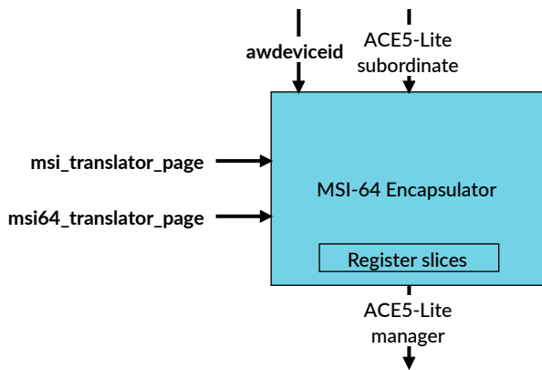
Figure 3-5: MSI-64 Encapsulator
