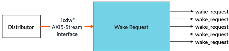
Figure 3-8: Wake Request
