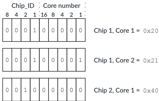
Figure 4-5: ProcessorNumber fields
