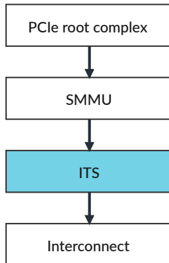
Figure 3-4: ITS integration
