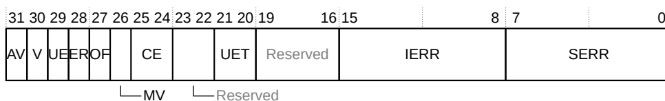
Figure 5-77: GICT_ERR<n>STATUS bit assignments
