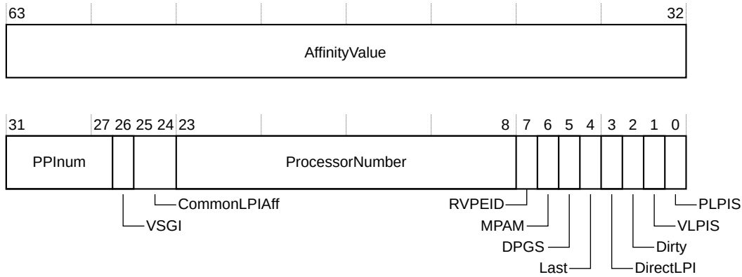
Figure 5-42: GIC_TYPER bit assignments
