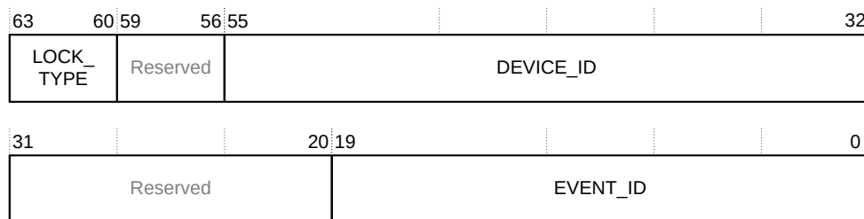
Figure 5-71: GITS_OPR bit assignments
