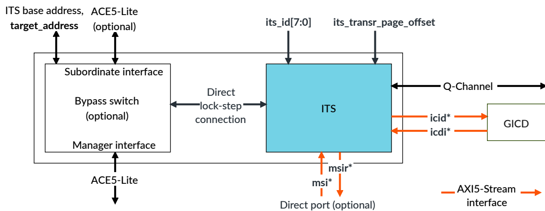
Figure 3-3: ITS block
