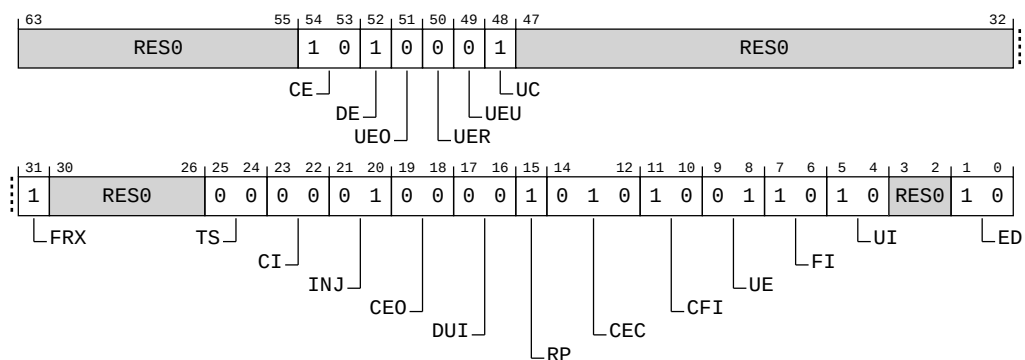
Figure B-217: EXT_ERR0FR bit assignments
