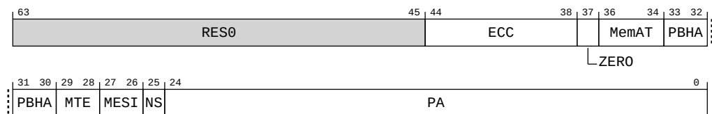
Figure A-79: AARCH64_IMP_L2_DATA0_EL3 bit assignments
