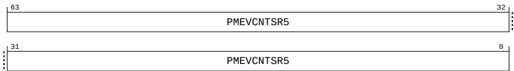
Figure B-170: PMU_PMEVCNTR5 bit assignments
