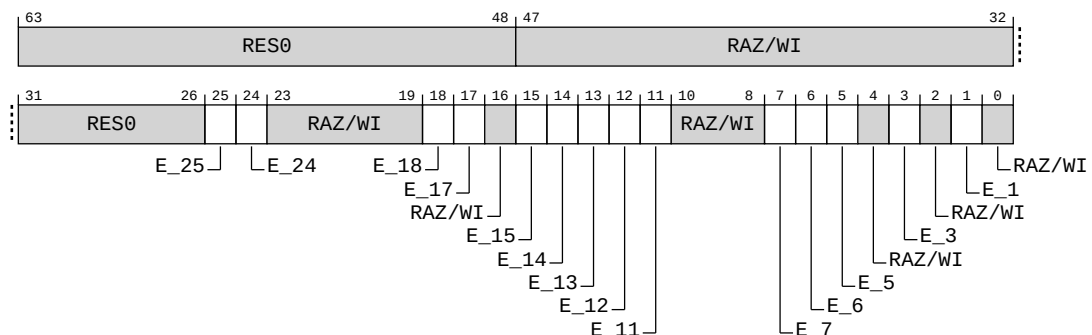
Figure A-167: AARCH64_PMSNEVFR_EL1 bit assignments
