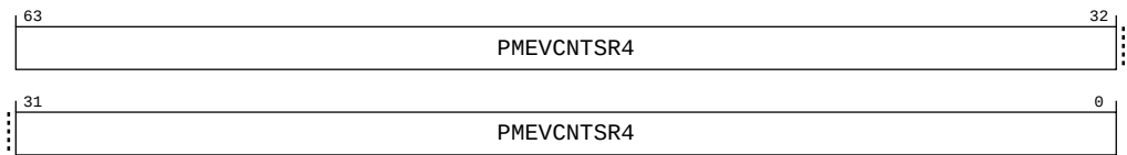
Figure B-169: PMU_PMEVCNTR4 bit assignments
