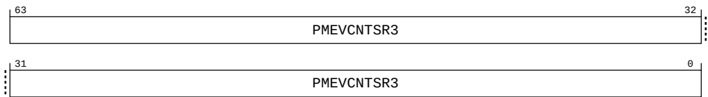
Figure B-168: PMU_PMEVCNTR3 bit assignments
