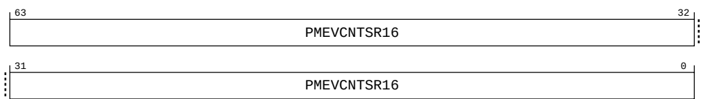
Figure B-181: PMU_PMEVCNTR16 bit assignments
