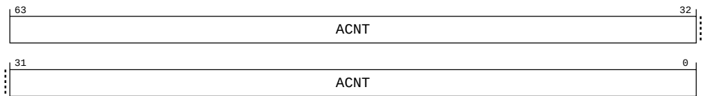
Figure B-9: AMU_AMEVCNTR14 bit assignments
