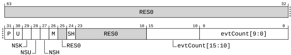
Figure B-136: PMU_PMEVTYPER7_ELO bit assignments
