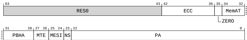
Figure A-77: AARCH64_IMP_L2_DATA0_EL3 bit assignments
