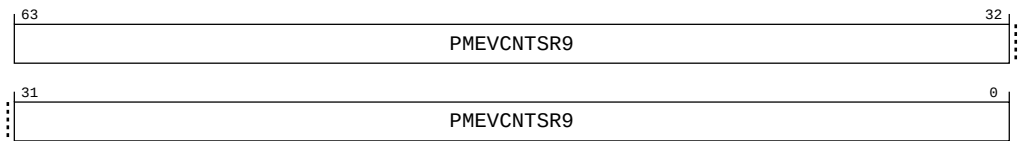
Figure B-174: PMU_PMEVCNTR9 bit assignments
