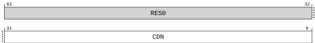
Figure A-152: AARCH64_ERXPGCDN_EL1 bit assignments
