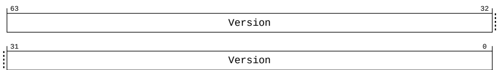
Figure A-129: AARCH64_REVIDR_EL1 bit assignments
