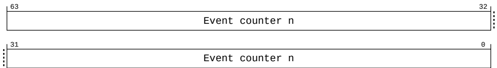
Figure B-102: PMU_PMEVCNTR4_ELO bit assignments
