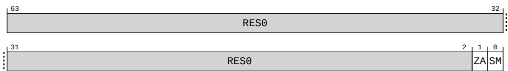
Figure A-99: AARCH64_SVCR bit assignments
