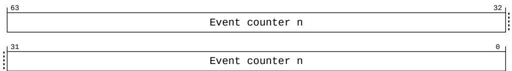
Figure B-107: PMU_PMEVCNTR9_ELO bit assignments
