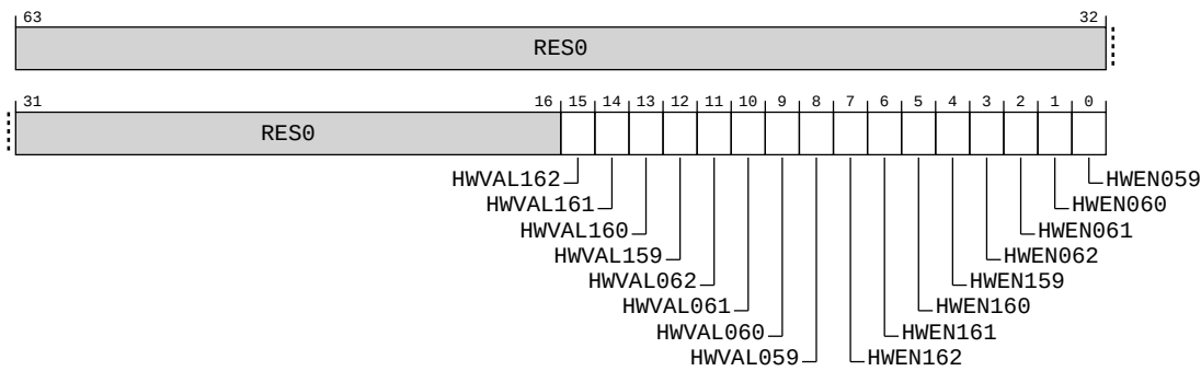
Figure A-40: AARCH64_IMP_ATCR_EL2 bit assignments
