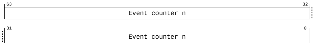
Figure B-103: PMU_PMEVCNTR5_ELO bit assignments
