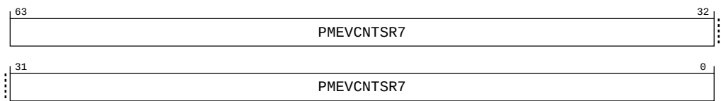
Figure B-172: PMU_PMEVCNTR7 bit assignments
