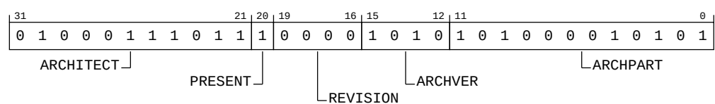
Figure B-41: EXT_EDDEVARCH bit assignments
