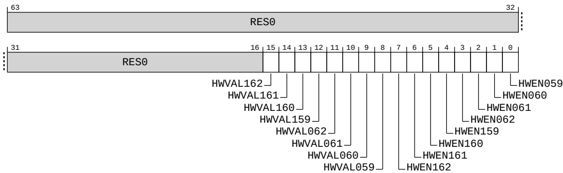
Figure A-39: AARCH64_IMP_ATCR_EL1 bit assignments
