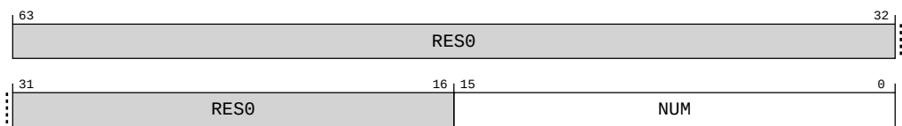
Figure A-143: AARCH64_ERRIDR_EL1 bit assignments
