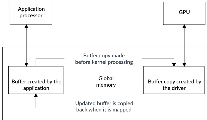
Figure 8-2: Memory buffer created by clCreateBuffer(CL_MEM_USE_HOST_PTR)
