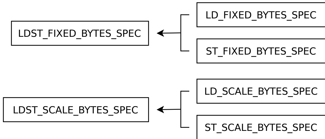
Figure 1: Byte counting
