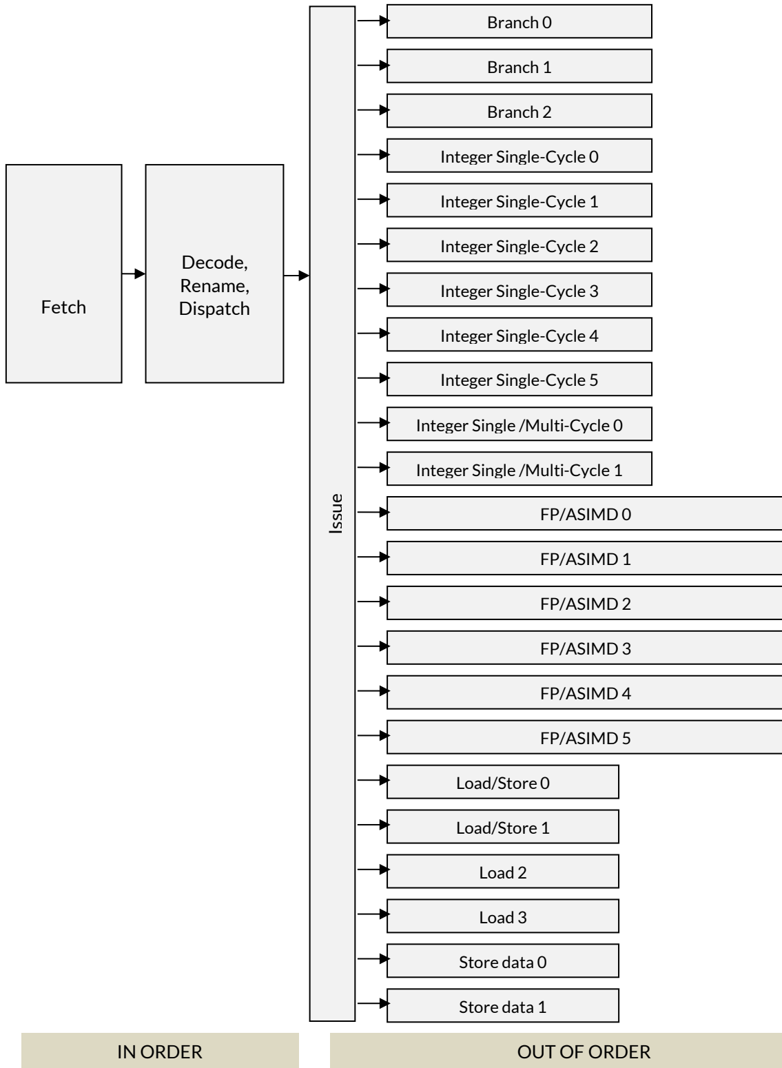
Figure 2-1 Cortex-X925 core pipeline
