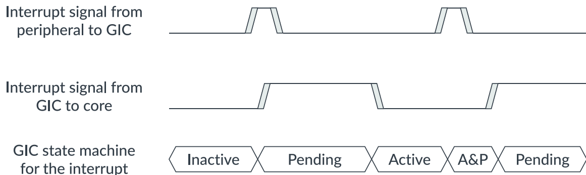
Figure 4-5: Timing edge-triggered
