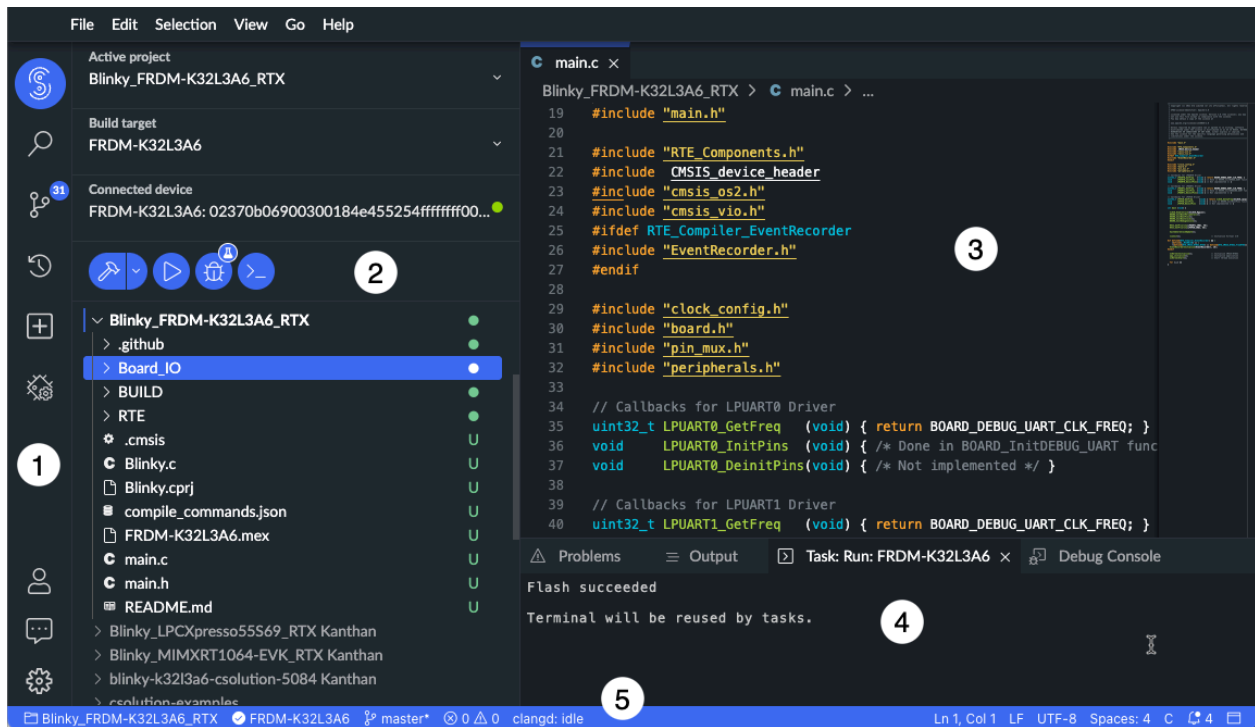
Figure 4-2: UI layout
