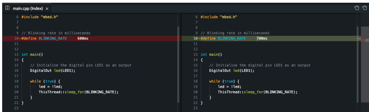
Figure 11-2: Double-click a file to view its side-by-side comparison
