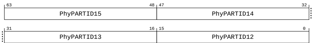
Figure A-262: AArch64_mpamvpm3_el2 bit assignments
