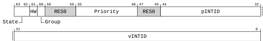
Figure A-169: AArch64_ich_lr3_el2 bit assignments
