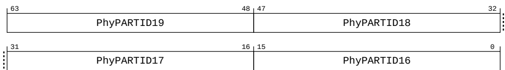
Figure A-263: AArch64_mpmvpm4_el2 bit assignments
