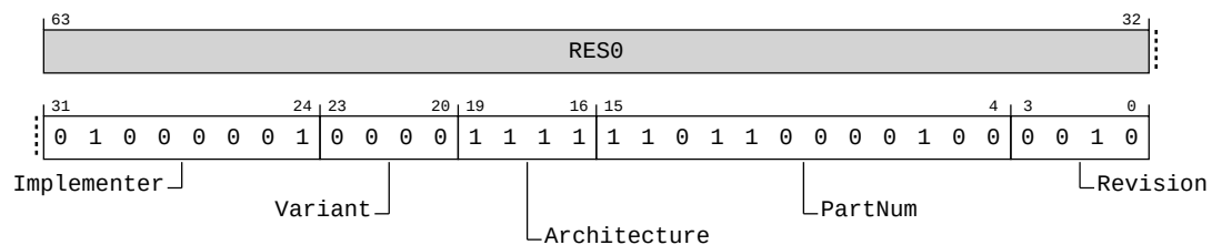
Figure A-118: AArch64_midr_el1 bit assignments
