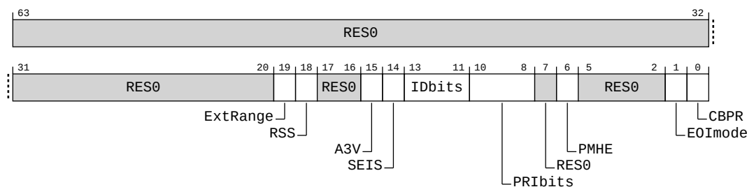
Figure A-161: AArch64_icc_ctlr_el1 bit assignments
