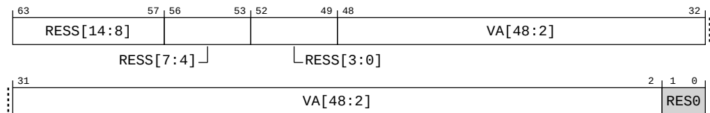
Figure B-131: ext_dbgwvr1_el1 bit assignments
