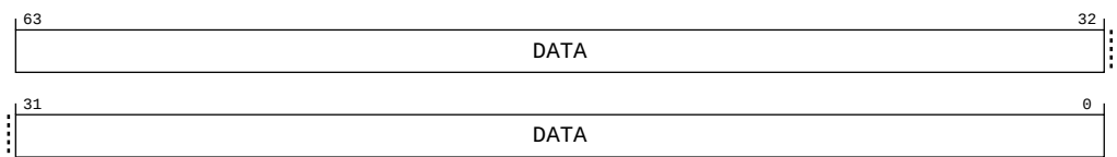
Figure A-109: AArch64_imp_idata0_el3 bit assignments
