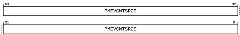
Figure B-57: ext_pmevcntr29 bit assignments
