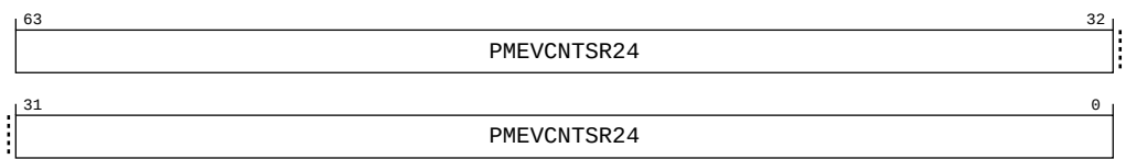
Figure B-52: ext_pmevcntr24 bit assignments
