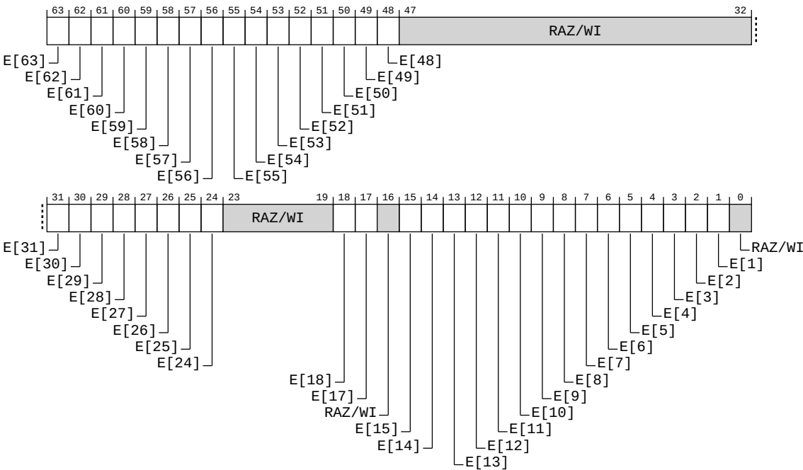
Figure A-267: AArch64_pmsnevfr_el1 bit assignments
