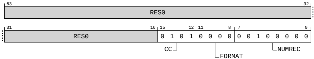
Figure A-212: AArch64_brbidr0_el1 bit assignments
