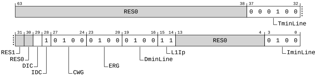
Figure A-139: AArch64_ctr_el0 bit assignments
