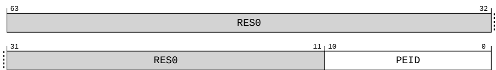
Figure A-116: AArch64_imp_cpurndpeid_el3 bit assignments
