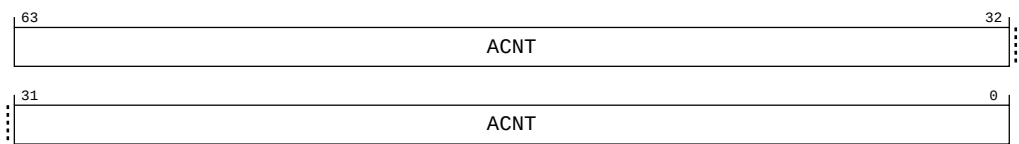
Figure A-197: AArch64_amevcntr11_el0 bit assignments
