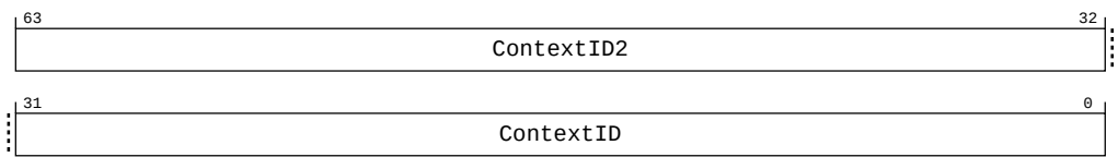
Figure B-87: ext_dbgbvr0_el1 bit assignments
