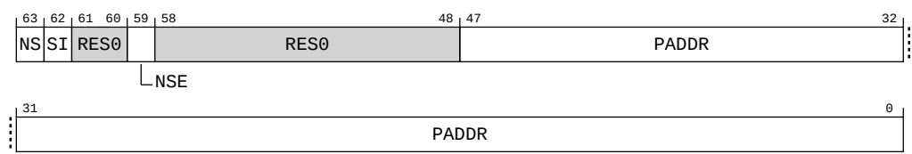
Figure B-224: ext_err0addr bit assignments
