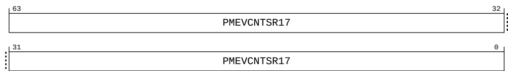
Figure B-45: ext_pmevcntr17 bit assignments
