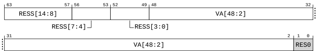
Figure B-113: ext_dbgivr4_el1 bit assignments
