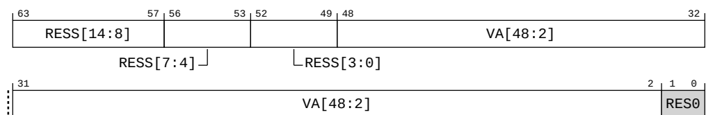
Figure B-105: ext_dbgvr3_el1 bit assignments
