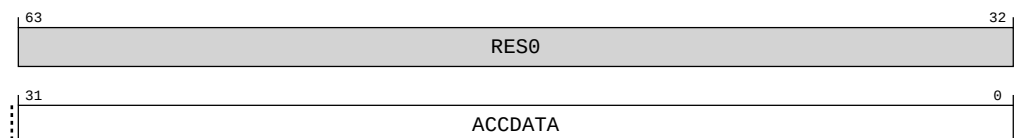
Figure A-171: AArch64_accdata_el1 bit assignments
