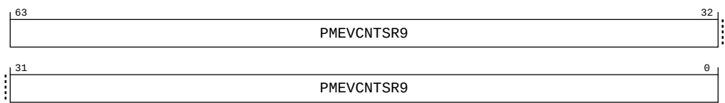
Figure B-37: ext_pmevcntr9 bit assignments
