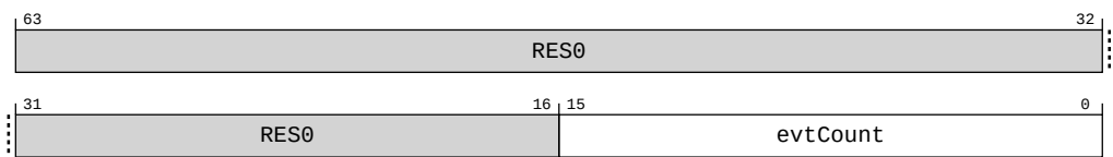
Figure A-200: AArch64_amevtyper11_el0 bit assignments
