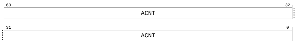
Figure B-162: ext_amevcntr11 bit assignments
