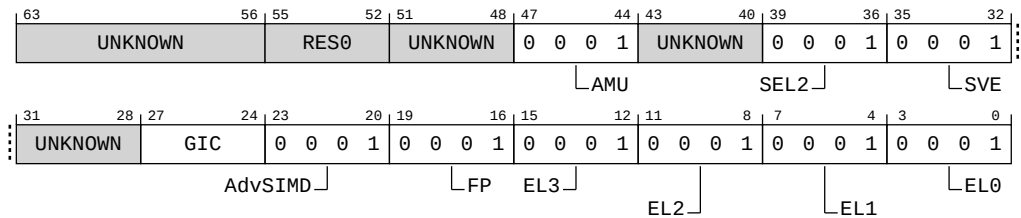
Figure B-138: ext_edpfr bit assignments
