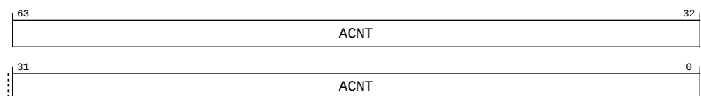
Figure A-191: AArch64_amevcntr03_el0 bit assignments
