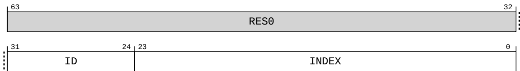
Figure A-117: AArch64_sys_imp_ramindex bit assignments
