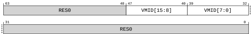
Figure A-76: AArch64_dbgvr2_el1 bit assignments
