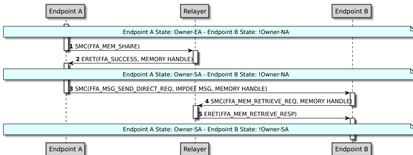
Figure 1.4: Share Memory Transaction Lifecycle
