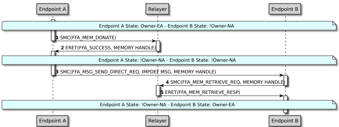
Figure 1.2: Donate Memory Transaction Lifecycle
