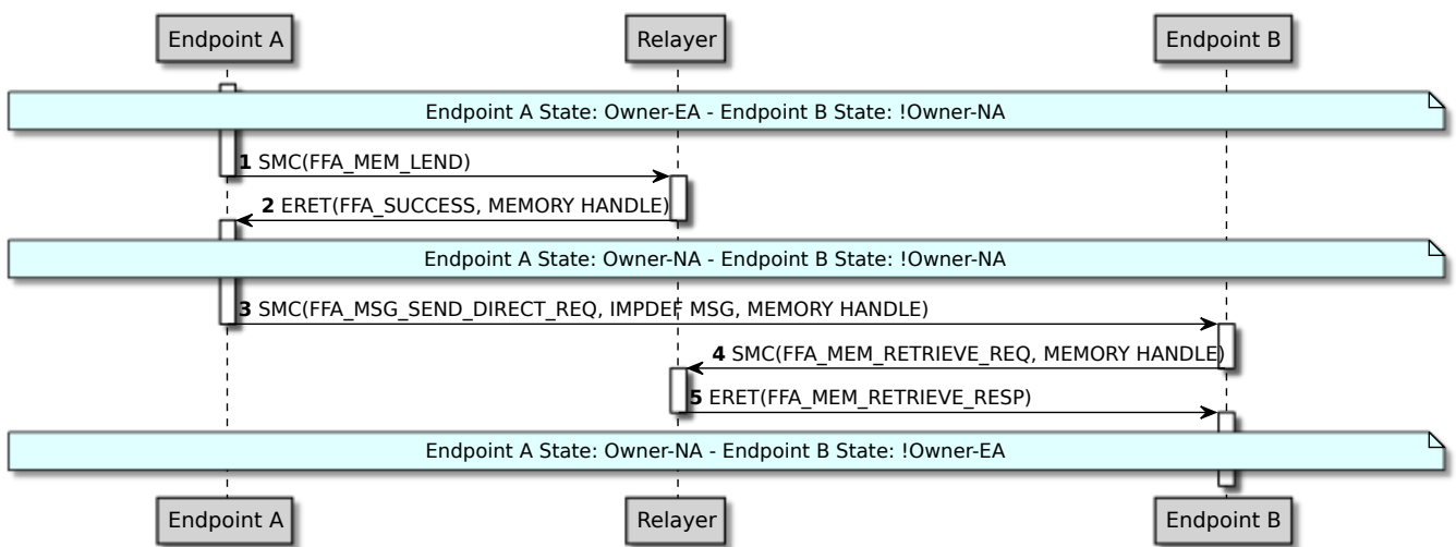
Figure 1.3: Lend Memory Transaction Lifecycle
