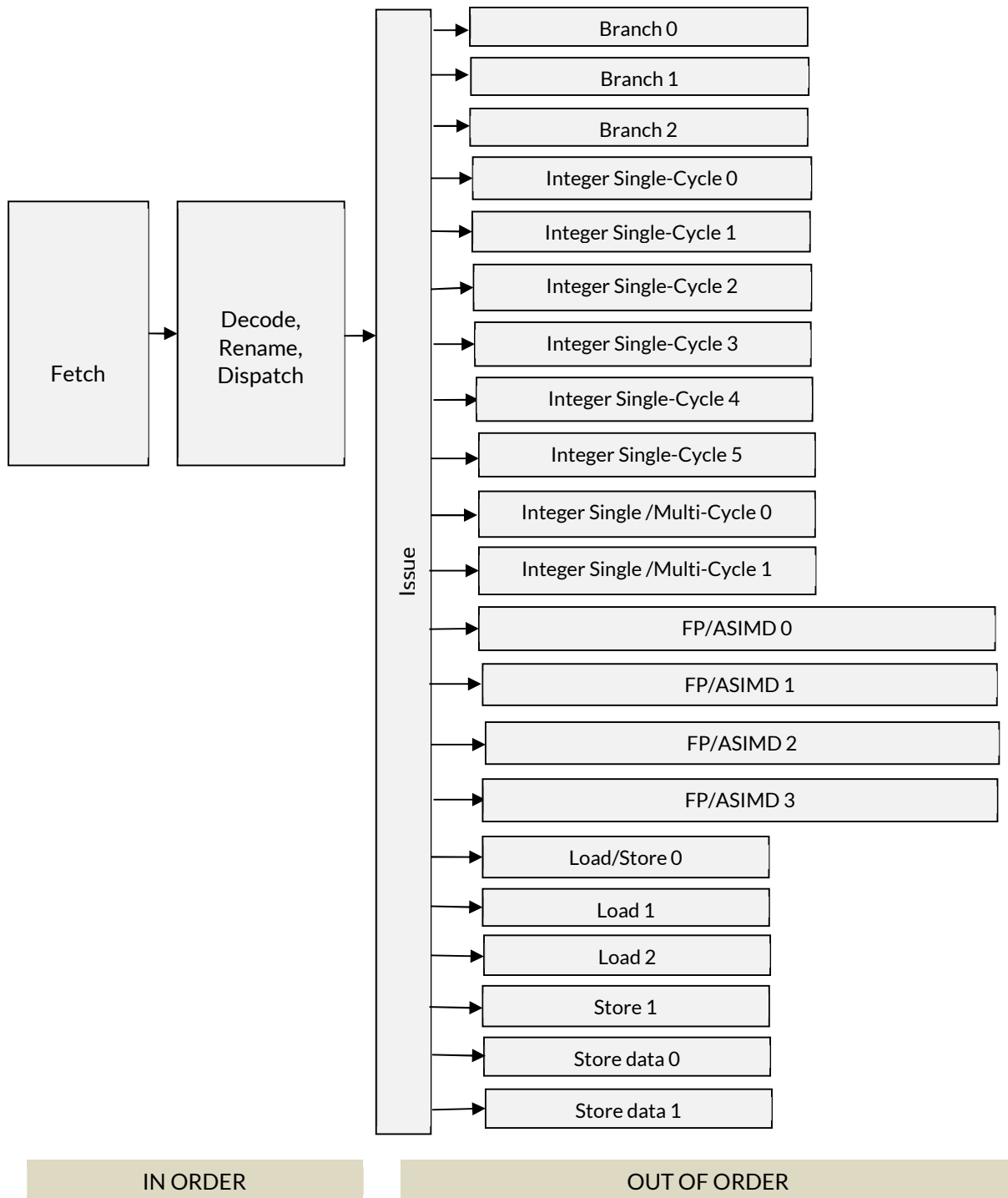
Figure 2-1 Neoverse V3 core pipeline
