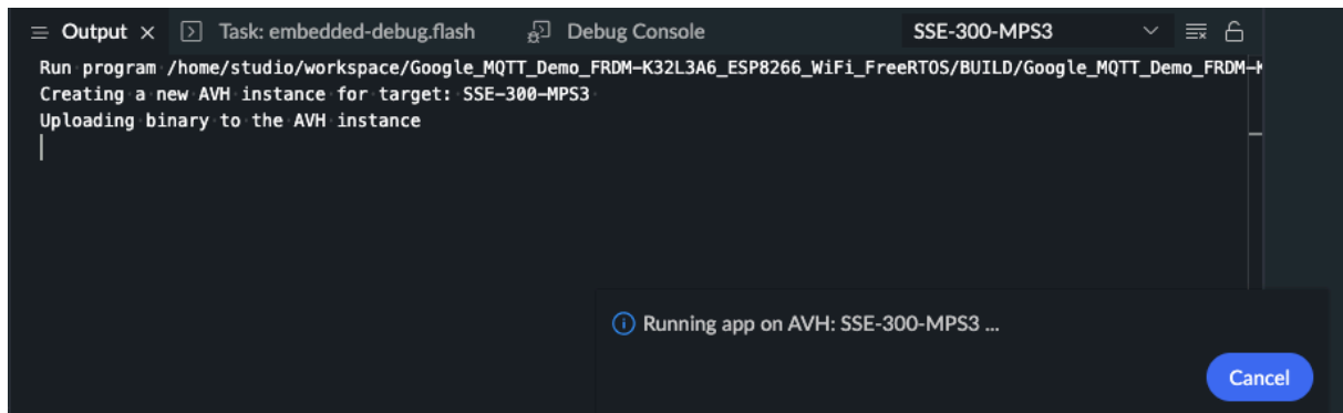
Figure 14-2: Output
