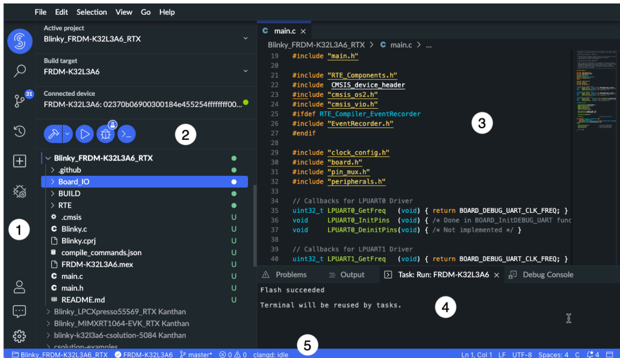
Figure 5-2: UI layout
