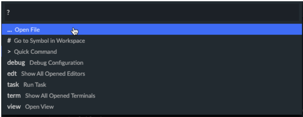
Figure 5-4: Available commands
