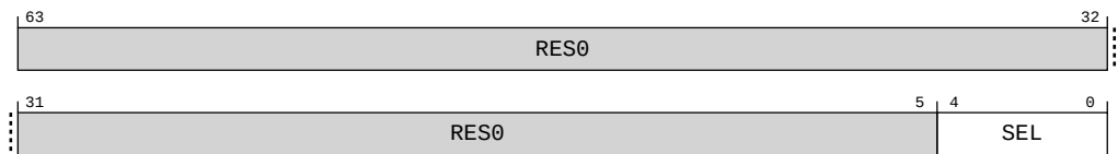
Figure A-27: AArch64_imp_clusterpmselr_el1 bit assignments
