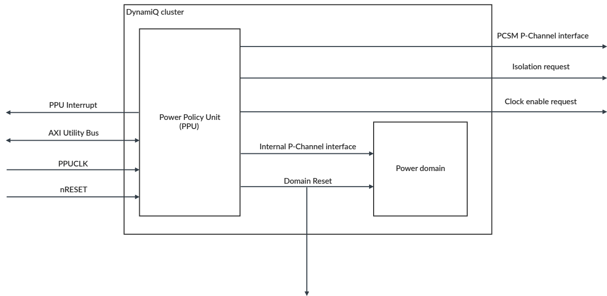
Figure 6-1: DSU-120 PPU interfaces
