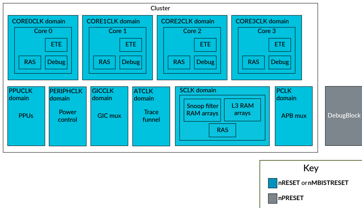
Figure 4-2: DSU-120 pin-controlled reset domains
