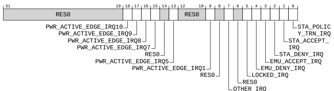
Figure B-132: ext_ppu_isr bit assignments
