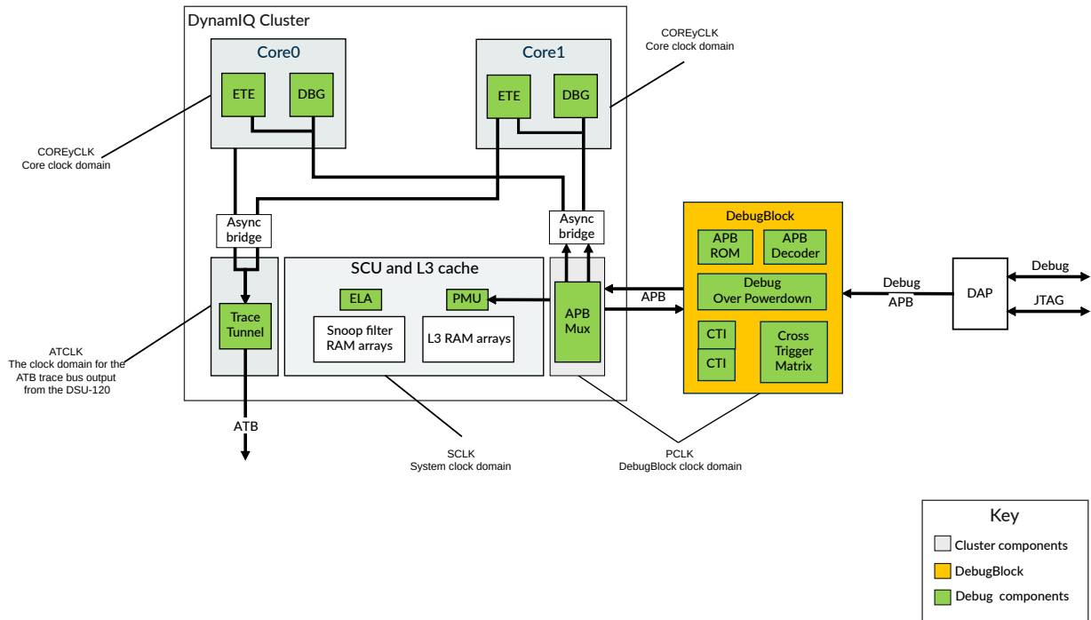
Figure 15-1: Cluster debug components
