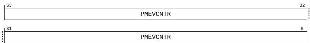
Figure B-354: ext_clusterpmu_pmevcntr5 bit assignments
