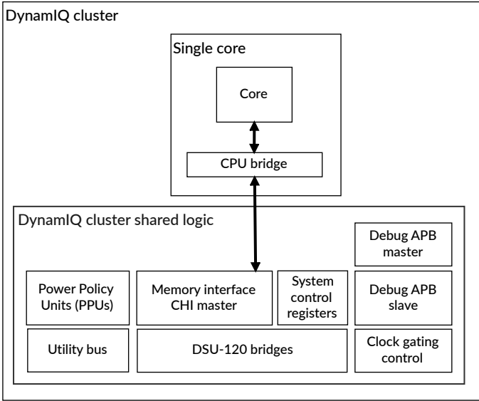
Figure 2-8: L3 Direct connect implementation
