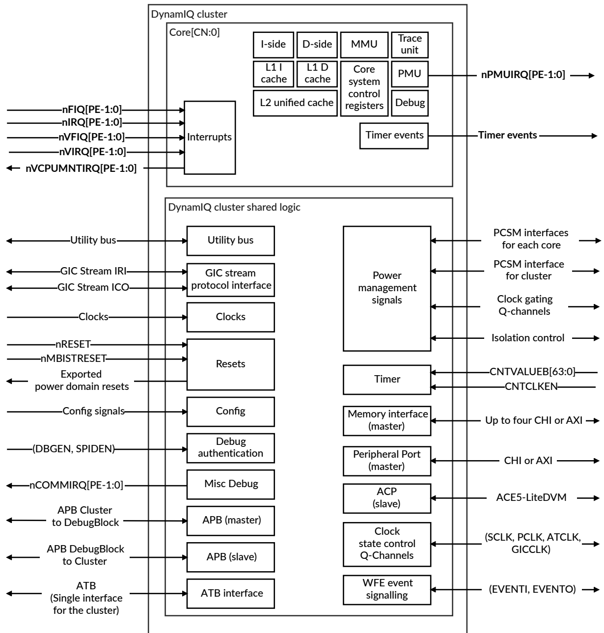
Figure 3-4: DSU-120 DynamIQ™ cluster interfaces
