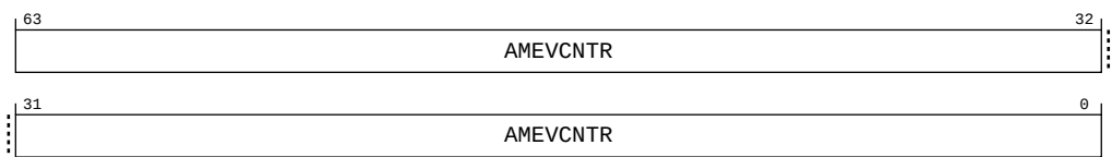
Figure B-93: ext_clusteramu_amevcntr0 bit assignments
