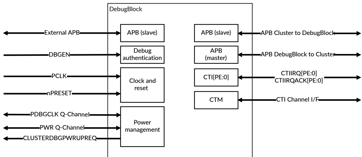
Figure 3-5: DebugBlock interfaces
