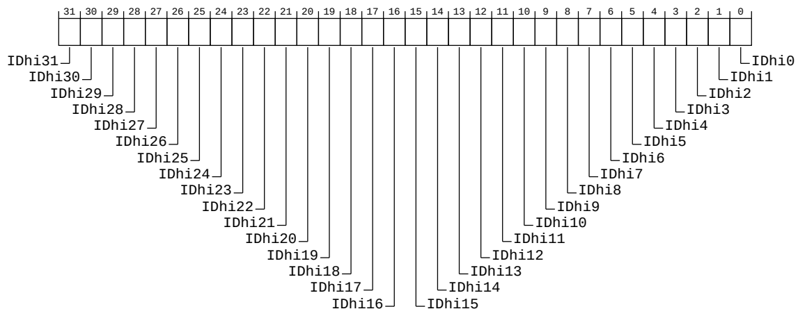
Figure B-381: ext_clusterpmu_pmceid3 bit assignments
