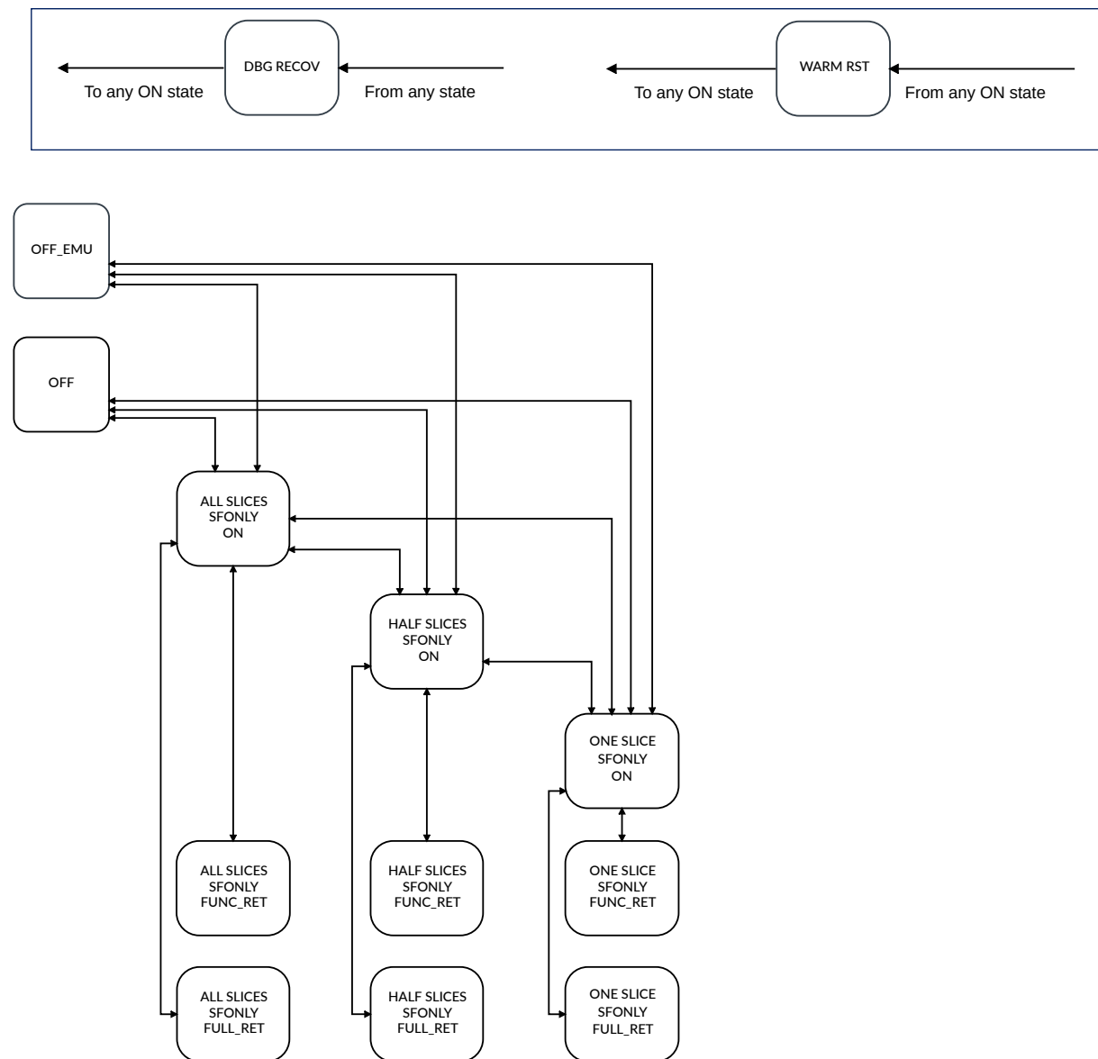
Figure 5-3: DSU-120 DynamIQ™ cluster PPU mode transitions, no L3 cache
