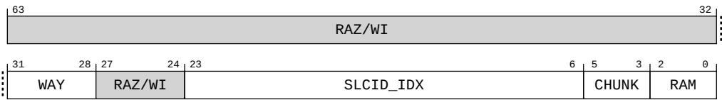
Figure A-20: AArch64_imp_clustercdbg_el3 bit assignments
