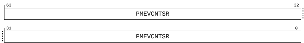
Figure B-362: ext_clusterpmu_pmevcntrs1 bit assignments
