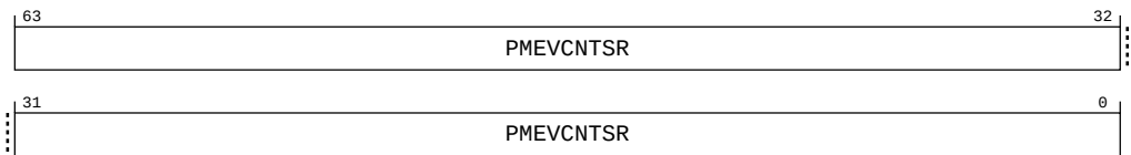
Figure B-361: ext_clusterpmu_pmevcntr0 bit assignments
