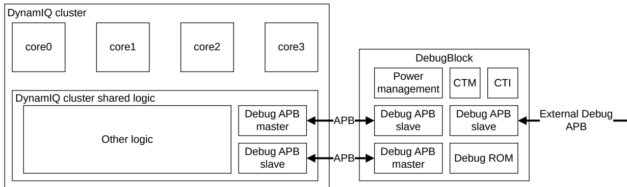
Figure 3-3: DebugBlock components
