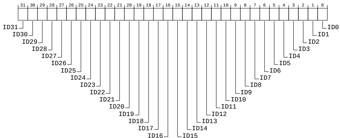
Figure B-378: ext_clusterpmu_pmceid0 bit assignments
