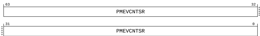
Figure B-366: ext_clusterpmu_pmevcntrs5 bit assignments
