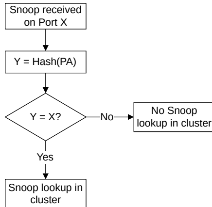
Figure 8-1: External snoop handling on CHI master port
