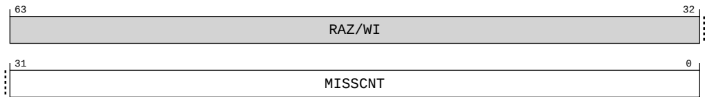
Figure A-15: AArch64_imp_clusterl3miss_el1 bit assignments
