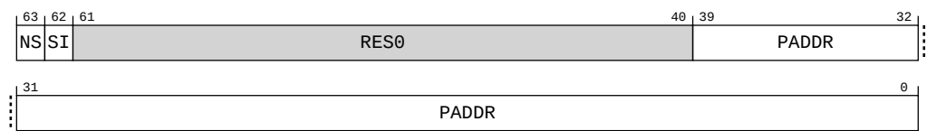
Figure B-225: ext_err0addr bit assignments
