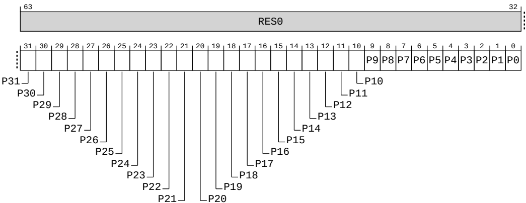
Figure A-157: AArch64_icv_ap1r0_el1 bit assignments
