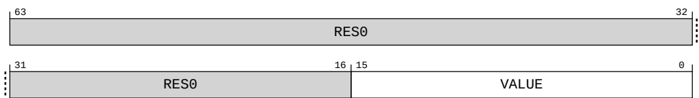
Figure A-190: AArch64_trccntrldvr1 bit assignments
