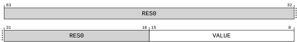
Figure A-199: AArch64_trcncntvr0 bit assignments
