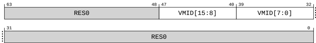
Figure A-103: AArch64_dbgvr5_el1 bit assignments
