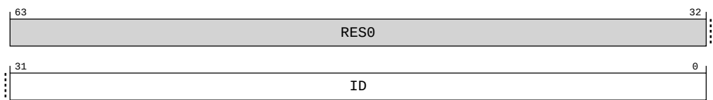
Figure A-117: AArch64_revidr_el1 bit assignments
