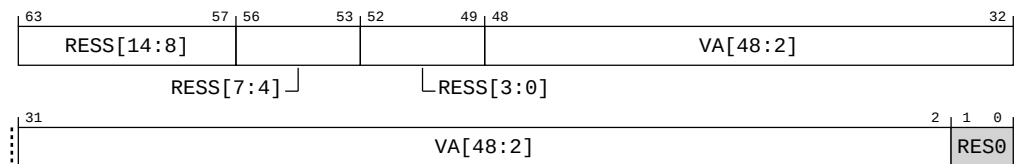
Figure A-62: AArch64_dbgvr1_el1 bit assignments
