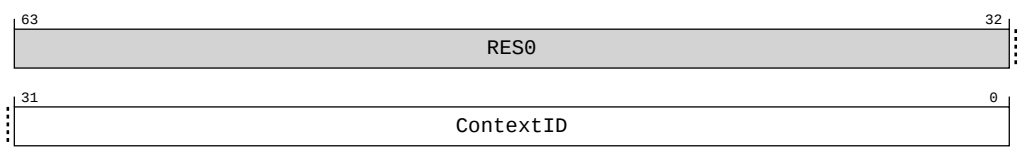
Figure B-114: ext_dbgivr4_el1 bit assignments
