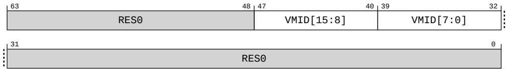
Figure B-84: ext_dbgivr0_el1 bit assignments
