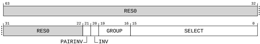
Figure A-215: AArch64_trcrsctlr6 bit assignments
