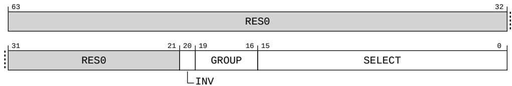
Figure A-216: AArch64_trcrsctlr7 bit assignments
