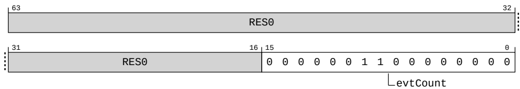
Figure A-181: AArch64_amevtyper10_el0 bit assignments
