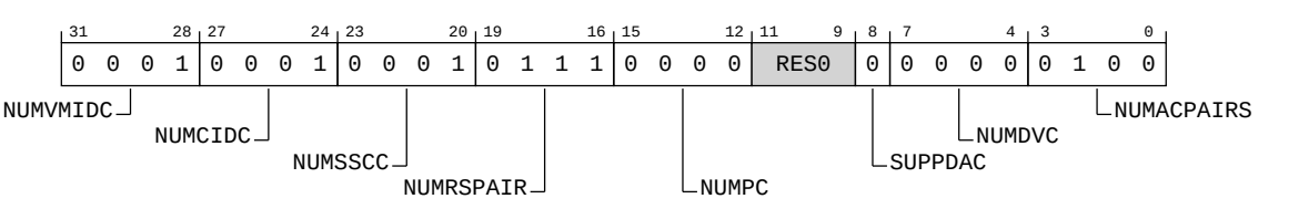
Figure B-197: ext_trcidr4 bit assignments
