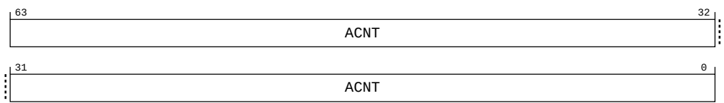
Figure A-178: AArch64_amevcntr10_el0 bit assignments
