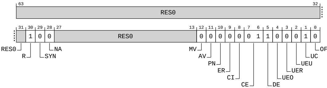
Figure A-253: AArch64_erxpfgf_el1 bit assignments
