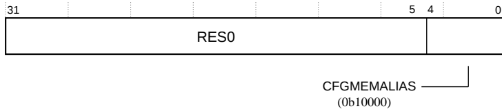
Figure 5-28: CFGINFORD bit assignments showing CFGMEMALIAS
