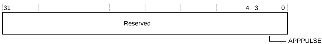
Figure 20-6: CTI_APPPULSE bit assignments
