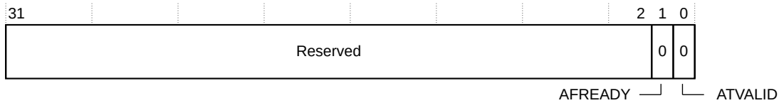
Figure 18-3: ITM_ITWRITE bit assignments
