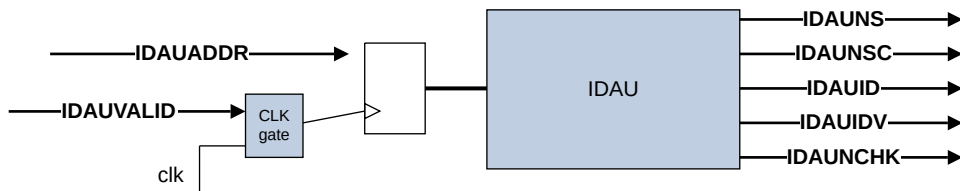
Figure 9-1: Cortex®-M55 IDAU interface backward compatibility
