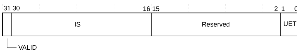
Figure 11-10: RFSR bit assignments
