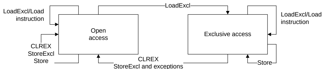
Figure 10-2: Operation of internal exclusive access monitor
