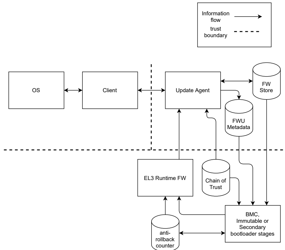
Figure D1.1: System diagram of the Secure World controlled NV storage model
