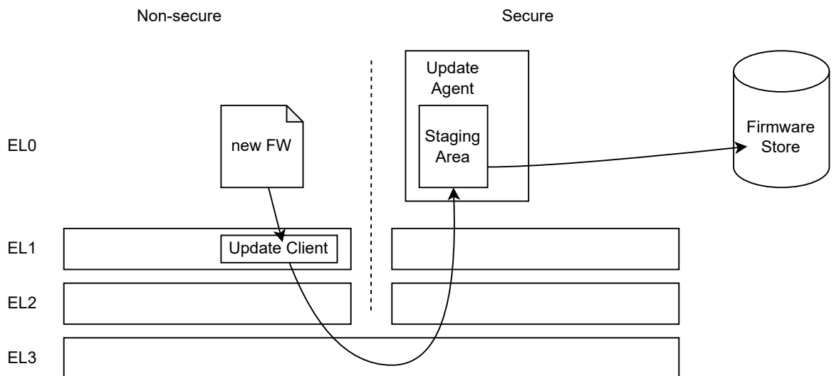
Figure 2.1: Firmware Store update system diagram
