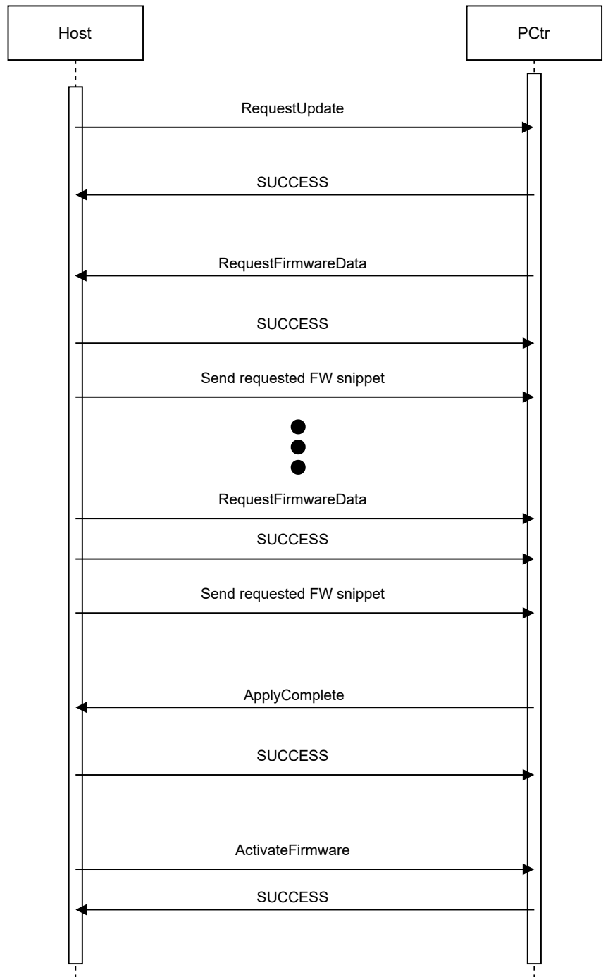
Figure B4.1: Information exchange between the AP and the PCtr during an image update
