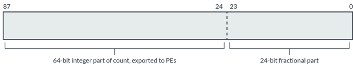
Figure 5-2: bit integer part of count image
