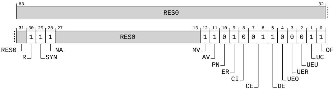
Figure A-146: AArch64_erxpfgf_el1 bit assignments
