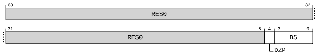
Figure A-134: AArch64_dczip_el0 bit assignments
