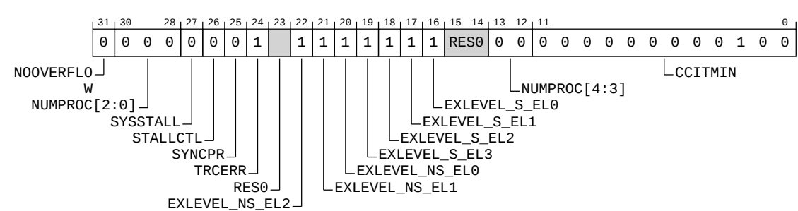
Figure B-126: ext_trcidr3 bit assignments
