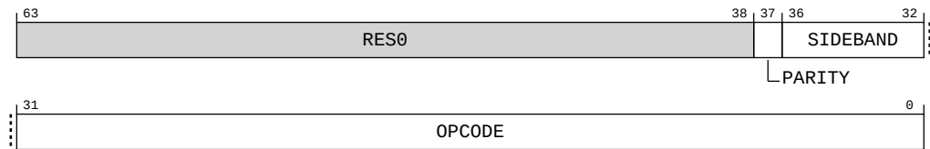
Figure A-39: AArch64_imp_iside_data0_el3 bit assignments
