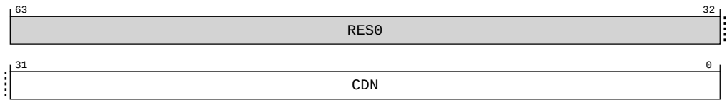
Figure B-79: ext_err0pfgcdn bit assignments
