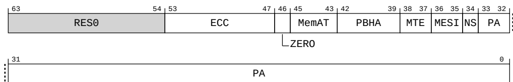
Figure A-61: AArch64_imp_l2_data0_el3 bit assignments
