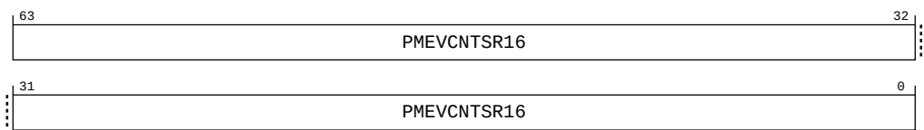
Figure B-25: ext_pmevcntr16 bit assignments
