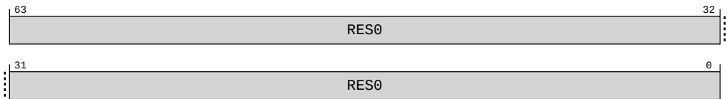
Figure A-165: AArch64_trcidr10 bit assignments
