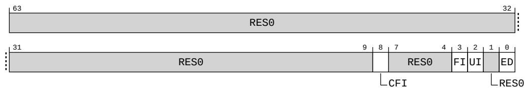
Figure A-143: AArch64_erxctlr_el1 bit assignments
