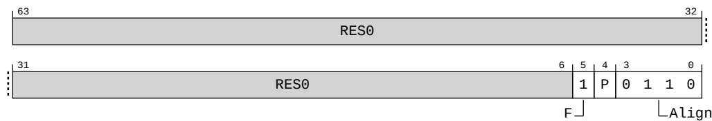
Figure A-138: AArch64_pmbidr_el1 bit assignments
