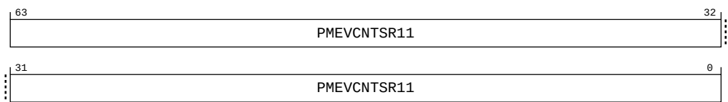
Figure B-20: ext_pmevcntr11 bit assignments
