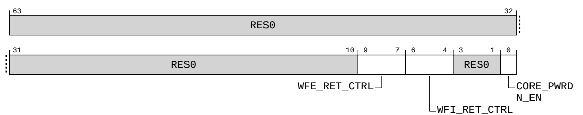
Figure A-14: AArch64_imp_cpupwrctlr_el1 bit assignments
