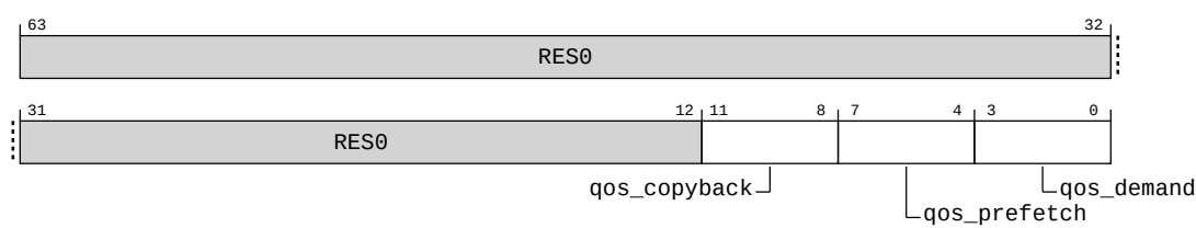
Figure A-13: AArch64_imp_cpubusqos_el1 bit assignments
