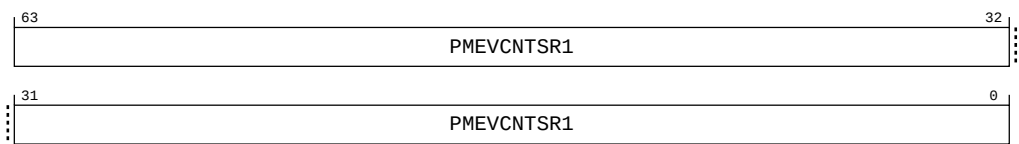
Figure B-10: ext_pmevcntr1 bit assignments
