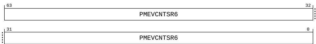
Figure B-15: ext_pmevcntrs6 bit assignments
