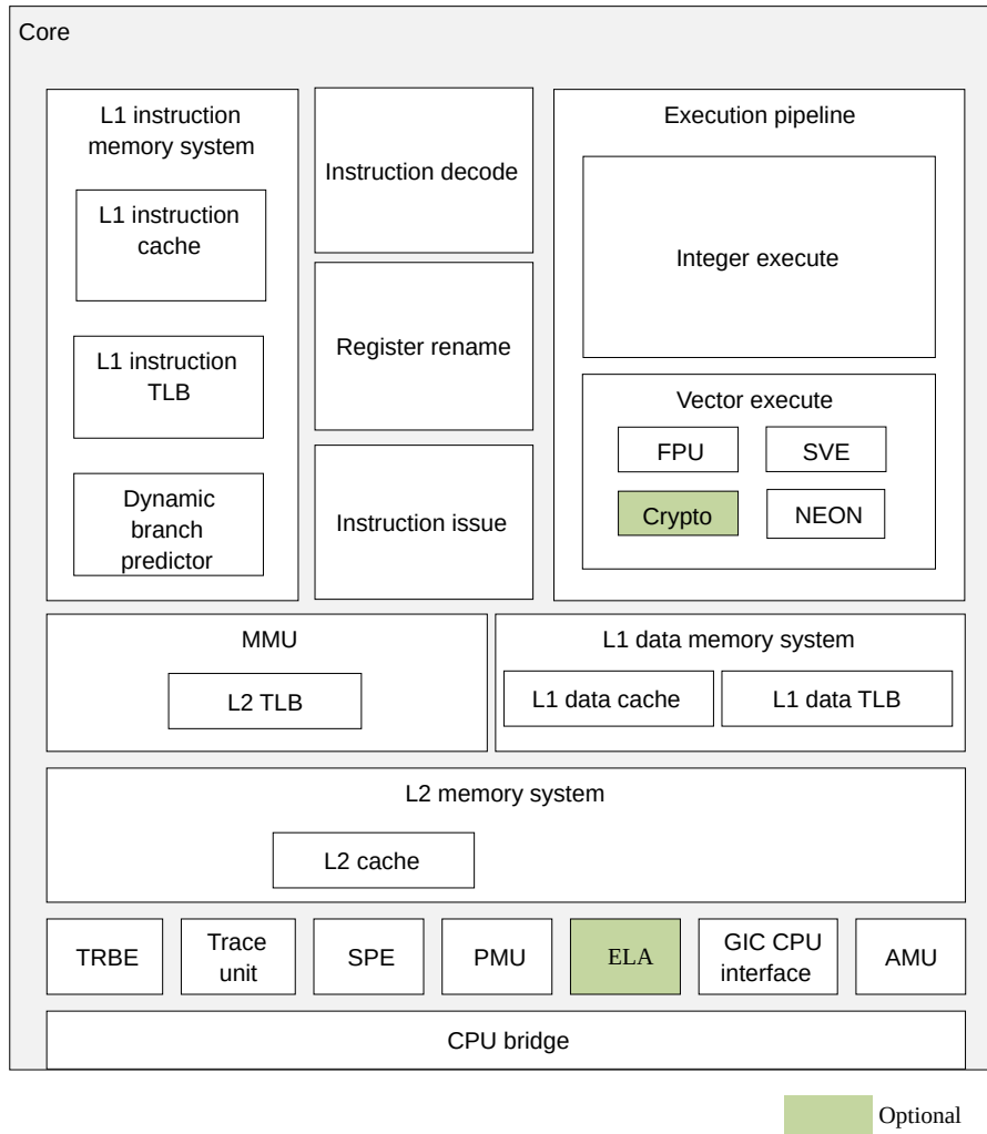
Figure 3-1: Neoverse™ N3 core components
