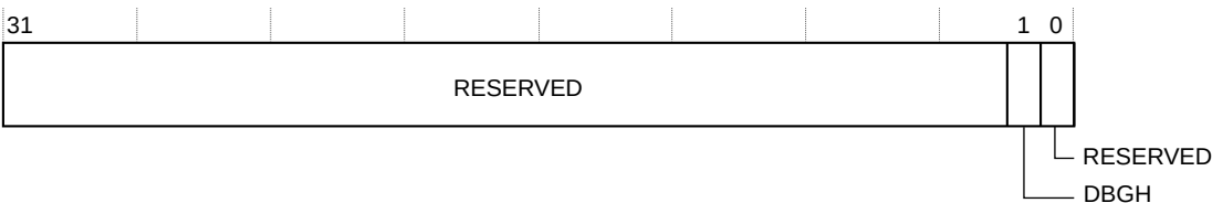
Figure 4-223: CNTSR bit assignments
