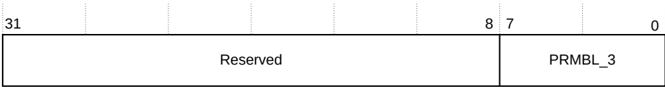
Figure 4-235: CIDR3 bit assignments
