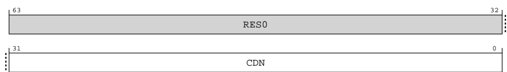
Figure A-252: AArch64_erpfgcdn_el1 bit assignments
