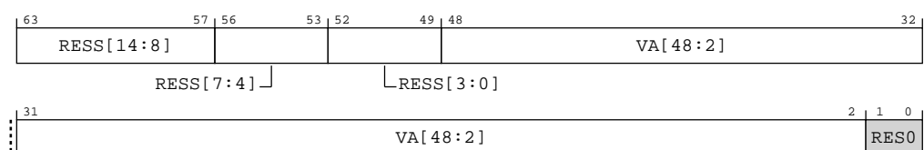
Figure B-89: ext_dbgbvr1_el1 bit assignments
