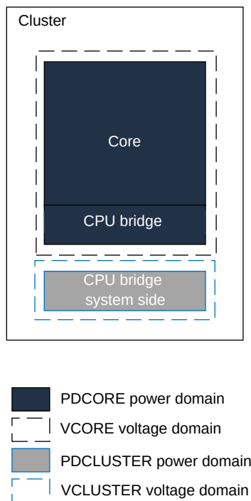
Figure 5-1: Cortex-X4 core voltage domains and power domains
