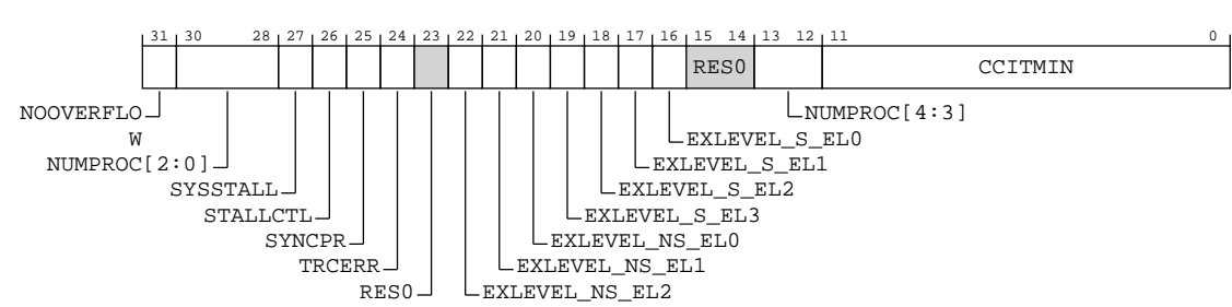
Figure B-196: ext_trcidr3 bit assignments
