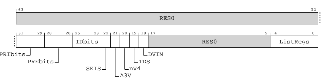
Figure A-160: AArch64_ich_vtr_el2 bit assignments
