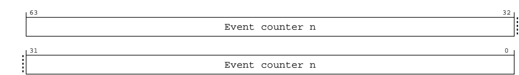
Figure A-144: AArch64_pmevcntr4_el0 bit assignments
