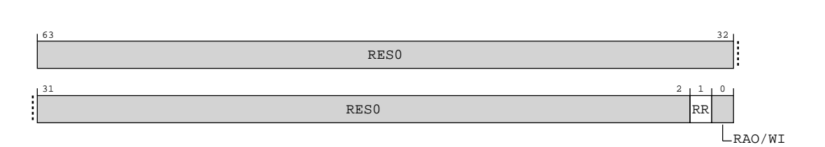
Figure A-33: AArch64_rmr_el3 bit assignments
