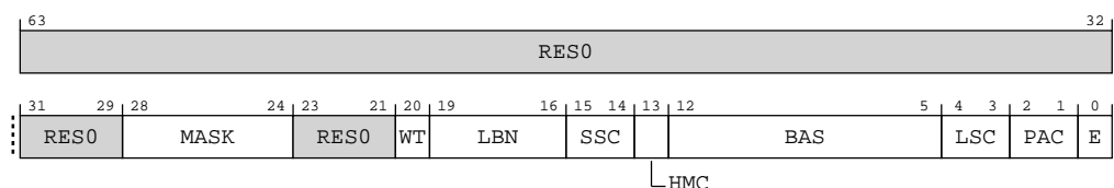
Figure A-79: AArch64_dbgwcr2_el1 bit assignments
