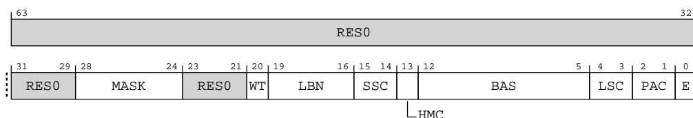
Figure A-89: AArch64_dbgwcr3_el1 bit assignments
