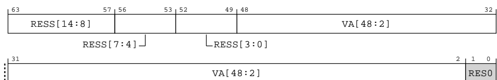
Figure A-98: AArch64_dbgvr5_el1 bit assignments
