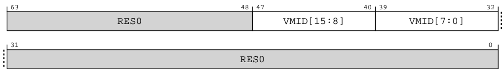
Figure A-83: AArch64_dbgvr3_el1 bit assignments
