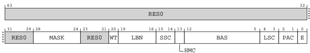
Figure A-59: AArch64_dbgwcr0_el1 bit assignments
