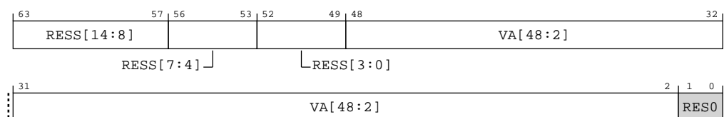
Figure A-50: AArch64_dbgbcvr0_el1 bit assignments
