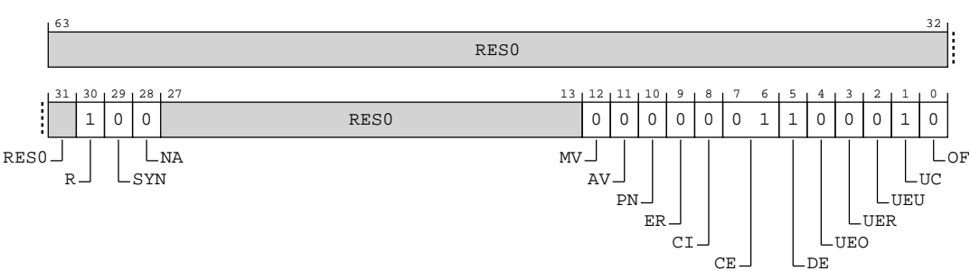
Figure B-240: ext_err1pfgf bit assignments
