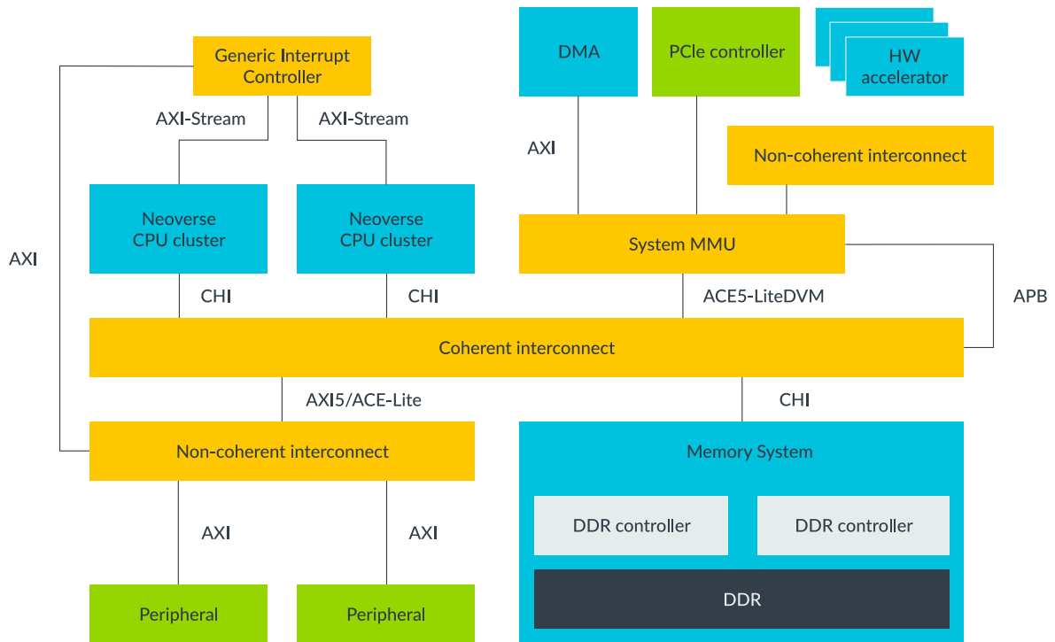
Figure 2-1: System diagram
