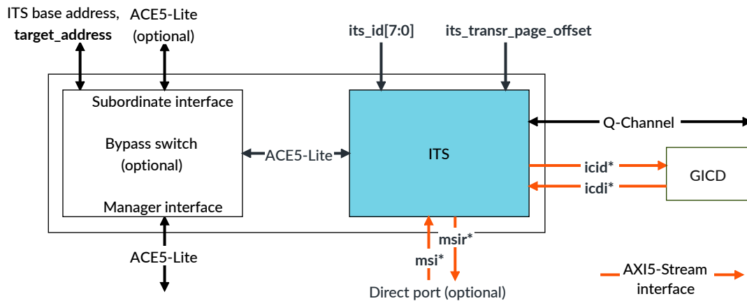
Figure 3-3: ITS block
