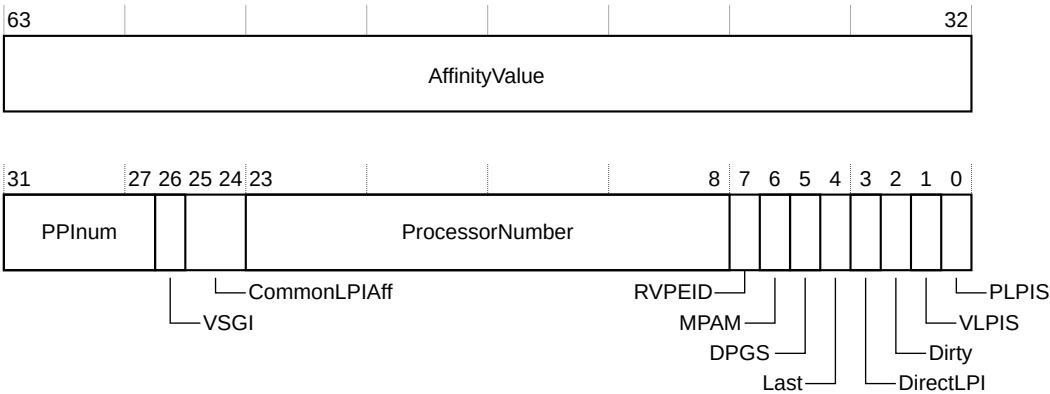
Figure 5-37: GICR_TYPER bit assignments
