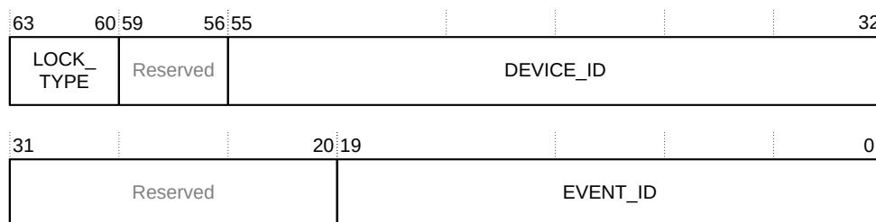
Figure 5-63: GITS_OPR bit assignments
