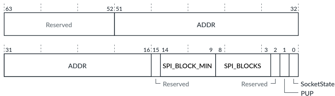
Figure 5-15: GICD_CHIPR<n> bit assignments
