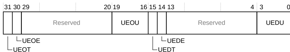
Figure 5-10: GICD_UTILR bit assignments
