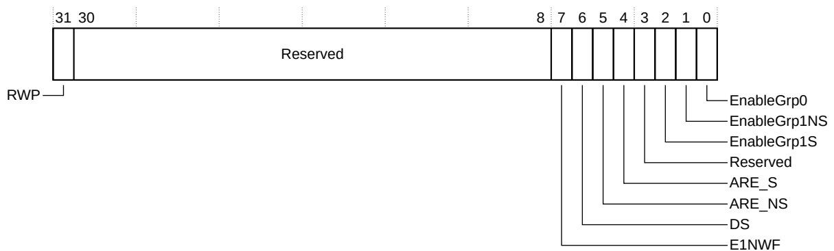
Figure 5-1: GICD_CTLR bit assignments
