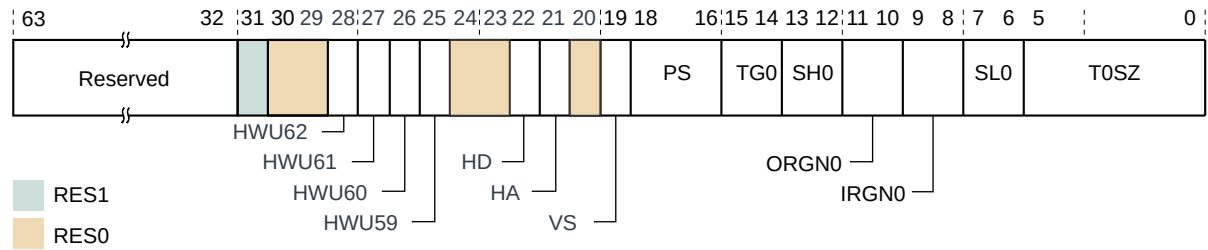
Figure 13-91: VTCR_EL2 bit assignments
