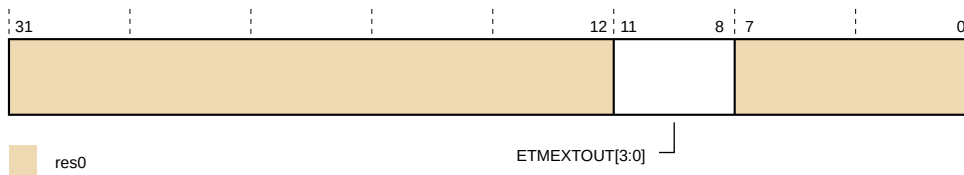
Figure 31-45: TRCITMISCOUT bit assignments
