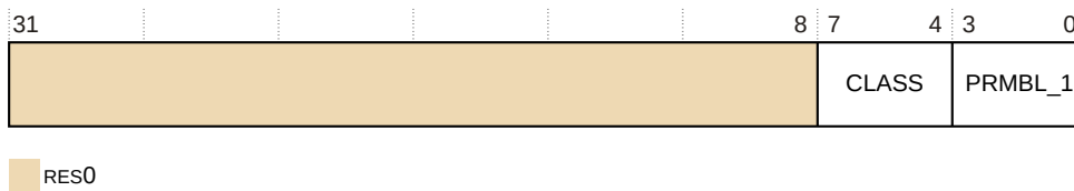
Figure 27-3: PMCIDR1 bit assignments
