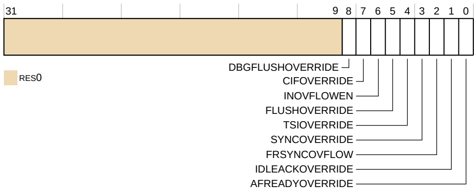
Figure 31-4: TRCAUXCTRL bit assignments
