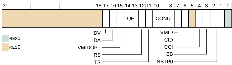
Figure 31-19: TRCCONFIGR bit assignments
