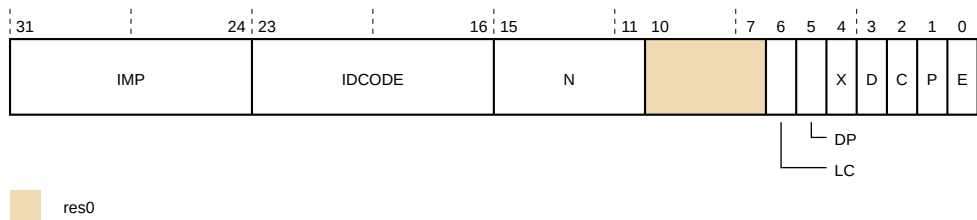
Figure 25-4: PMCR bit assignments
