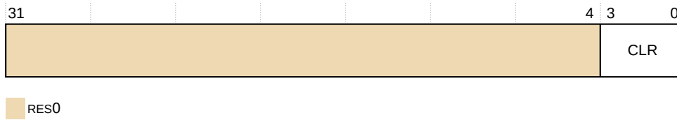
Figure 31-13: TRCCLAIMCLR bit assignments
