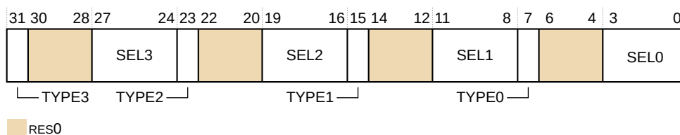
Figure 31-23: TRCEVENTCTL0R bit assignments
