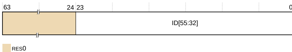
Figure 26-2: PMCEID1 bit assignments
