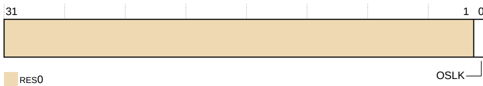
Figure 31-48: TRCOSLAR bit assignments
