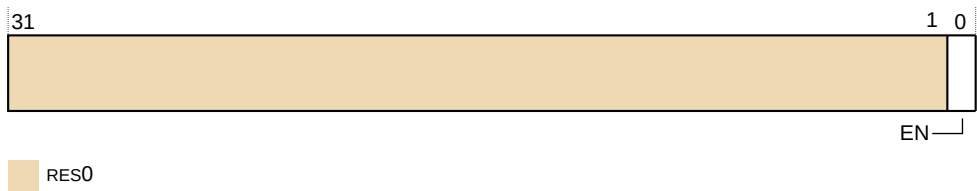
Figure 29-4: AMUSERENR_ELO bit assignments
