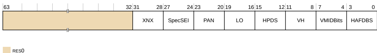
Figure 13-48: ID_AA64MMFR1_EL1 bit assignments
