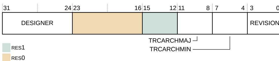
Figure 31-27: TRCIDR1 bit assignments
