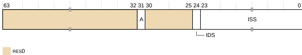
Figure 13-89: VDISR_EL2 at EL1 using AArch64
