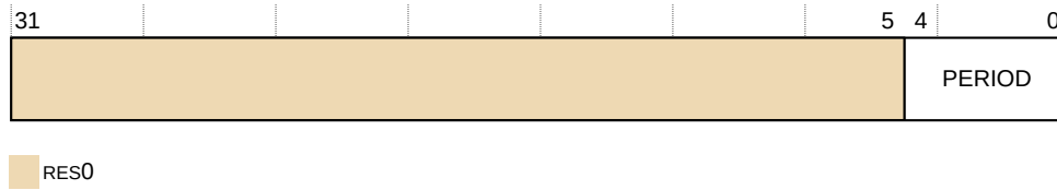
Figure 31-65: TRCSYNCPR bit assignments
