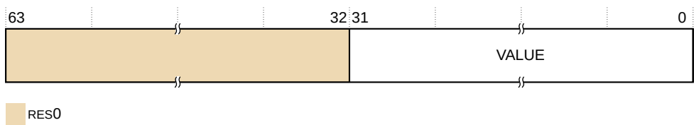
Figure 31-71: TRCVMIDCVR0 bit assignments
