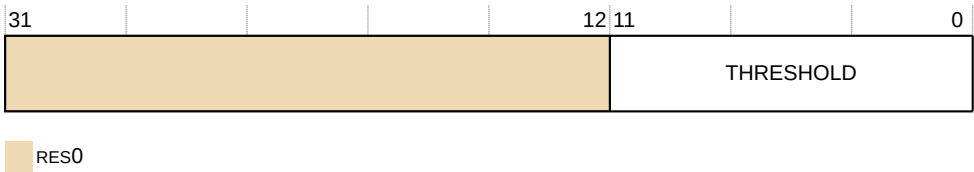
Figure 31-6: TRCCCCTLR bit assignments
