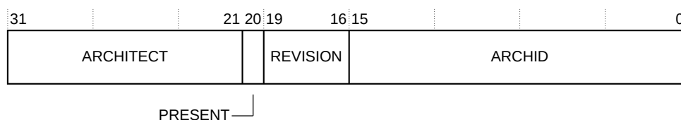
Figure 31-20: TRCDEVARCH bit assignments
