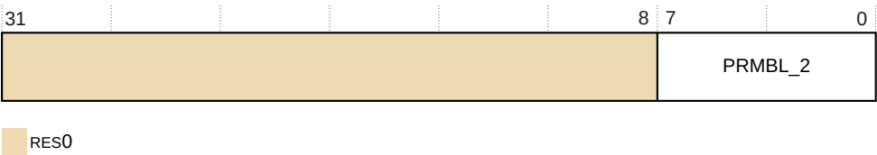
Figure 31-11: TRCCIDR2 bit assignments
