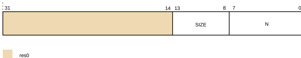
Figure 29-3: AMCFGR_EL0 bit assignments
