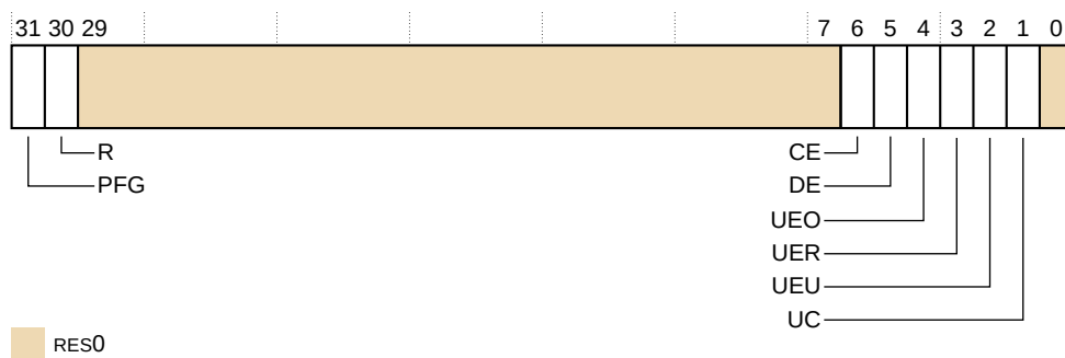
Figure 14-7: ERRORPFGF bit assignments
