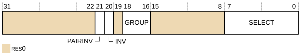
Figure 31-58: TRCRSCTLRn bit assignments
