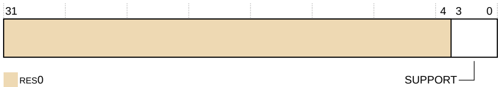
Figure 31-38: TRCIMSPECO bit assignments
