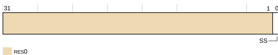
Figure 28-3: PMSSCR bit assignments
