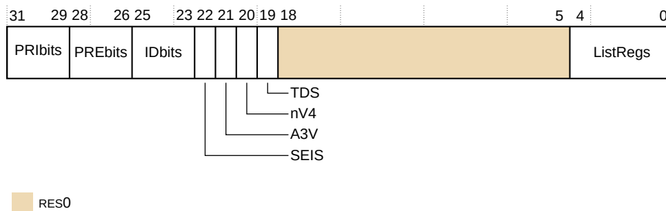
Figure 15-13: ICH_VTR_EL2 bit assignments
