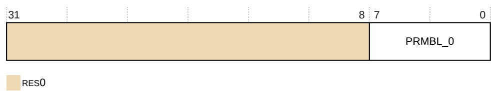
Figure 31-9: TRCCIDR0 bit assignments
