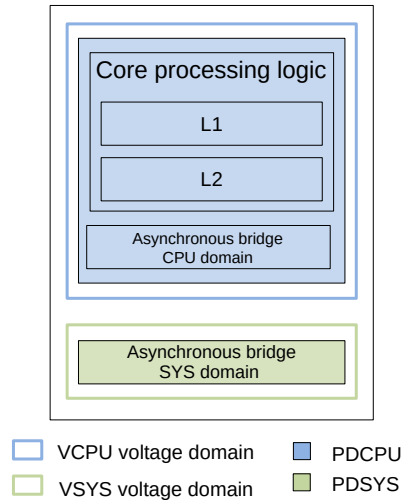
Figure 5-2: Neoverse™ N1 core power domain diagram at core processing logic level
