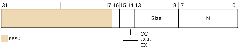
Figure 27-1: PMCFGR bit assignments
