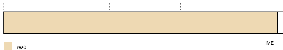
Figure 31-43: TRCITCTRL bit assignments
