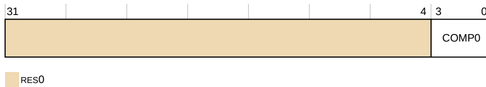
Figure 31-72: TRCVMIDCCTLRO bit assignments
