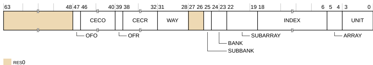
Figure 14-4: ERR0MISC0 bit assignments
