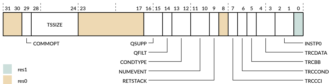
Figure 31-26: TRCIDR0 bit assignments
