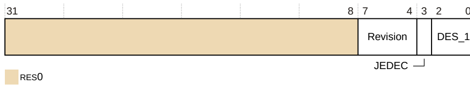
Figure 31-54: TRCPIDR2 bit assignments
