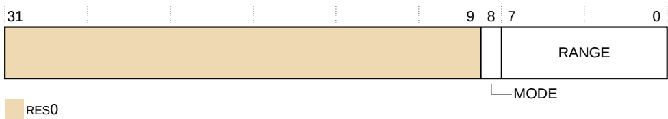
Figure 31-5: TRCBBCTLR bit assignments
