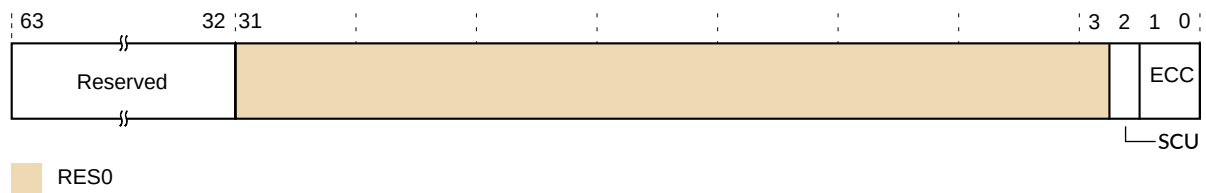
Figure 13-26: CPUCFR_EL1 bit assignments
