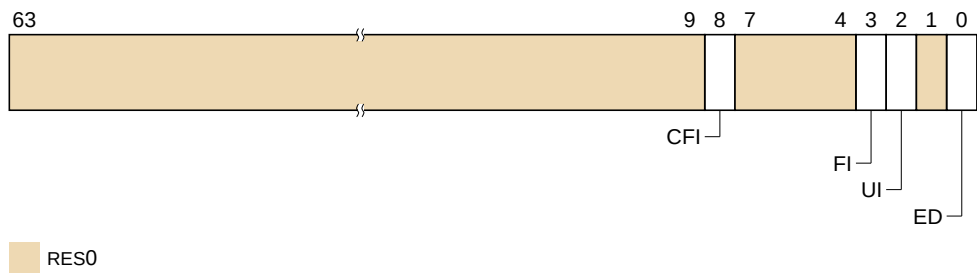
Figure 14-2: ERROCTLR bit assignments
