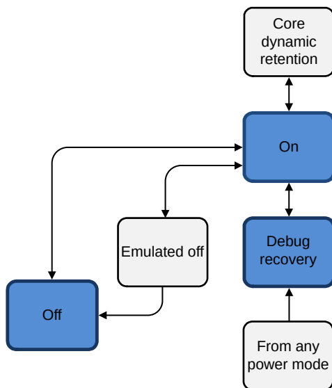
Figure 5-4: Neoverse™ N1 core power domain mode transitions
