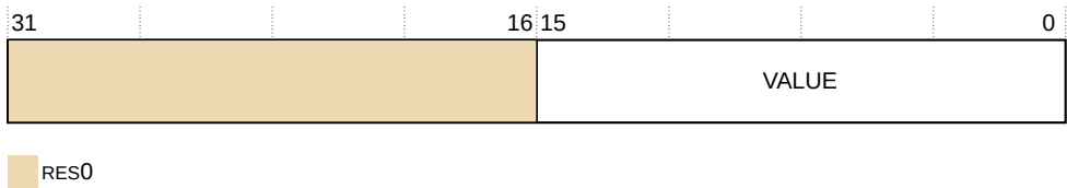
Figure 31-17: TRCCNTRLDVRn bit assignments
