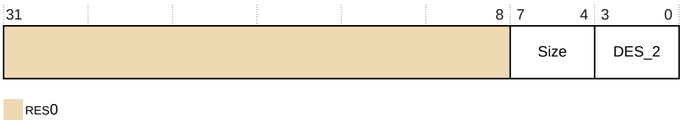
Figure 31-56: TRCPIDR4 bit assignments
