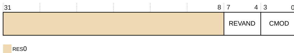
Figure 27-9: PMPIDR3 bit assignments
