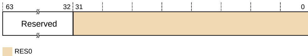
Figure 13-6: AFSR0_EL3 bit assignments
