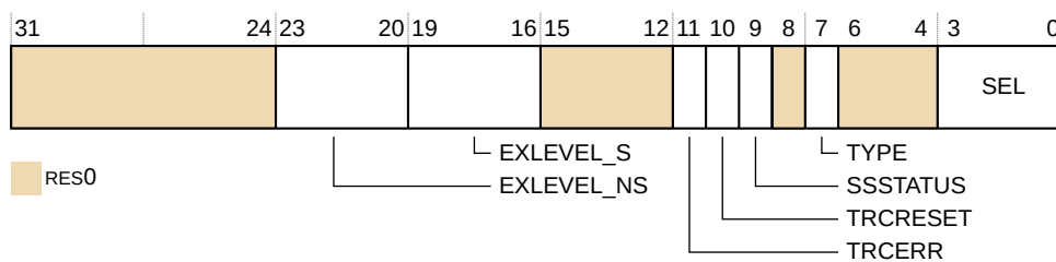
Figure 31-68: TRCVICTLR bit assignments
