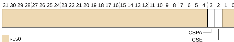
Figure 24-12: EDRCR bit assignments
