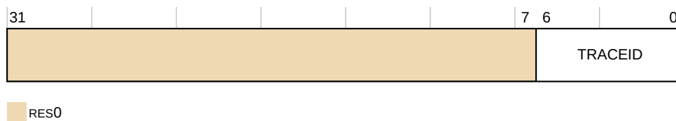
Figure 31-66: TRCTRACEIDR bit Assignments
