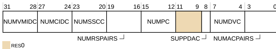
Figure 31-30: TRCIDR4 bit assignments
