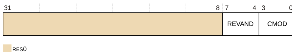
Figure 31-55: TRCPIDR3 bit assignments
