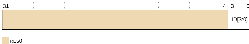
Figure 25-3: PMCEID2 bit assignments
