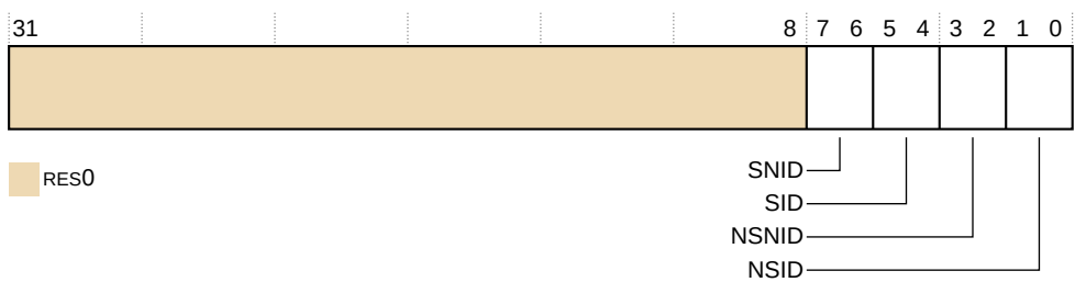
Figure 31-3: TRCAUTHSTATUS bit assignments
