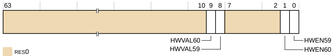
Figure 13-17: AVTCCR_EL2 bit assignments
