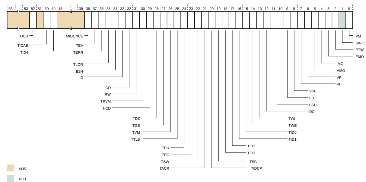
Figure 13-43: HCR_EL2 bit assignments
