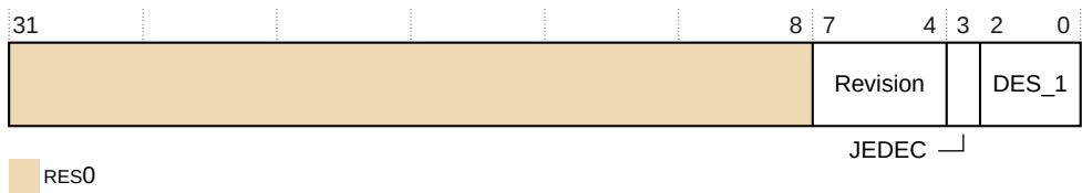
Figure 24-9: EDPIDR2 bit assignments
