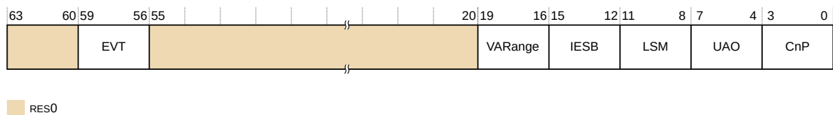
Figure 13-49: ID_AA64MMFR2_EL1 bit assignments
