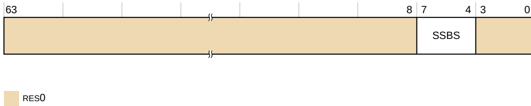
Figure 13-51: ID_AA64PFR1_EL1 bit assignments
