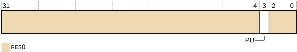
Figure 31-50: TRCPDCR bit assignments
