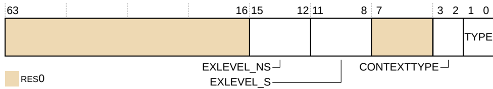
Figure 31-1: TRCACATRn bit assignments
