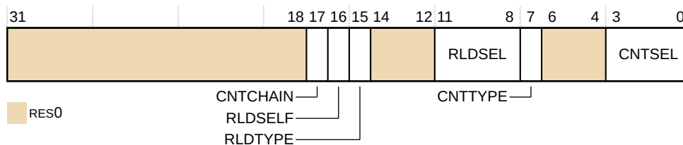
Figure 31-16: TRCCNTCTLR1 bit assignments
