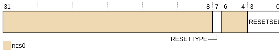
Figure 31-60: TRCSEQRSTEVr bit assignments
