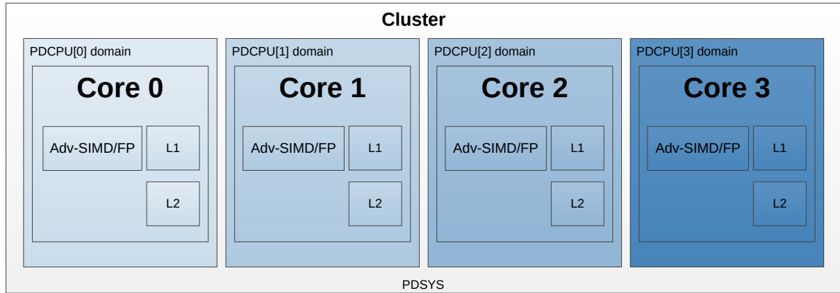
Figure 5-3: Neoverse™ N1 power domains at core processing logic level
