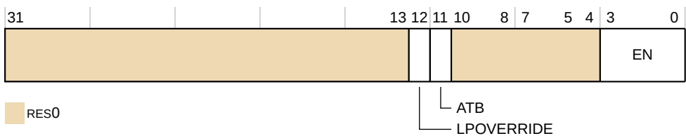
Figure 31-24: TRCEVENTCTL1R bit assignments
