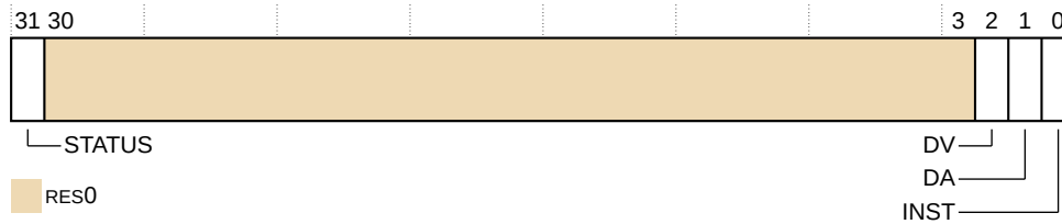
Figure 31-63: TRCSSCSR0 bit assignments
