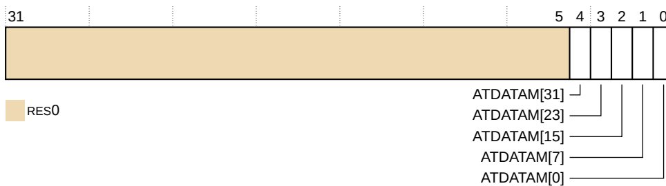
Figure 31-42: TRCITATBDATA0 bit assignments
