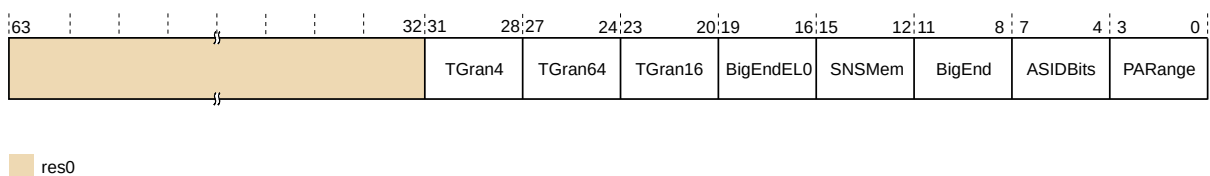
Figure 13-47: ID_AA64MMFR0_EL1 bit assignments
