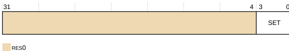
Figure 31-14: TRCCLAIMSET bit assignments
