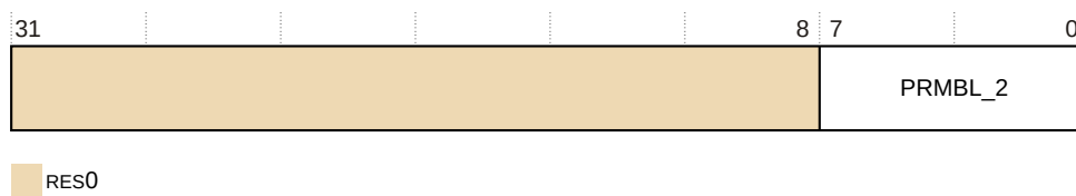
Figure 27-4: PMCIDR2 bit assignments
