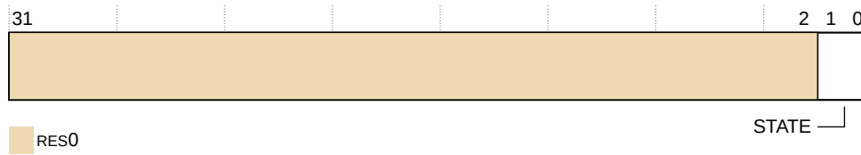
Figure 31-61: TRCSEQSTR bit assignments
