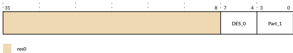
Figure 24-8: EDPIDR1 bit assignments
