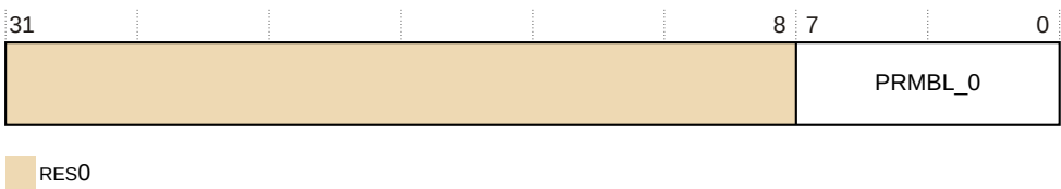
Figure 27-2: PMCIDR0 bit assignments
