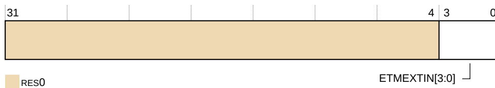
Figure 31-44: TRCITMISCIN bit assignments
