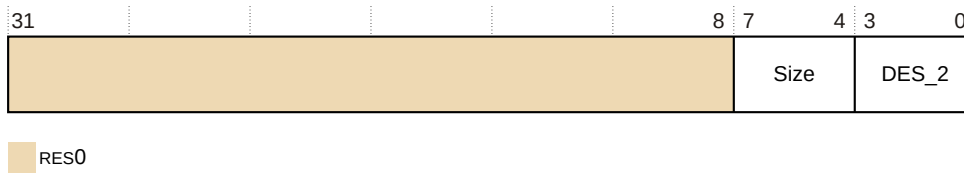
Figure 27-10: PMPIDR4 bit assignments
