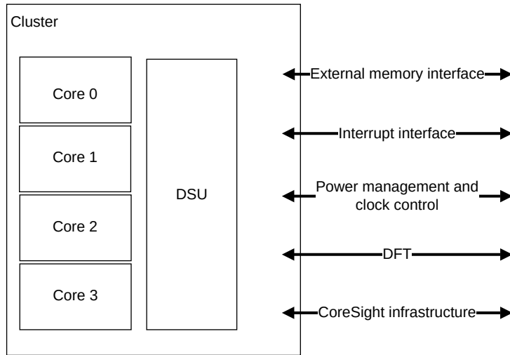
Figure 2-1: Example Neoverse™ N1 quad-core configuration
