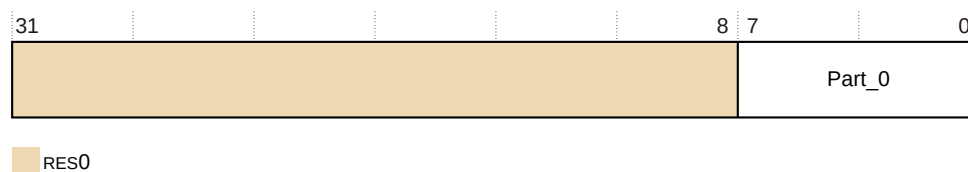
Figure 27-6: PMPIDR0 bit assignments
