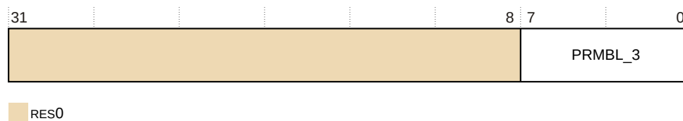
Figure 27-5: PMCIDR3 bit assignments
