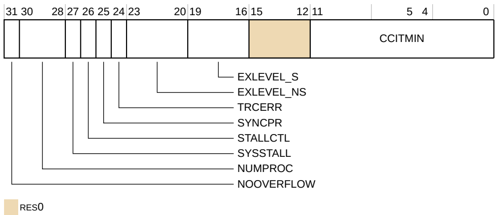
Figure 31-29: TRCIDR3 bit assignments
