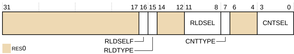
Figure 31-15: TRCCNTCTLR0 bit assignments
