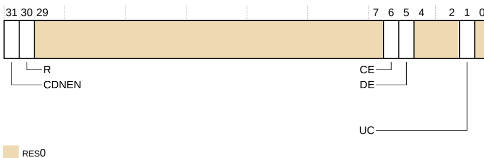
Figure 14-6: ERR0PFGCTL bit assignments
