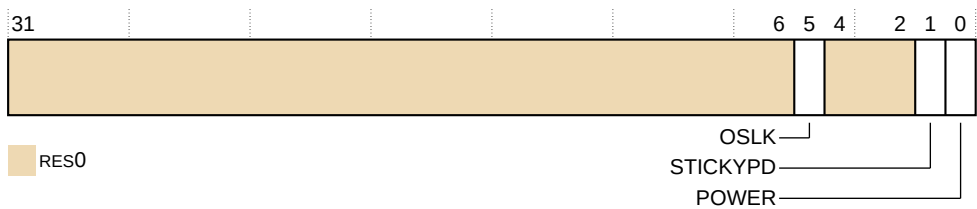
Figure 31-51: TRCPDSR bit assignments
