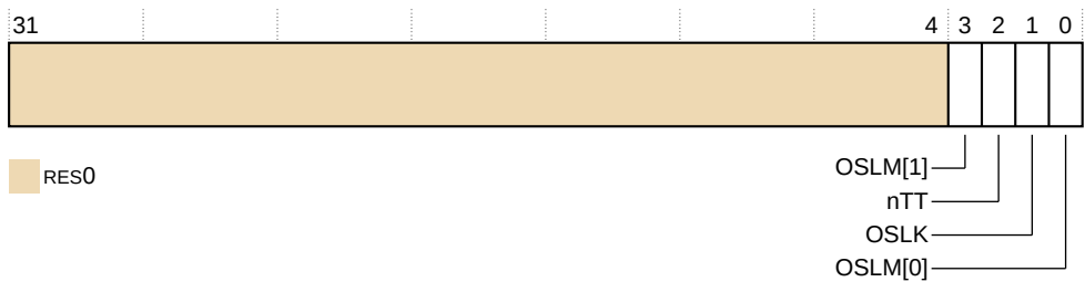
Figure 31-49: TRCOSLSR bit assignments
