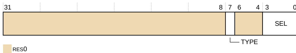
Figure 31-67: TRCTSCTLR bit assignments
