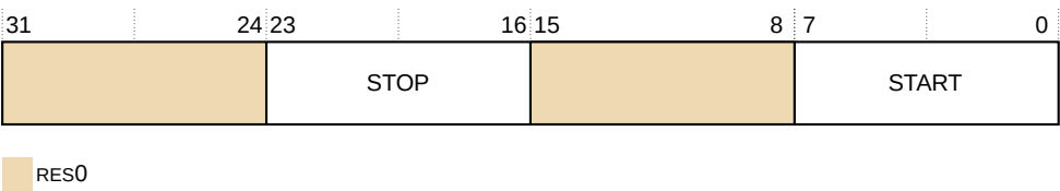
Figure 31-70: TRCVISSCTLR bit assignments
