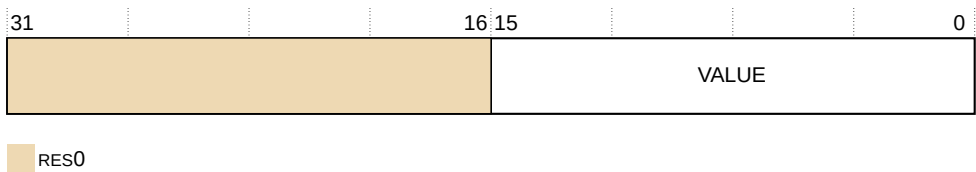
Figure 31-18: TRCCNTRn bit assignments
