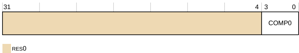
Figure 31-7: TRCCIDCCTLR0 bit assignments
