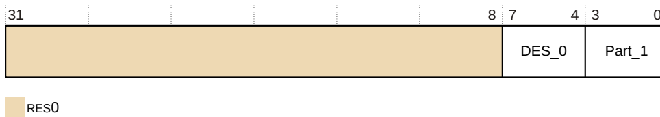
Figure 31-53: TRCPIDR1 bit assignments
