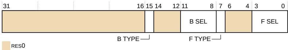
Figure 31-59: TRCSEQEVRn bit assignments
