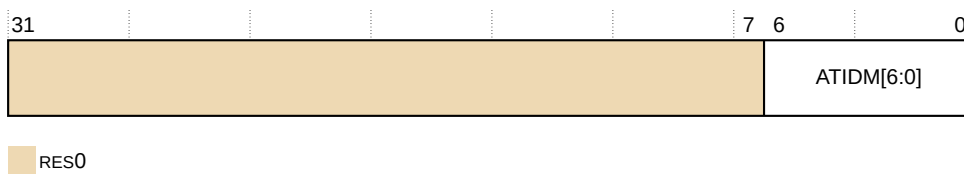
Figure 31-40: TRCITATBCTR1 bit assignments
