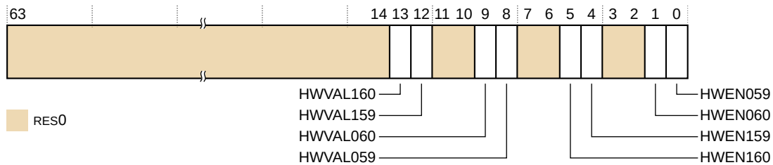
Figure 13-15: ATCR_EL2 bit assignments
