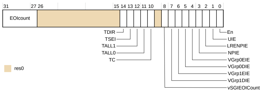
Figure 15-11: ICH_HCR_EL2 bit assignments
