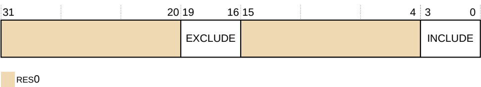
Figure 31-69: TRCVIIECTLR bit assignments
