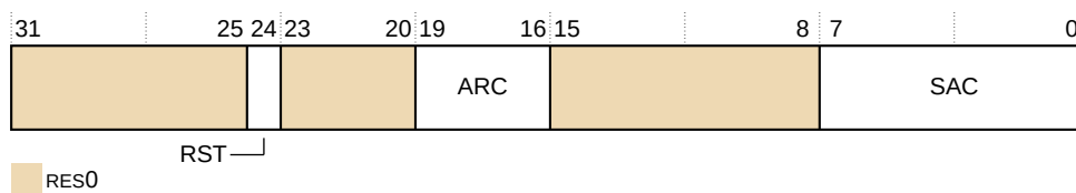
Figure 31-62: TRCSSCCR0 bit assignments
