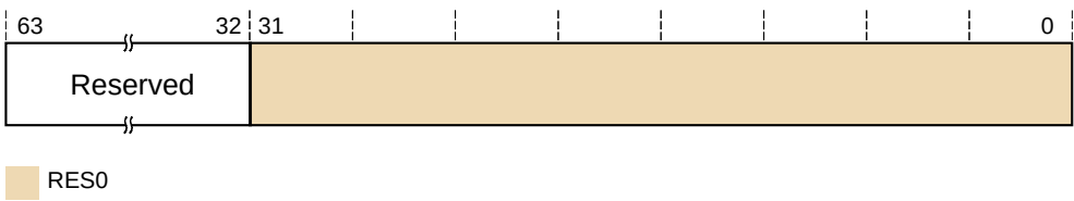
Figure 13-4: AFSRO_EL1 bit assignments
