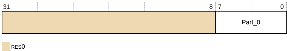
Figure 31-52: TRCPIDR0 bit assignments
