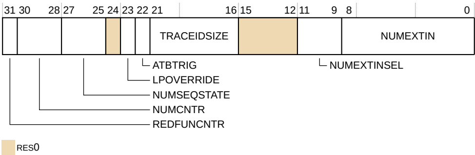
Figure 31-31: TRCIDR5 bit assignments
