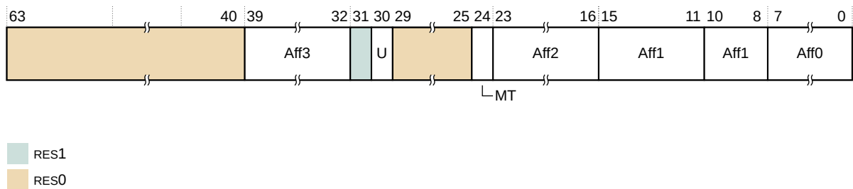
Figure 13-74: MPIDR_EL1 bit assignments
