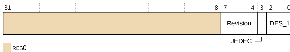
Figure 27-8: PMPIDR2 bit assignments
