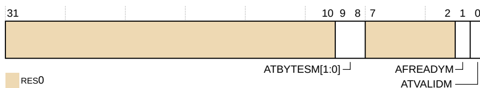
Figure 31-39: TRCITATBCTR0 bit assignments
