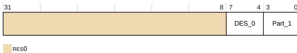
Figure 27-7: PMPIDR1 bit assignments
