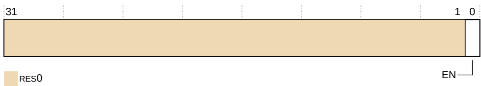
Figure 31-57: TRCPRGCTLR bit assignments
