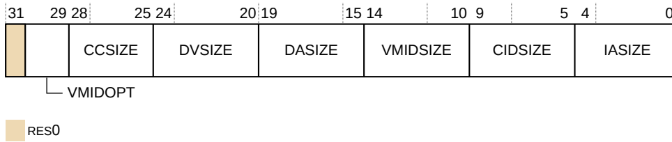
Figure 31-28: TRCIDR2 bit assignments
