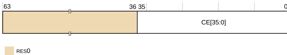
Figure 26-1: PMCEID0_ELO bit assignments
