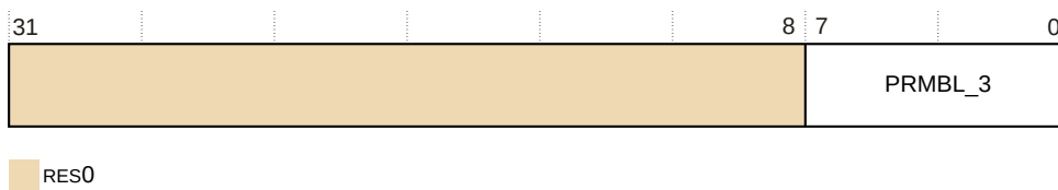
Figure 31-12: TRCCIDR3 bit assignments
