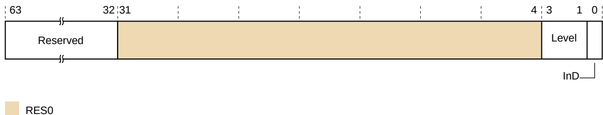
Figure 13-33: CSSELR_EL1 bit assignments
