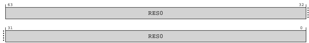
Figure A-150: AArch64_trcauxctlr bit assignments
