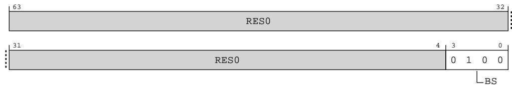
Figure A-103: AArch64_gmid_el1 bit assignments
