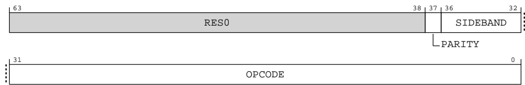
Figure A-31: AArch64_imp_iside_data0_el3 bit assignments
