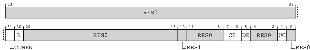
Figure A-128: AArch64_erxpfctl_el1 bit assignments
