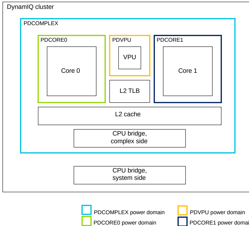
Figure 5-2: Cortex-A520 power domains, dual core
