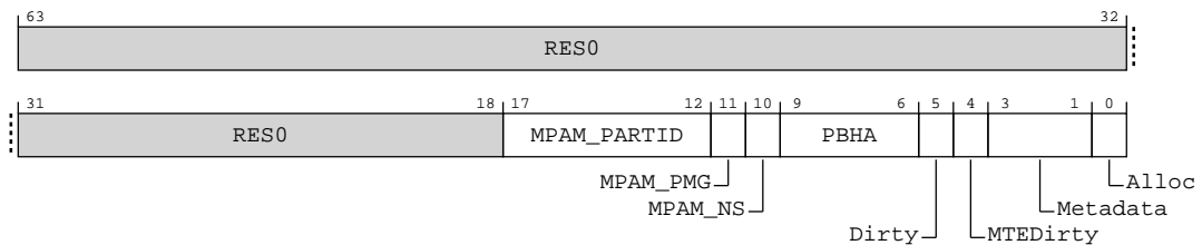
Figure A-34: AArch64_imp_cdbgdr0_el3 bit assignments
