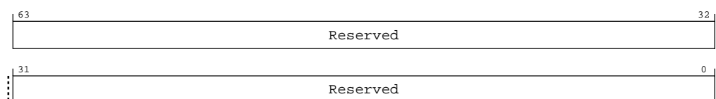
Figure A-10: AArch64_imp_cpuactlr3_el1 bit assignments
