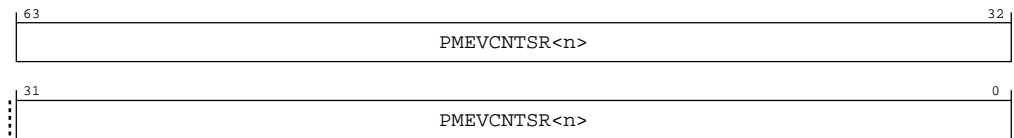
Figure B-54: ext_pmevcntrs0 bit assignments
