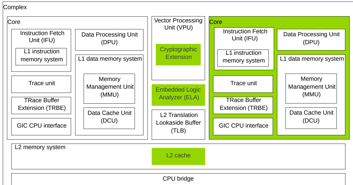
Figure 3-1: Cortex-A520 core components
