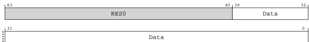
Figure A-32: AArch64_imp_cdbgdr0_el3 bit assignments
