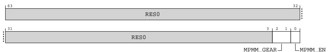
Figure A-98: AArch64_imp_cpumpmmcr_el3 bit assignments
