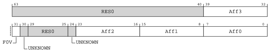
Figure B-14: complex_ras.errdevaff bit assignments
