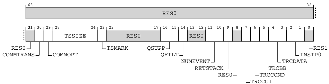
Figure A-130: AArch64_trcidr0 bit assignments
