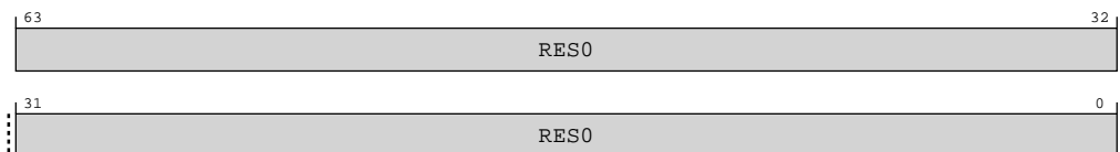
Figure A-18: AArch64_hacr_el2 bit assignments
