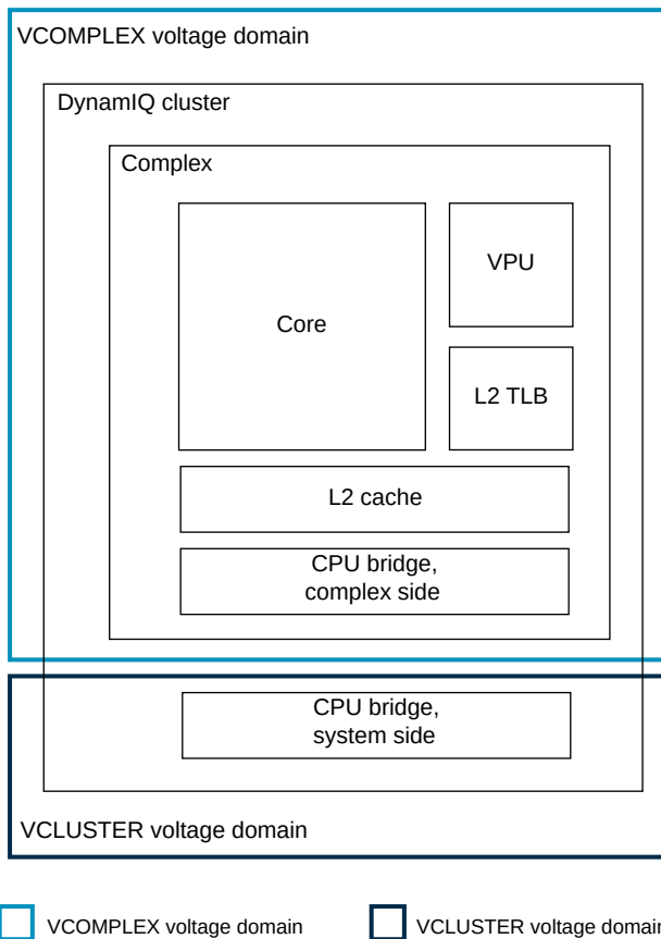
Figure 5-3: Cortex-A520 voltage domains, single core
