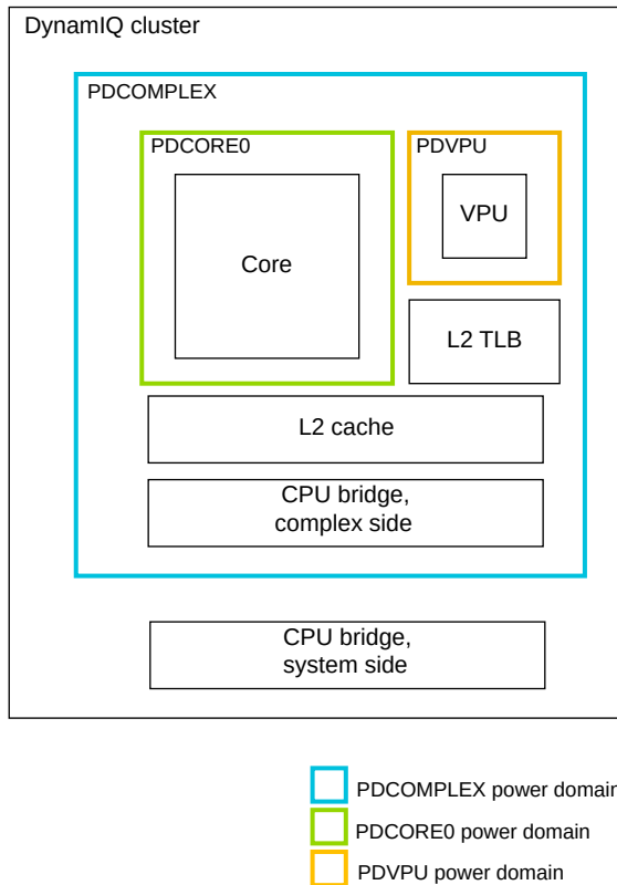
Figure 5-4: Cortex-A520 power domains, single core
