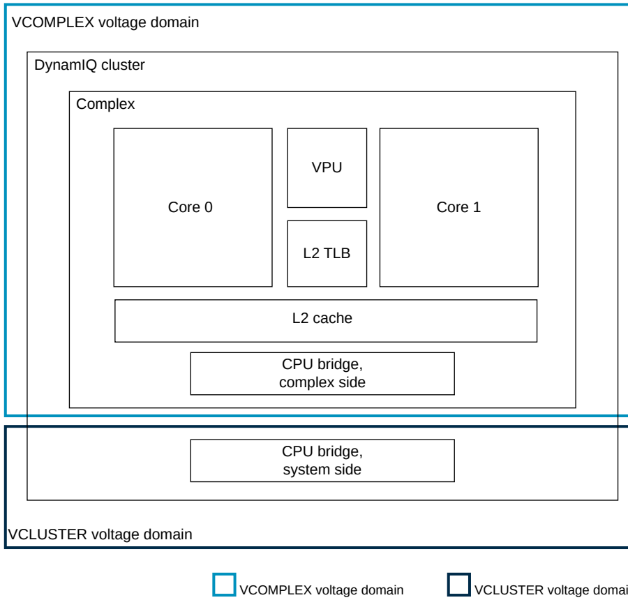
Figure 5-1: Cortex-A520 voltage domains, dual core
