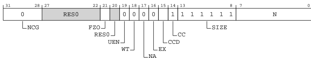
Figure B-74: ext_pmcfgr bit assignments
