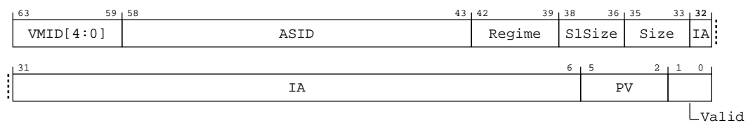
Figure A-37: AArch64_imp_cdbgdr0_el3 bit assignments
