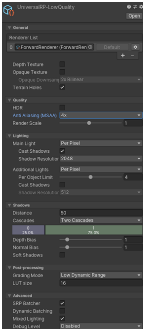
Figure 5-1: Screenshot of the URP settings window
