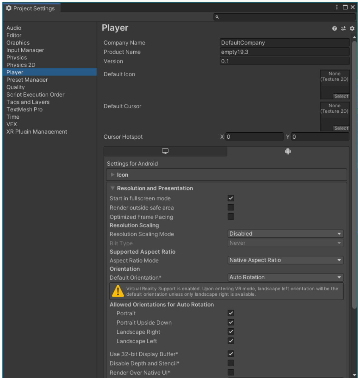
Figure 4-1: Screenshot of the player settings window
