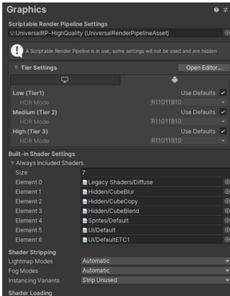
Figure 3-1: Screenshot of the graphics settings
