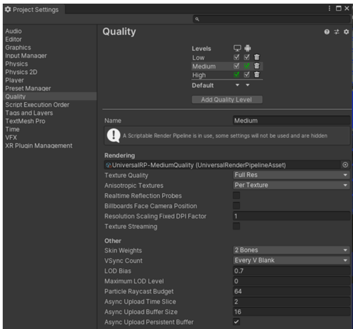
Figure 2-1: Project settings quality screenshot
