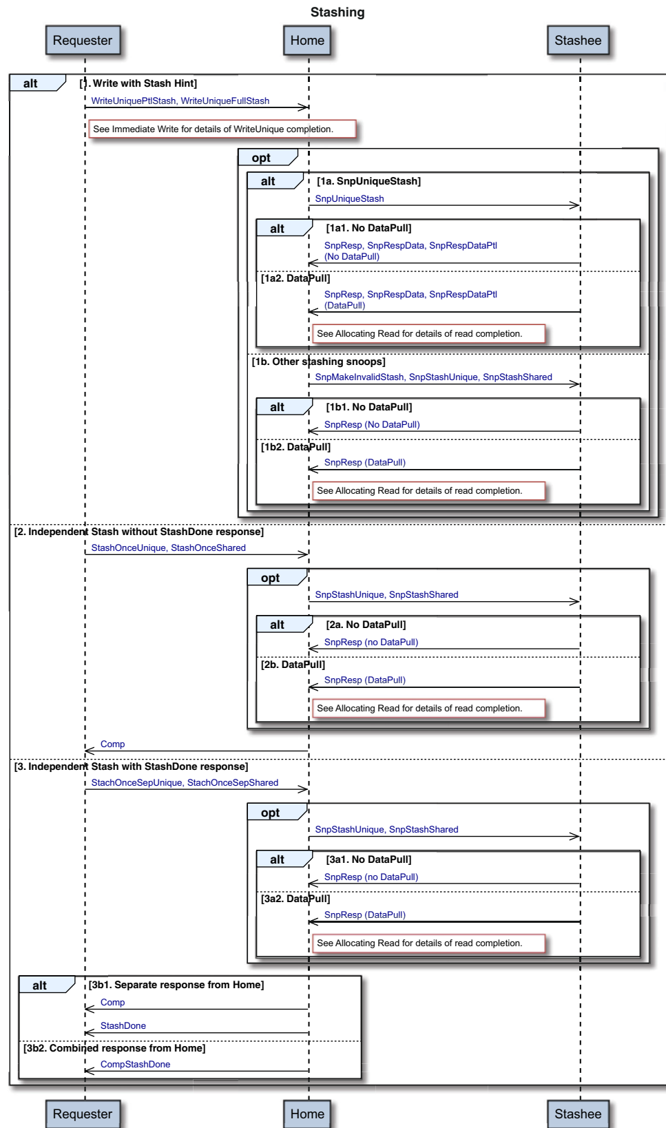
Figure 2-10 Stash transactions
