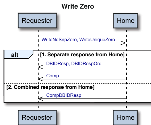
Figure 2-4 Write Zero
