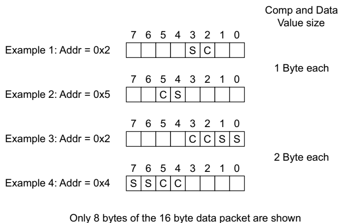
Figure 2-36 Data value packing for AtomicCompare transaction
