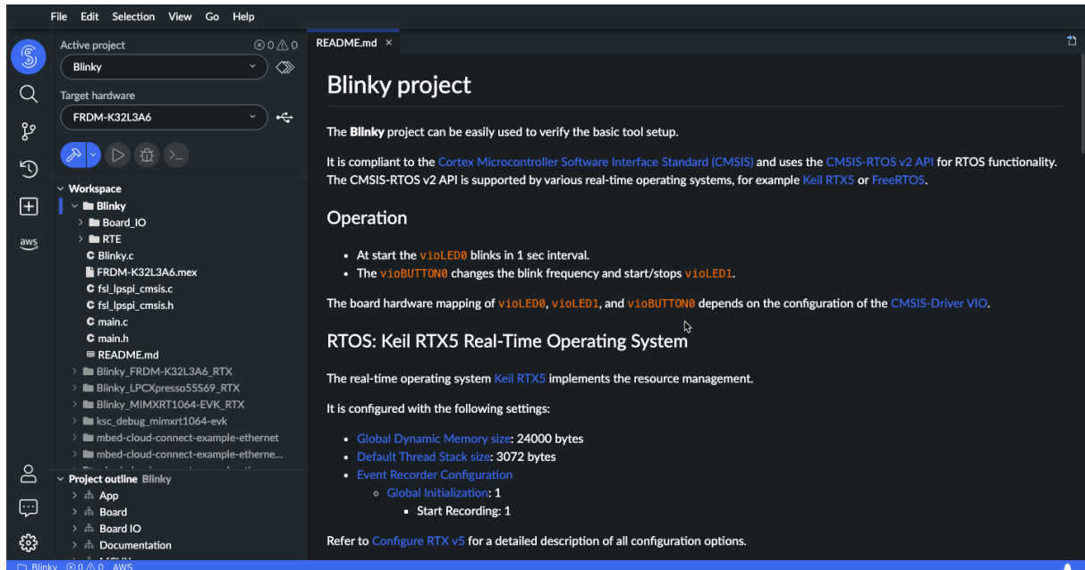
Figure 4-2: Open project showing README.md
