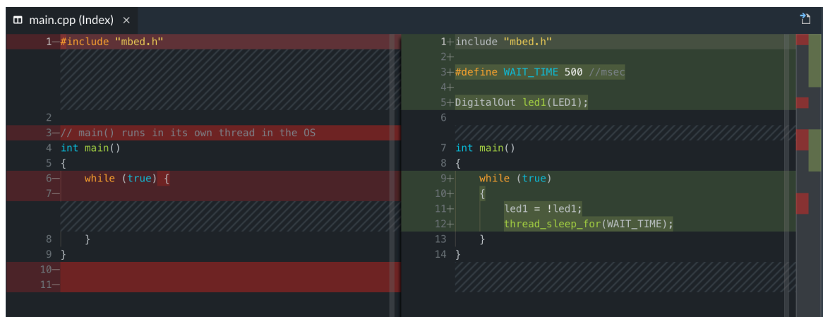
Figure 12-5: Double-click a file to view its side-by-side comparison
