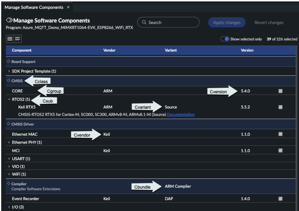
Figure 10-1: The ‘Manage Software Components’ view showing the components included in the active project
