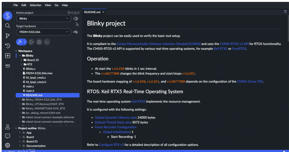
Figure 4-3: Manage software components
