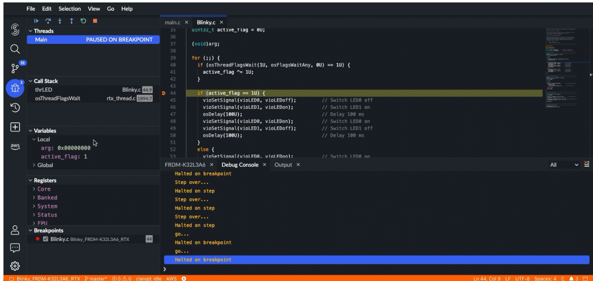
Figure 4-18: Examine the call stack
