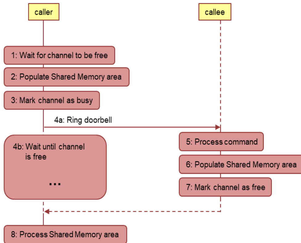
Figure 7: Polling based Communication Flow
