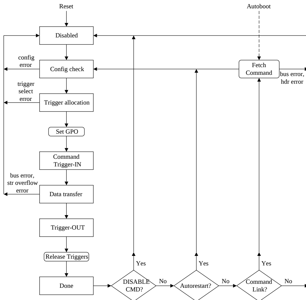
Figure 5-22: DMA channel states
