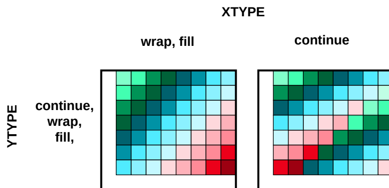
Figure 5-10: 2D wrap when SRCXSIZE > DESXSIZE and SRCYSIZE >= DESYSIZE
