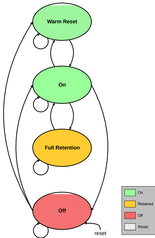
Figure 5-25: Supported power states and transitions
