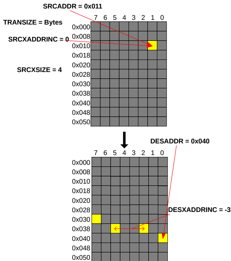
Figure 5-4: 1D transfer with zero and negative increments
