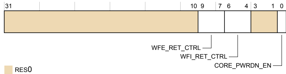
Figure B2-49 CPUPWRCTLR_EL1 bit assignments
