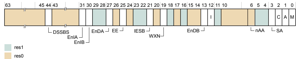
Figure B2-98 SCTL_EL3 bit assignments
