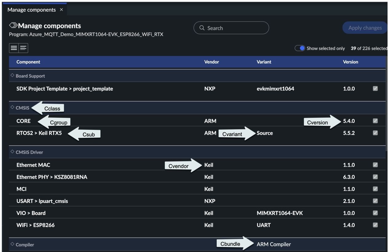
Figure 10-1: The 'Manage components' view showing the components included in the active project
