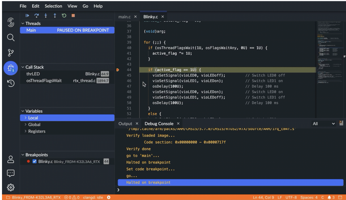
Figure 4-8: Check variables
