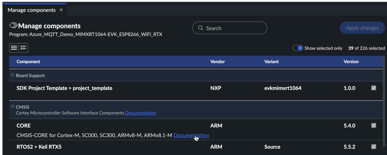
Figure 10-2: Documentation links in the 'Manage components' view
