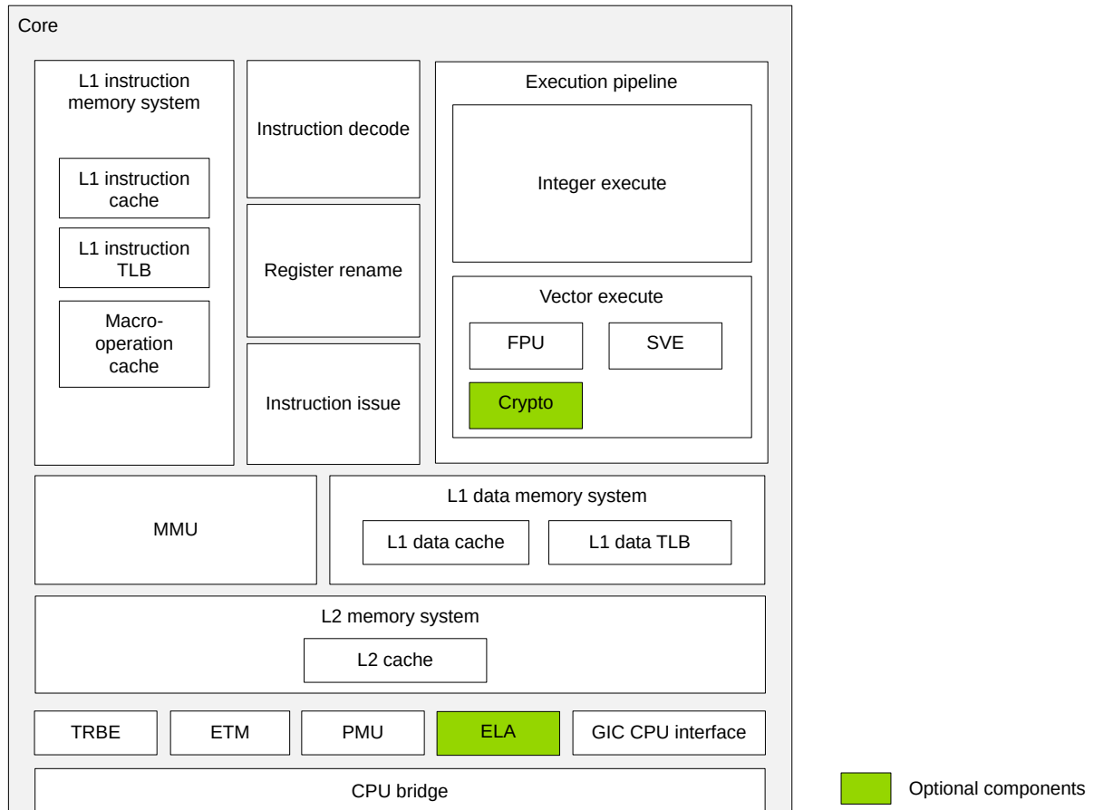
Figure 3-1: Cortex®-X2 core components
