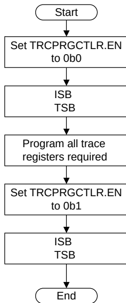
Figure 18-3: Programming ETM registers using the System register interface
