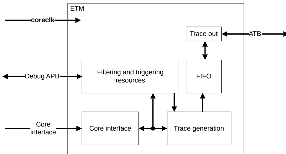
Figure 18-1: ETM components
