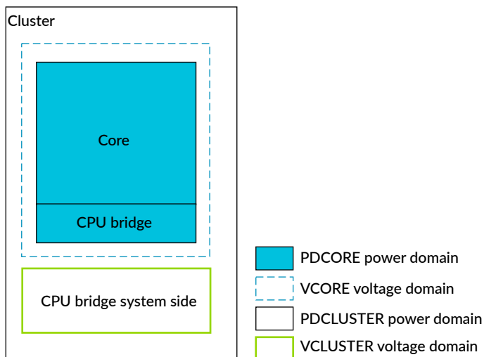
Figure 5-1: Cortex®-X2 core voltage domains and power domains
