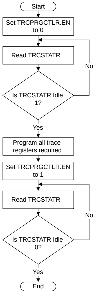
Figure 18-2: Programming ETM registers using the Debug APB interface
