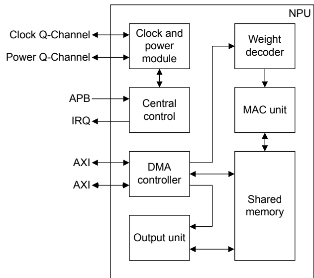
Figure 2-3 Functional blocks diagram
