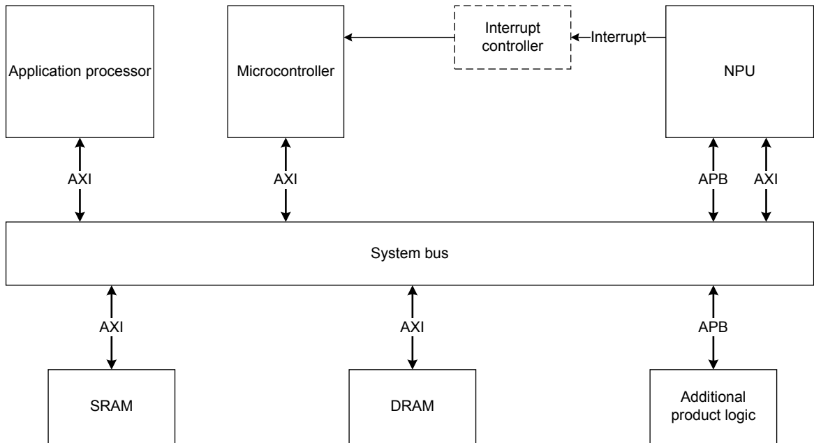
Figure 1-1 Typical system configuration block diagram
