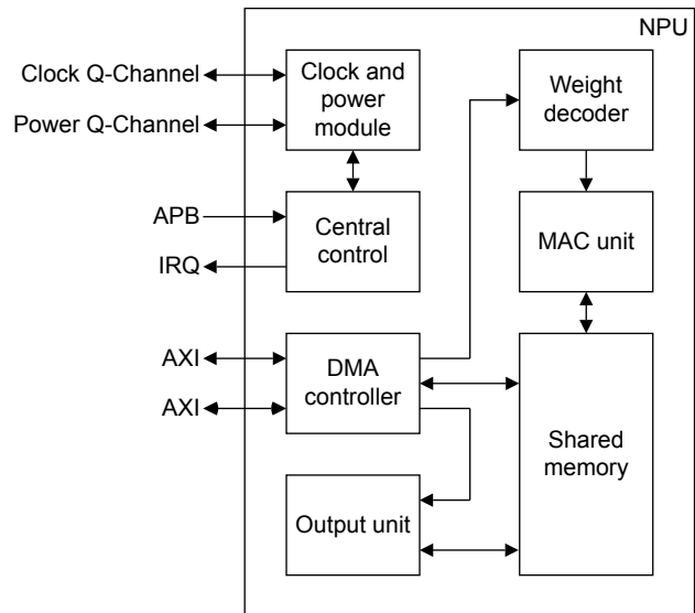
Figure 1-2 Functional blocks diagram
