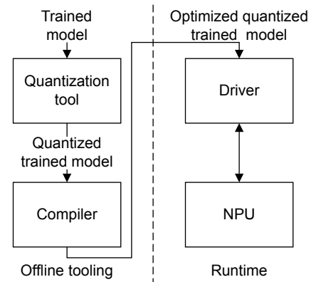
Figure 2-1 The software stack of the NPU
