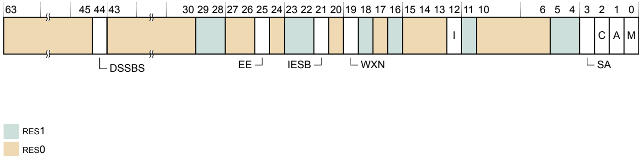
Figure B2-88 SCTLR_EL3 bit assignments
