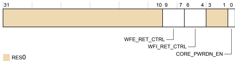
Figure B2-39 CPUPWRCTLR_EL1 bit assignments
