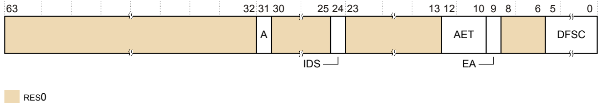
Figure B2-43 DISR_EL1 bit assignments, DISR_EL1.IDS is 0
