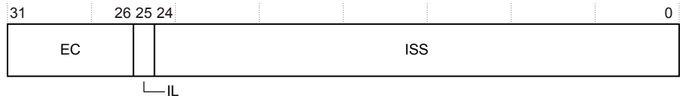
Figure B2-47 ESR_EL2 bit assignments
