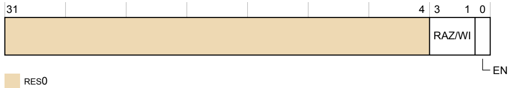
Figure D8-12 AMUSERENR_EL0 bit assignments
