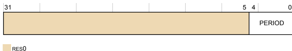
Figure D10-65 TRCSYNCP bit assignments
