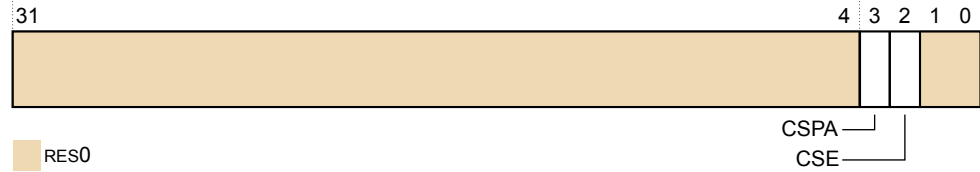
Figure D3-12 EDRCR bit assignments
