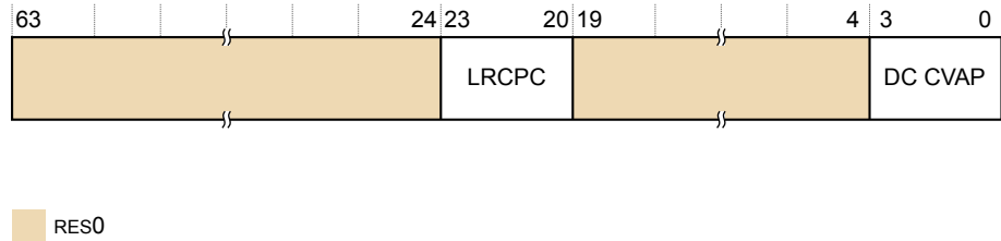
Figure B2-53 ID_AA64ISAR1_EL1 bit assignments
