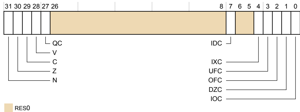
Figure B5-2 FPSR bit assignments
