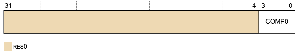
Figure D10-72 TRCVMIDCCTLRO bit assignments
