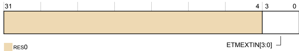
Figure D10-44 TRCITMISCIN bit assignments
