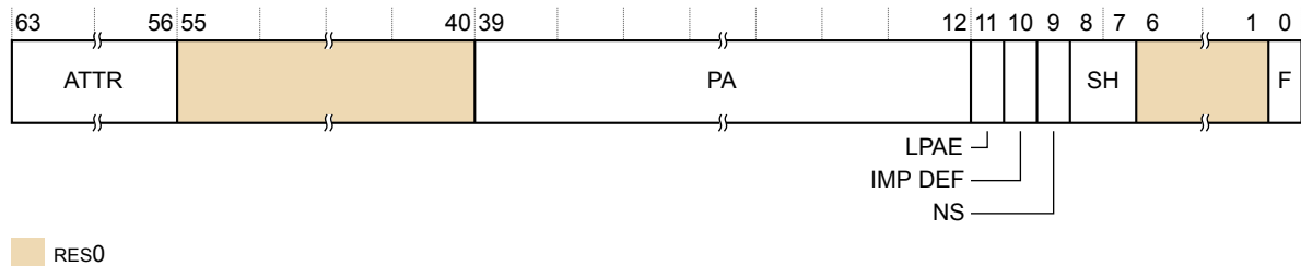
Figure B2-82 PAR bit assignments, PAR_EL1.F is 0
