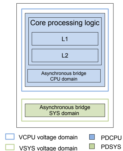
Figure A4-2 Cortex-X1 core power domain diagram
