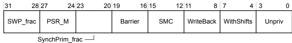
Figure B2-65 ID_ISAR4_EL1 bit assignments
