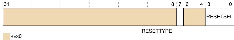
Figure D10-60 TRCSEQRSTEVR bit assignments
