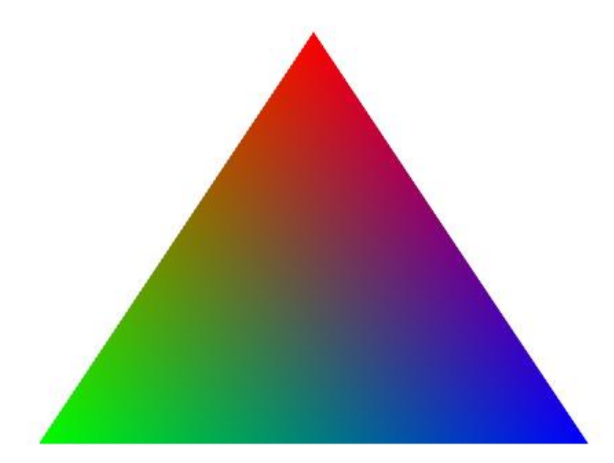
Figure 4 Color Interpolation
