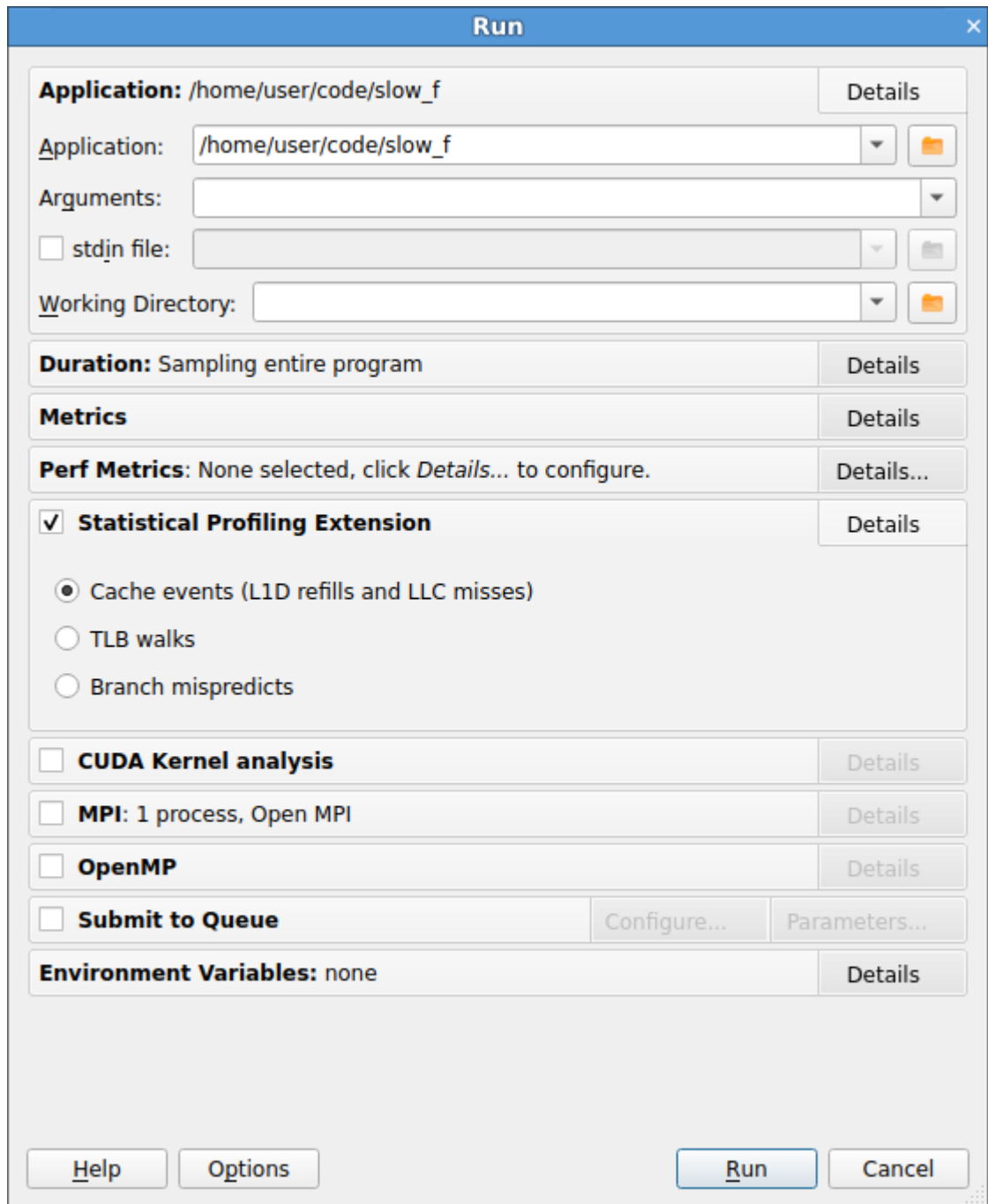
Figure C19-1 The Run dialog with SPE profiling enabled
