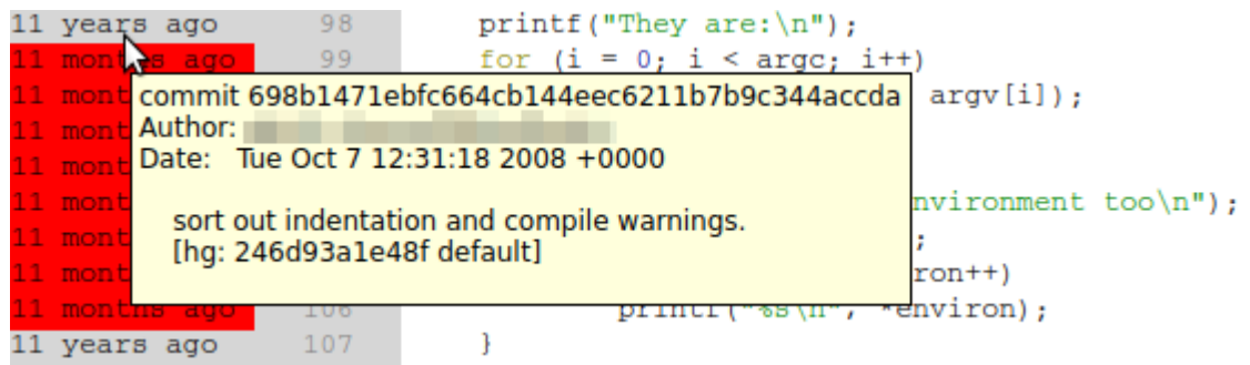
Figure B2-9 Version control information-tooltips
