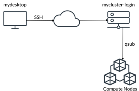
Figure A4-1 Connect-remotely
