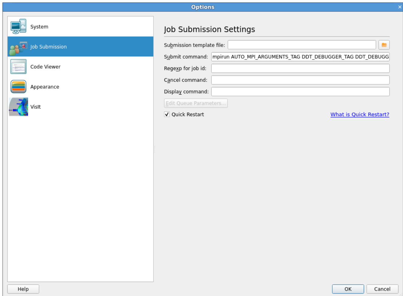
Figure B1-12 Using custom MPI scripts
