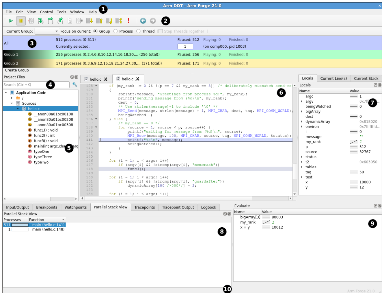
Figure B1-14 DDT main window
