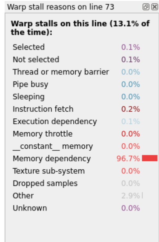
Figure C4-2 Selected lines view (GPU kernel)
