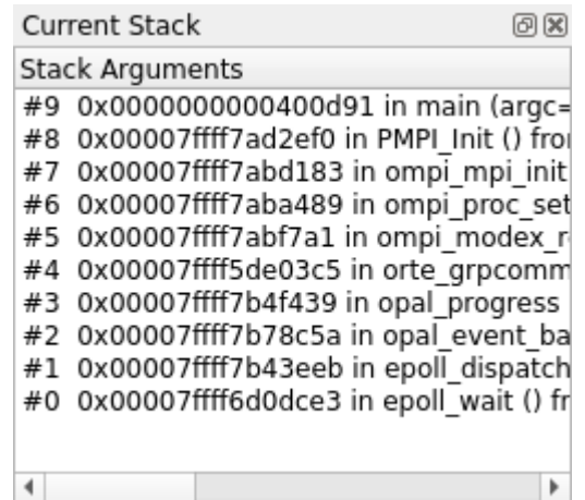
Figure B3-15 The Current Stack tab
