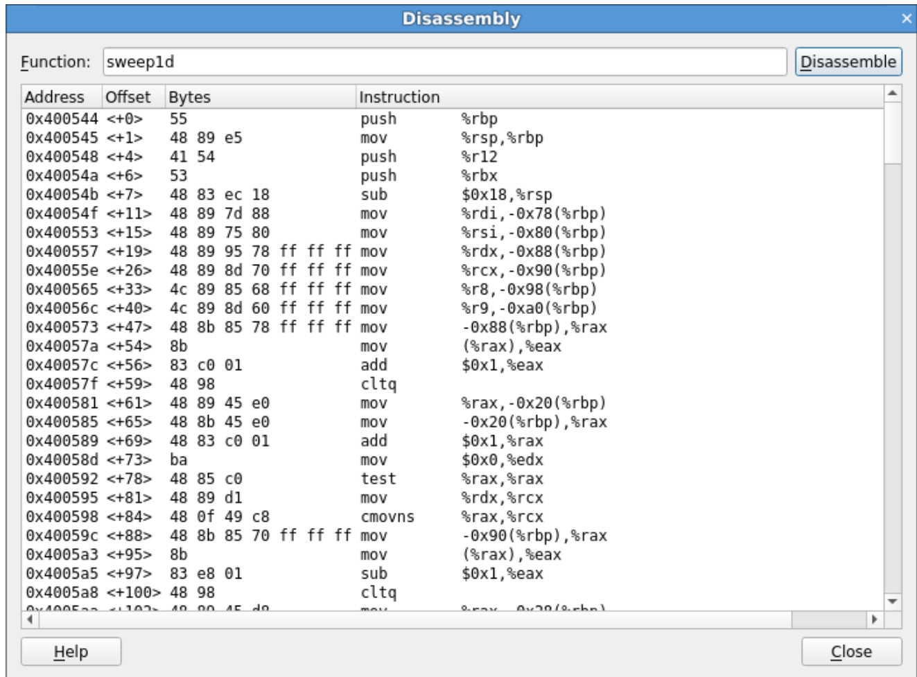
Figure B4-17 Disassembly dialog
