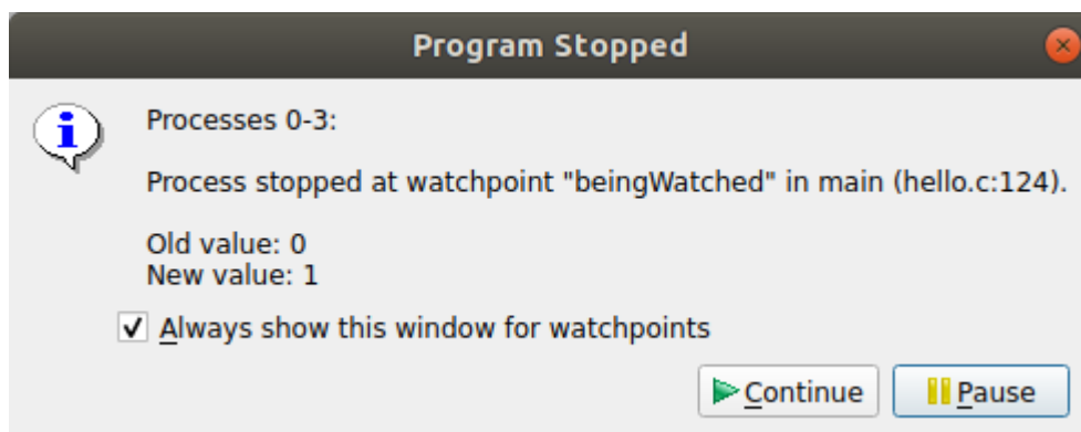
Figure B3-9 Program stopped at watchpoint
