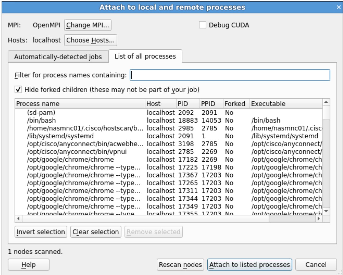
Figure B1-5 Attach window
