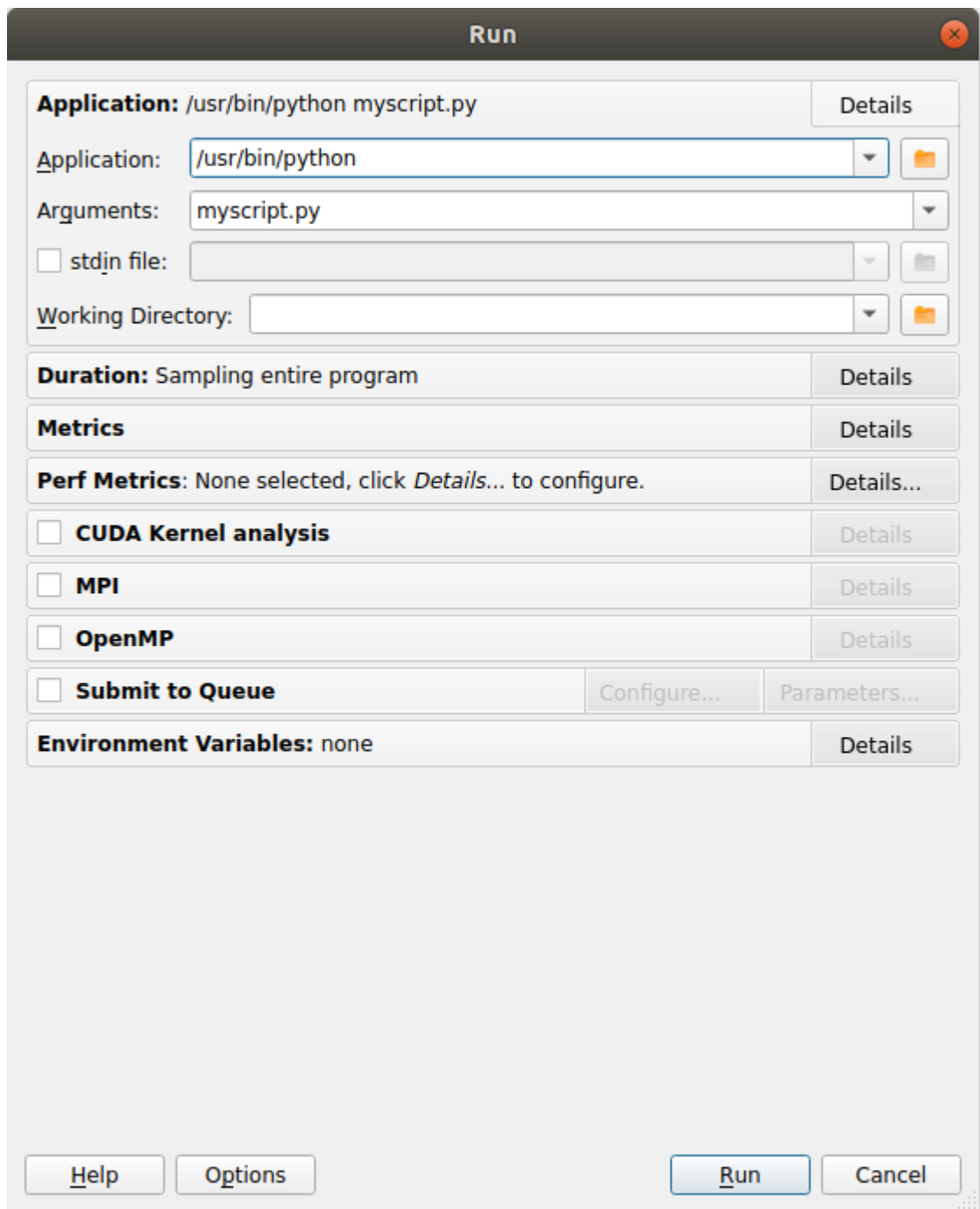
Figure C17-1 Profiling a Python script
