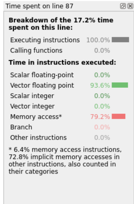
Figure C4-1 Selected lines view
