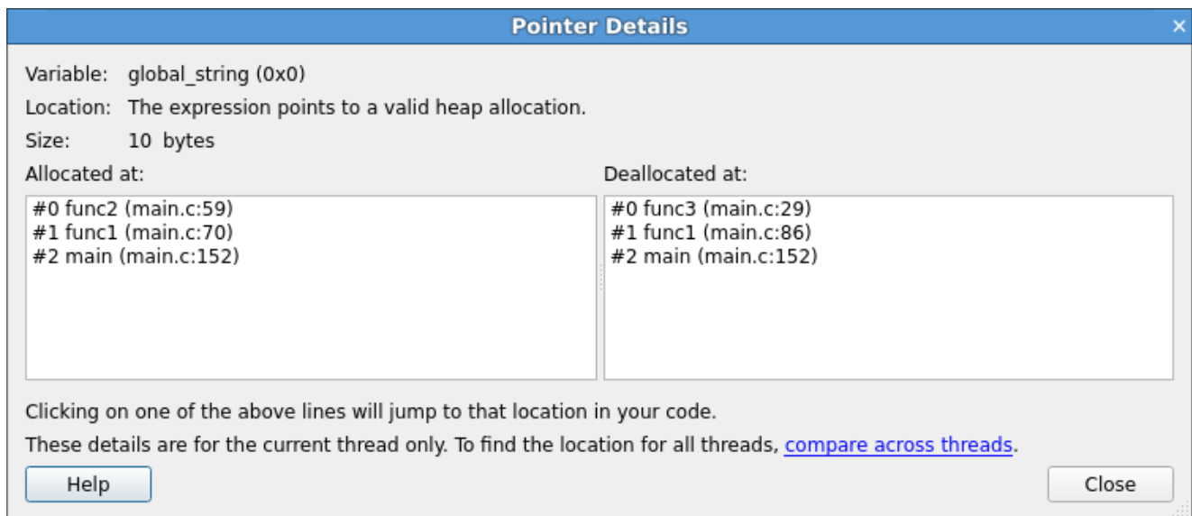
Figure B8-3 Pointer details
