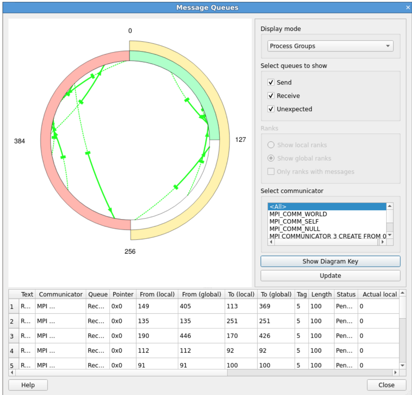
Figure B7-1 Message Queue window
