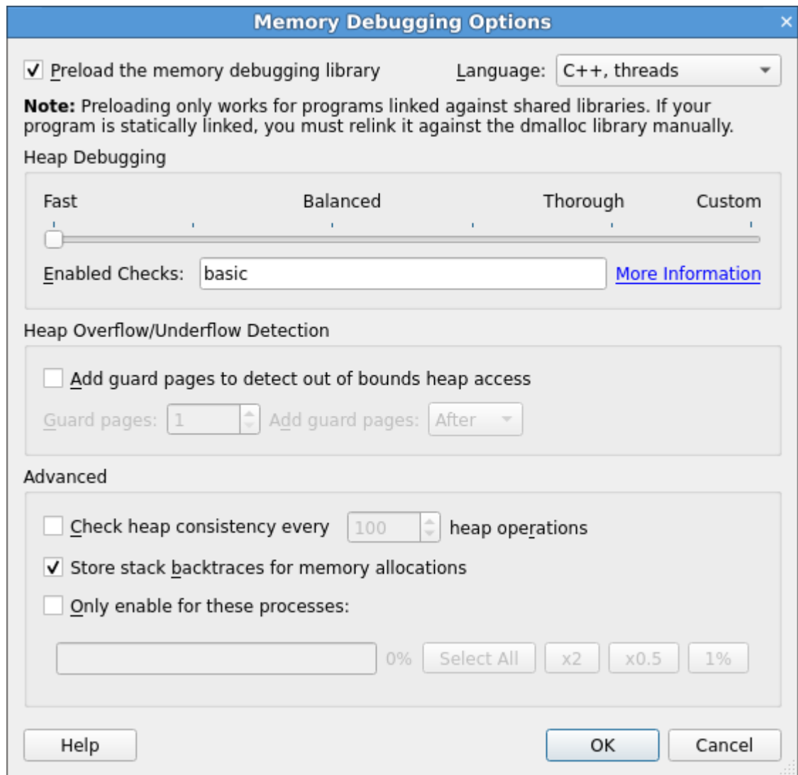
Figure B8-1 Memory Debugging Options
