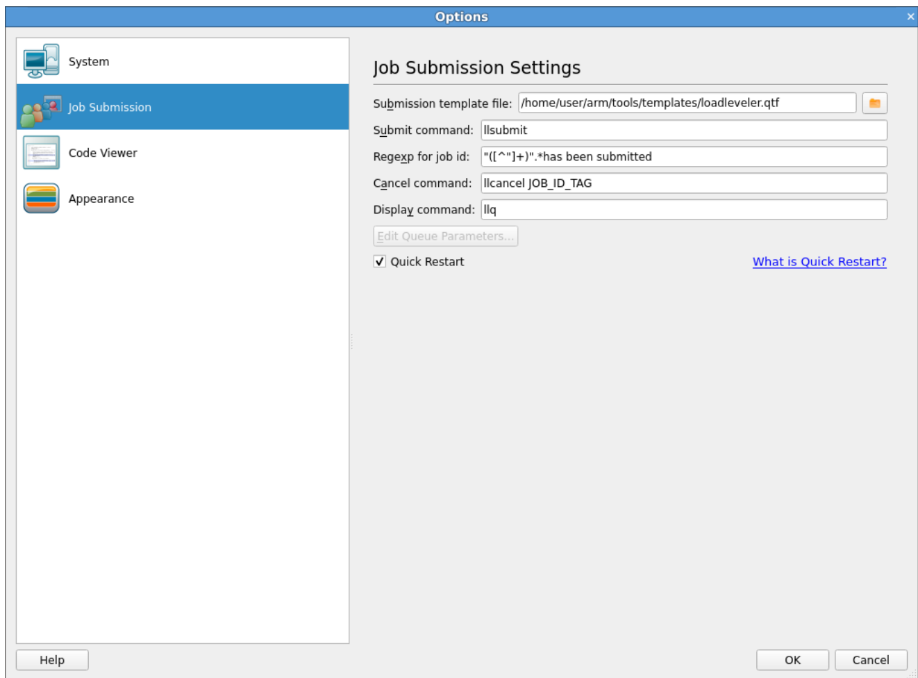
Figure C1-8 Using substitute MPI commands
