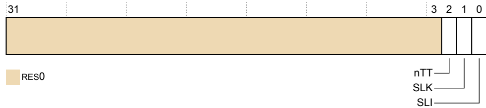
Figure D9-46 TRCLSR bit assignments
