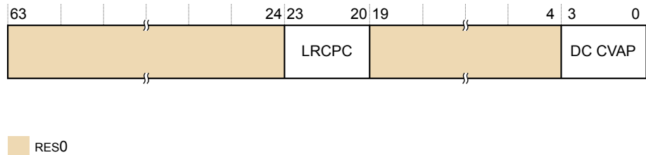
Figure B2-42 ID_AA64ISAR1_EL1 bit assignments
