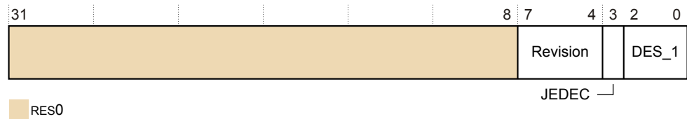
Figure D9-54 TRCPIDR2 bit assignments
