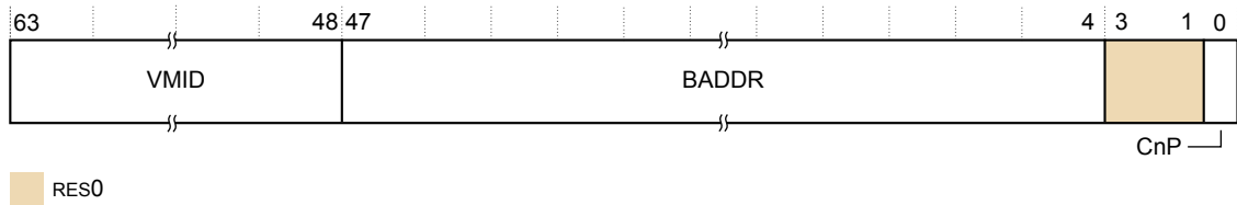
Figure B2-88 VTTBR_EL2 bit assignments
