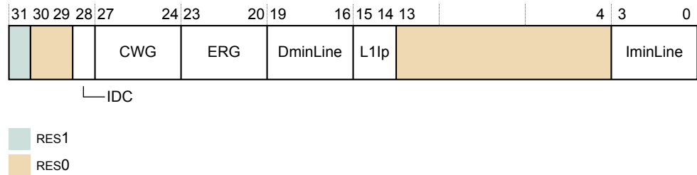
Figure B2-30 CTR_EL0 bit assignments
