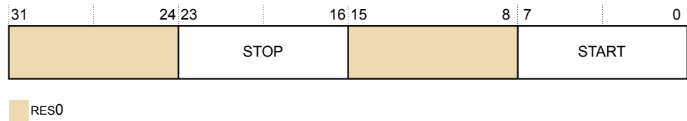
Figure D9-71 TRCVISSCTLR bit assignments
