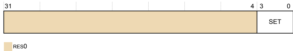
Figure D9-14 TRCCLAIMSET bit assignments
