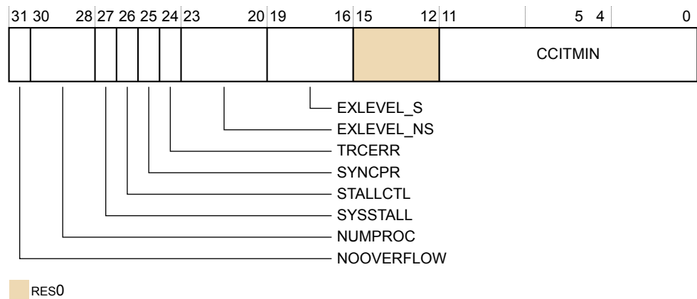
Figure D9-30 TRCIDR3 bit assignments
