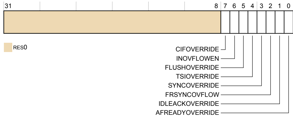
Figure D9-4 TRCAUXCTLR bit assignments
