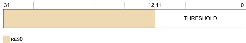
Figure D9-6 TRCCCCTL bit assignments
