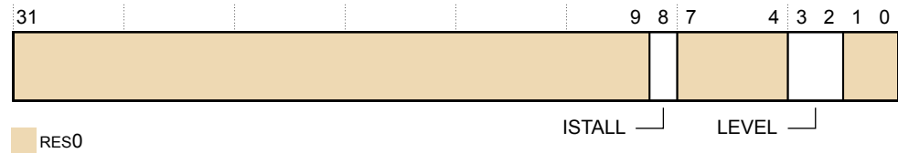
Figure D9-64 TRCSTALLCTLR bit assignments
