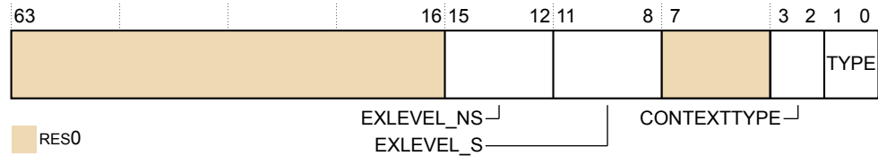
Figure D9-1 TRCACATRn bit assignments
