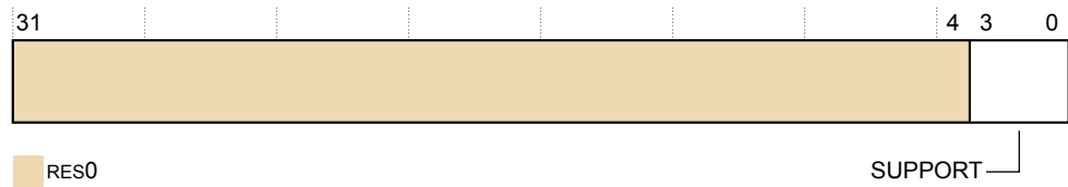
Figure D9-39 TRCIMSPEC0 bit assignments
