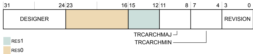
Figure D9-28 TRCIDR1 bit assignments
