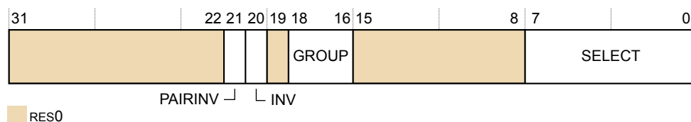
Figure D9-58 TRCRSCTLRn bit assignments
