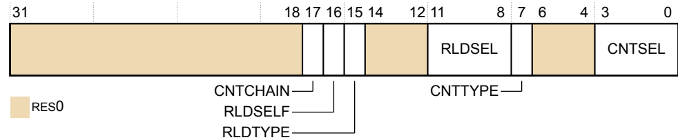
Figure D9-16 TRCCNTCTLR1 bit assignments
