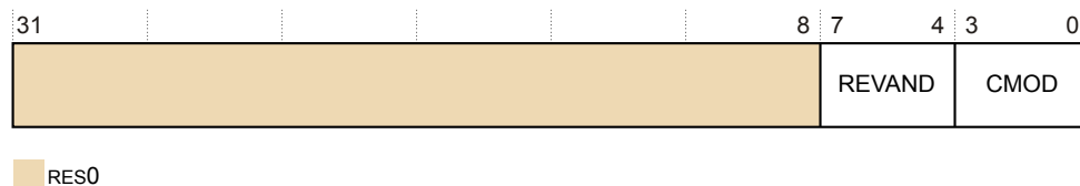
Figure D9-55 TRCPIDR3 bit assignments
