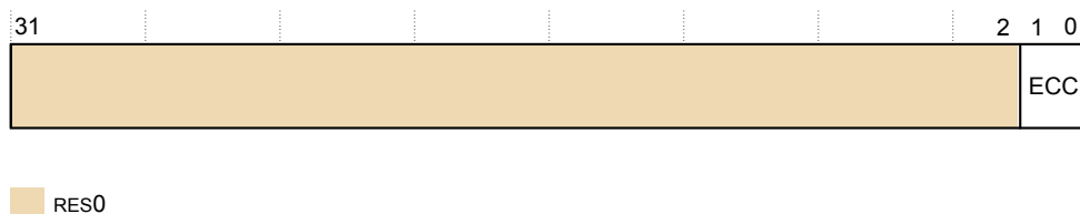
Figure B2-22 CPUCFR_EL1 bit assignments
