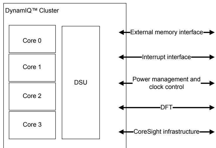
Figure A1-1 Example Cortex-A76 configuration
