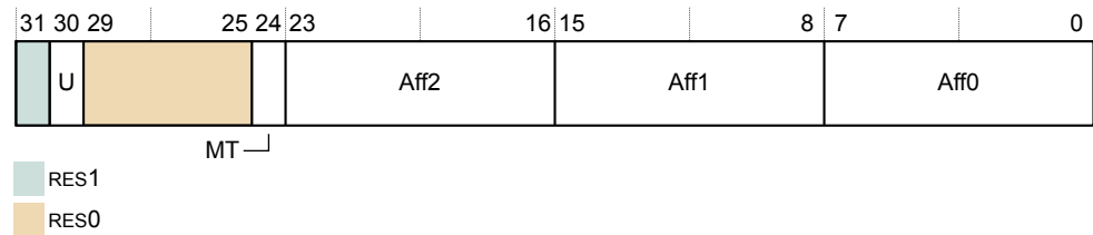
Figure D9-20 TRCDEVAFF0 bit assignments
