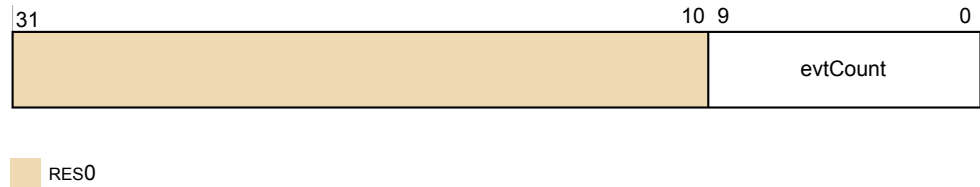
Figure D8-4 AMEVTYPERN_EL0 bit assignments
