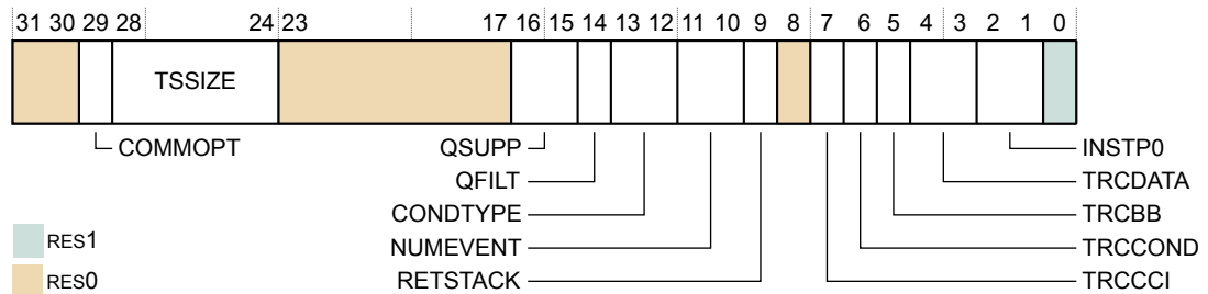
Figure D9-27 TRCIDR0 bit assignments
