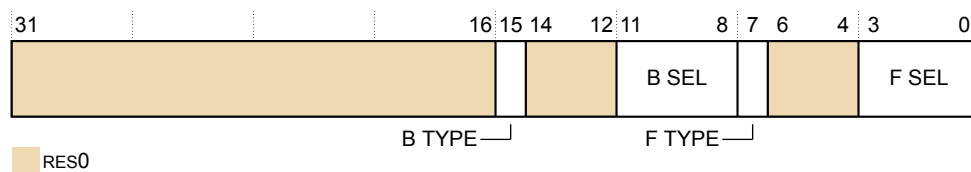
Figure D9-59 TRCSEQEVRn bit assignments
