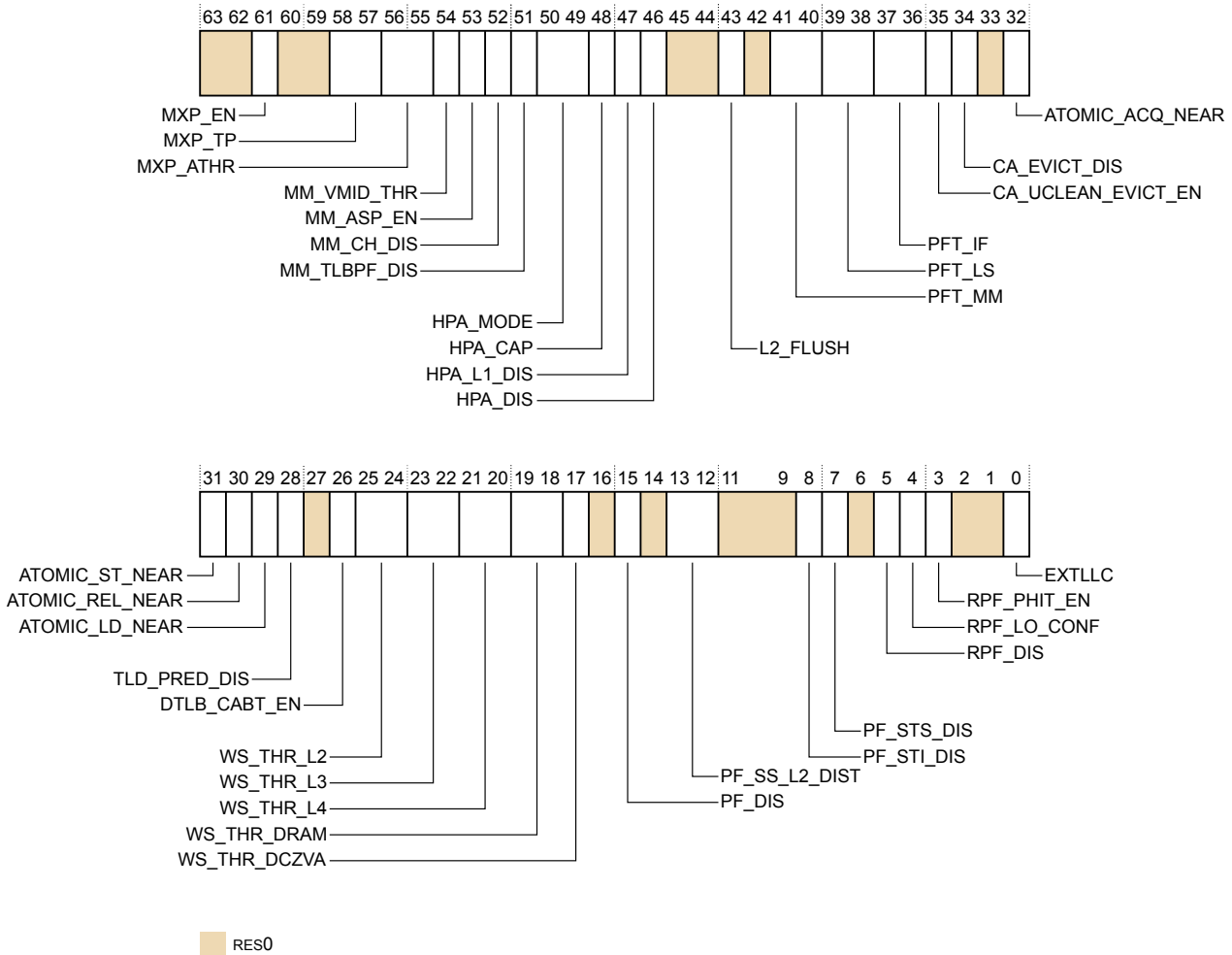
Figure B2-23 CPUECTLR_EL1 bit assignments
