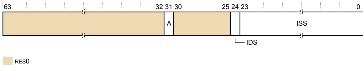
Figure B2-85 VDISR_EL2 at EL1 using AArch64
