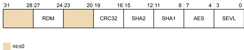
Figure B2-55 ID_ISAR5_EL1 bit assignments
