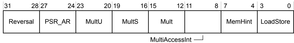
Figure B2-52 ID_ISAR2_EL1 bit assignments
