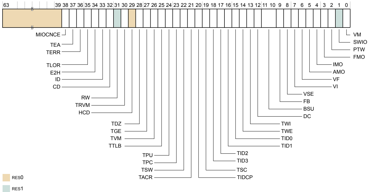
Figure B2-39 HCR_EL2 bit assignments
