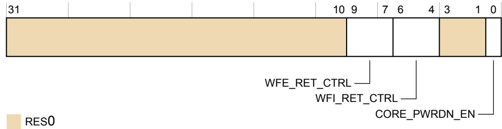
Figure B2-28 CPUPWRCTLR_EL1 bit assignments
