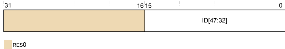
Figure D5-2 PMCEID1_EL0 bit assignments
