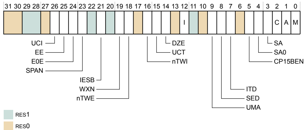
Figure B2-75 SCTL R _EL1 bit assignments
