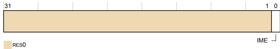
Figure D9-41 TRCITCTRL bit assignments
