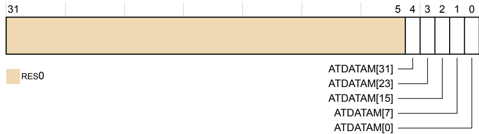
Figure D9-44 TRCITIDATAR bit assignments
