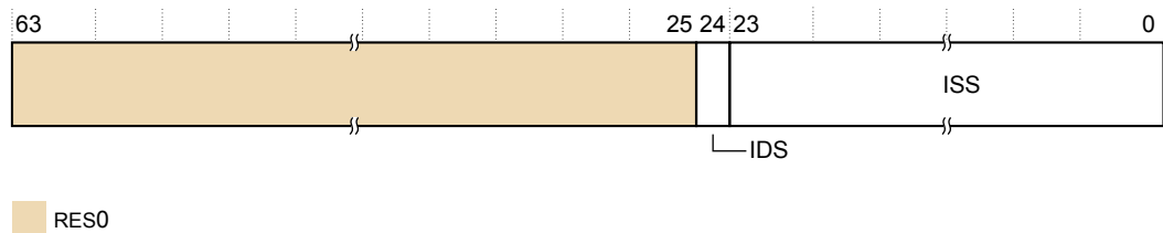
Figure B2-86 VESR_EL2 bit assignments
