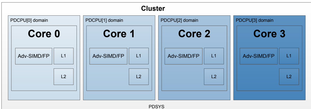
Figure A4-3 Cortex-A76 power domains at enyo_core level
