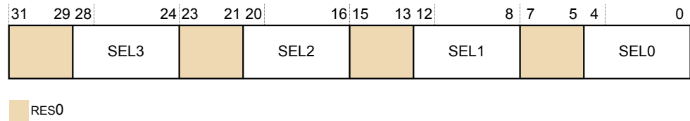
Figure D9-26 TRCEXTINSEL bit assignments
