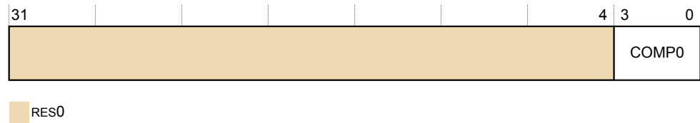
Figure D9-7 TRCCIDCCTL0 bit assignments
