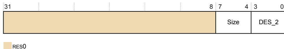
Figure D9-56 TRCPIDR4 bit assignments
