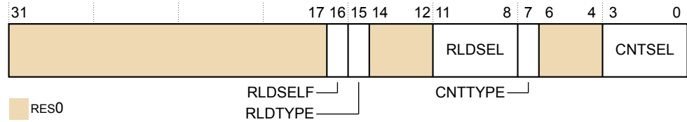
Figure D9-15 TRCCNTCTLR0 bit assignments
