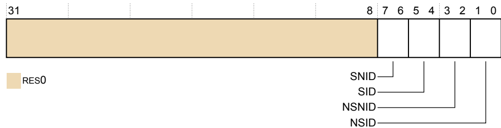
Figure D9-3 TRCAUTHSTATUS bit assignments
