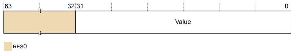
Figure D9-8 TRCCIDCVR0 bit assignments
