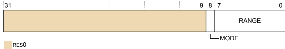
Figure D9-5 TRCBBCTLR bit assignments
