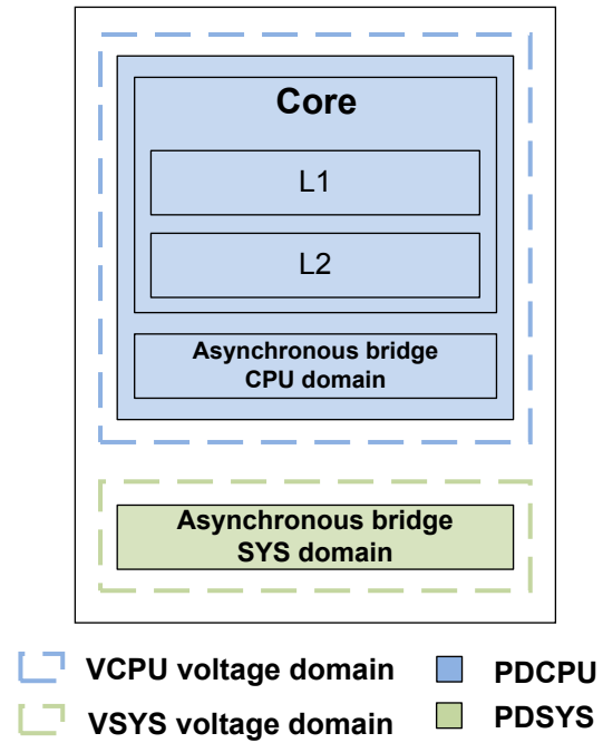
Figure A4-2 Cortex-A76 core power domain diagram at enyo_core level
