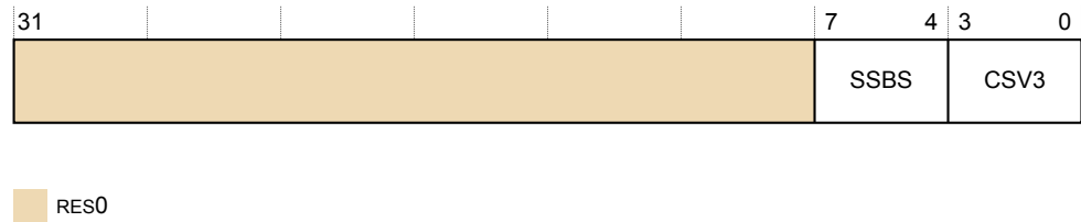
Figure B2-64 ID_PFR2_EL1 bit assignments
