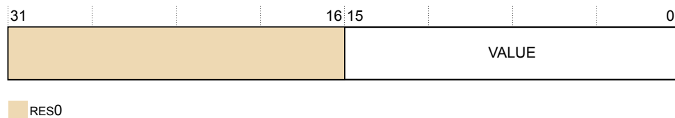
Figure D9-17 TRCCNTRLDVRn bit assignments
