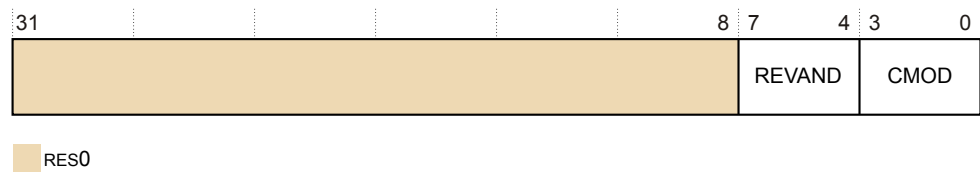
Figure D6-53 TRCPIDR3 bit assignments
