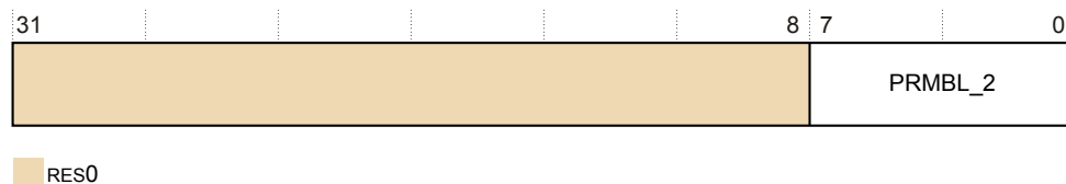
Figure D6-11 TRCCIDR2 bit assignments
