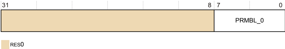
Figure D6-9 TRCCIDR0 bit assignments
