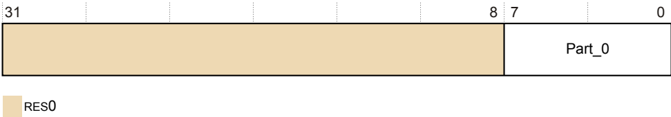
Figure D6-50 TRCPIDR0 bit assignments
