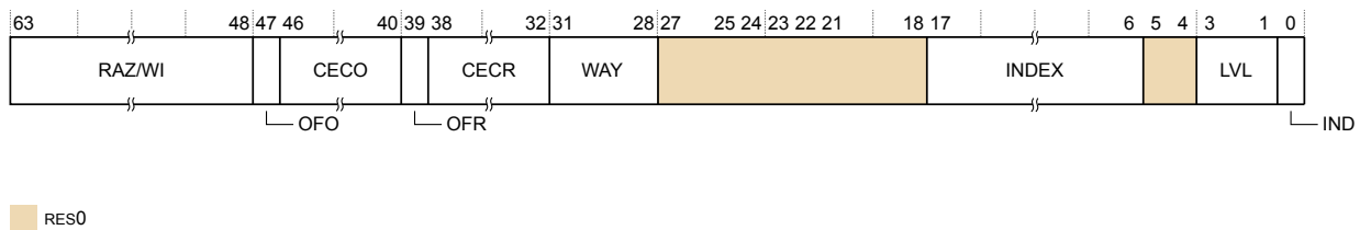
Figure B2-3 ERR0MISC0 bit assignments
