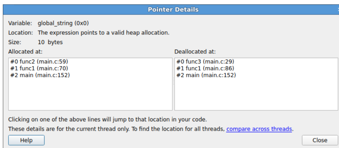
Figure 83: Pointer details
