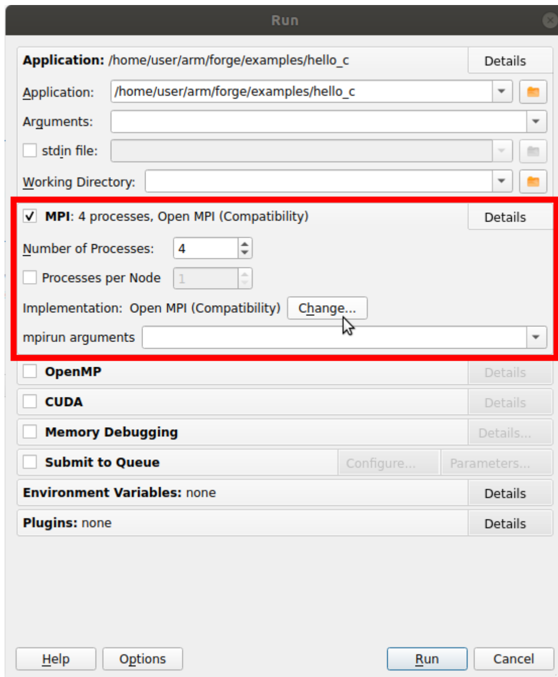
Figure 131: Setting the MPI Implementation in the GUI
