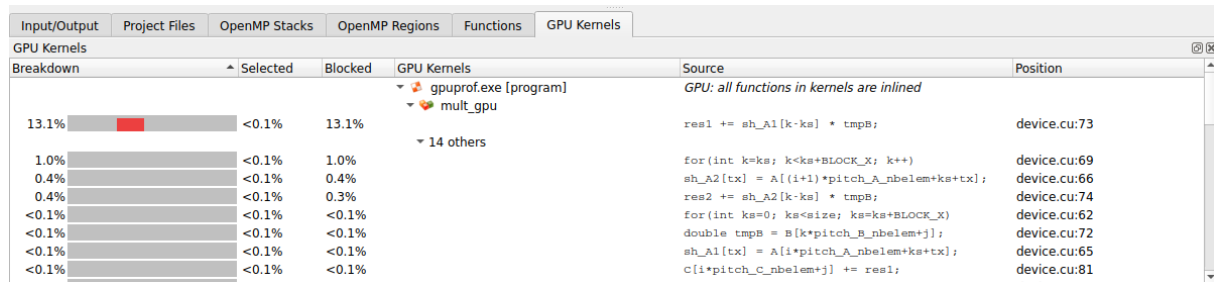
Figure 121: GPU kernels view (with CUDA kernel analysis)
