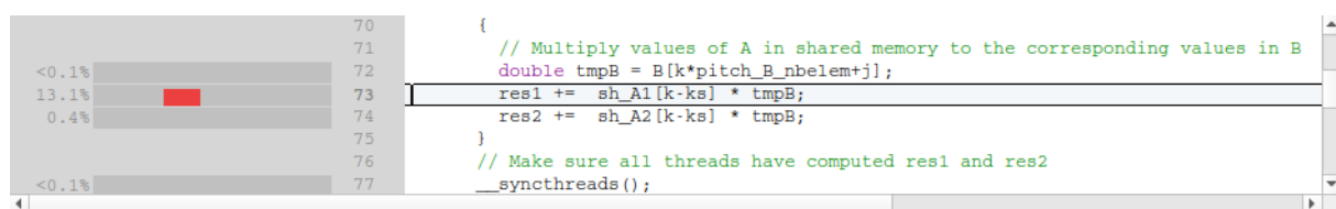
Figure 105: Source Code View (GPU Kernel)
