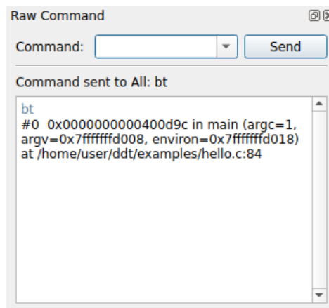
Figure 75: Raw Command Window
