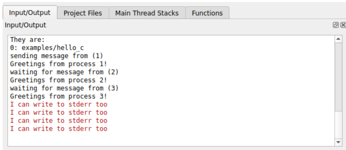
Figure 102: MAP Standard Output Window
