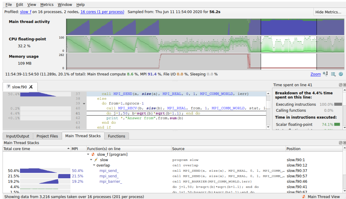
Figure 116: Map with a region of time selected
