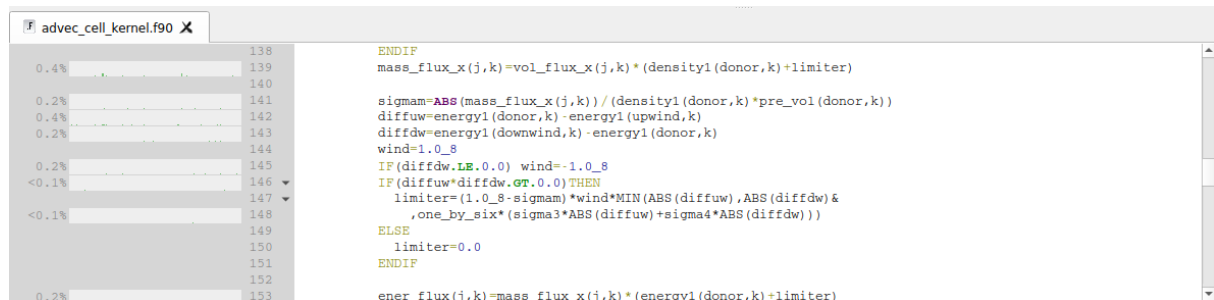
Figure 106: Typical Fortran Code in MAP
