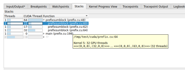
Figure 88: CUDA threads in the parallel stack view
