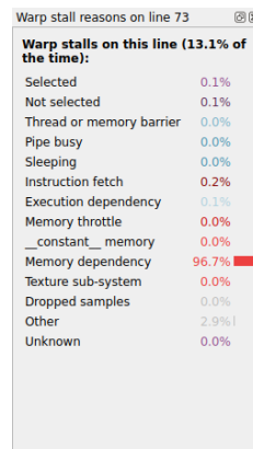
Figure 110: Selected lines view (GPU kernel)
