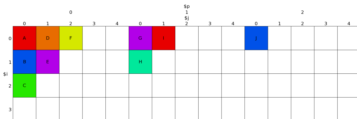
Figure 69: A three dimensional distributed array comprised of the local array myArray($i, $j) with \$i = 0..3 and \$j = 0..4 on ranks 0–2 projected onto the Data Table with \$p (the distributed dimension) and \$j displayed as Columns and \$i displayed as Rows.
