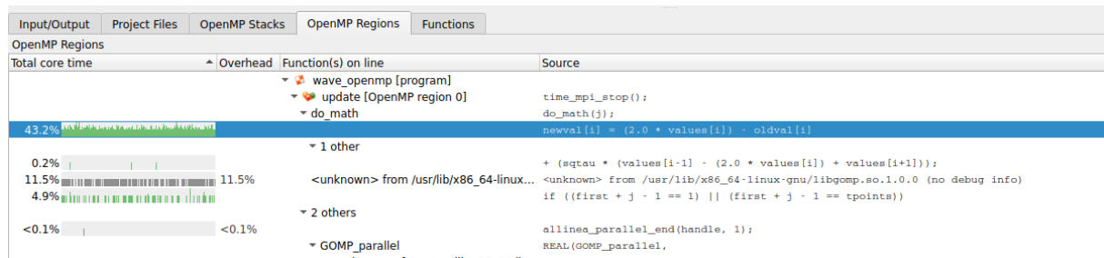
Figure 112: OpenMP Regions View
