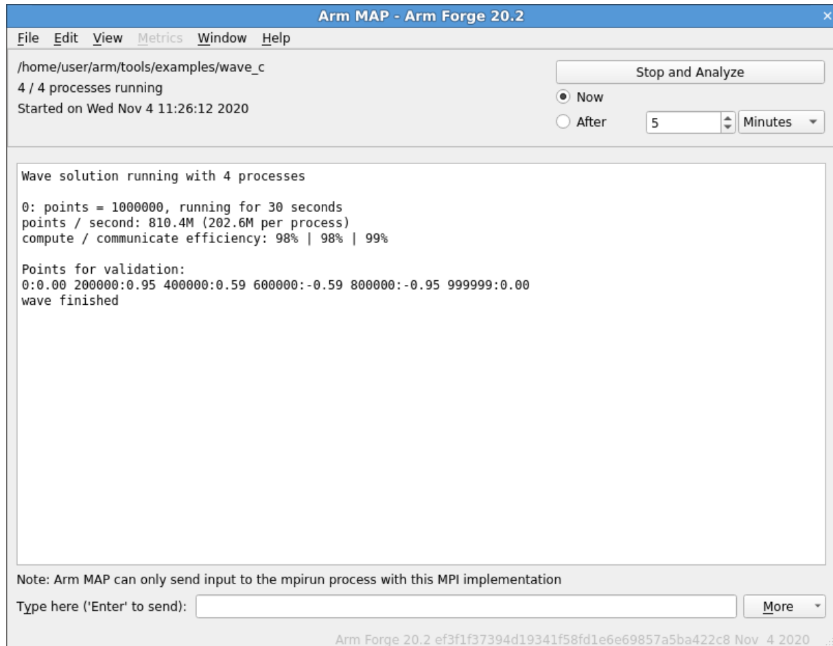
Figure 97: Running window
