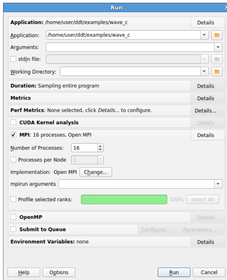
Figure 96: Run window
