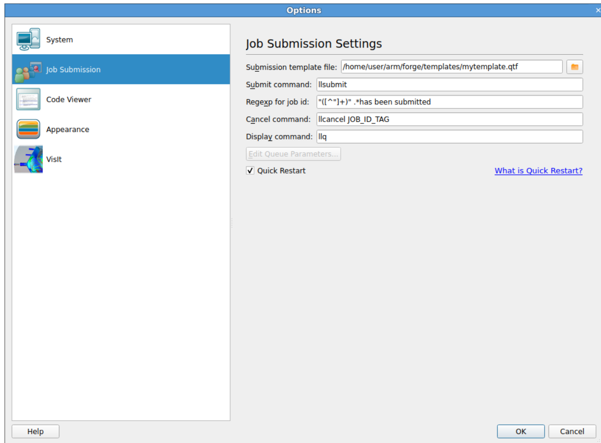
Figure 127: Queuing Systems
