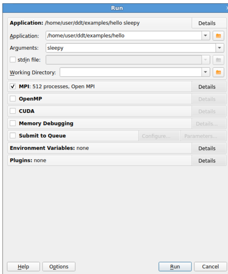
Figure 12: Run Window
