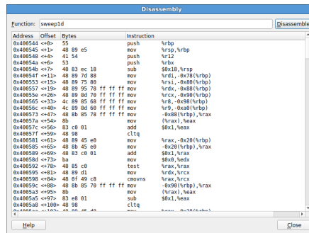
Figure 74: Disassemble Tool
