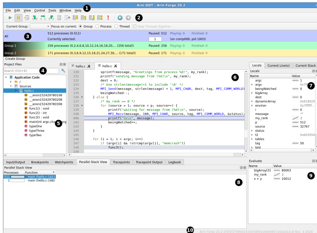
Figure 25: DDT Main Window
