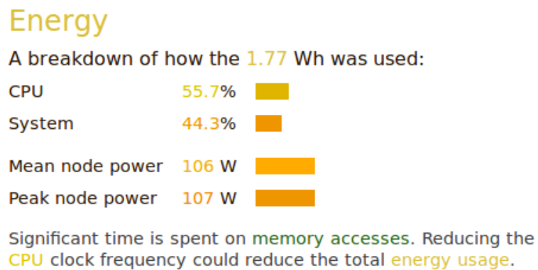
Figure 126: Energy metrics report
