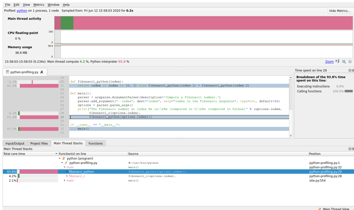
Figure 123: Viewing Python profiling results
