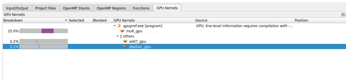
Figure 119: GPU Kernels View
