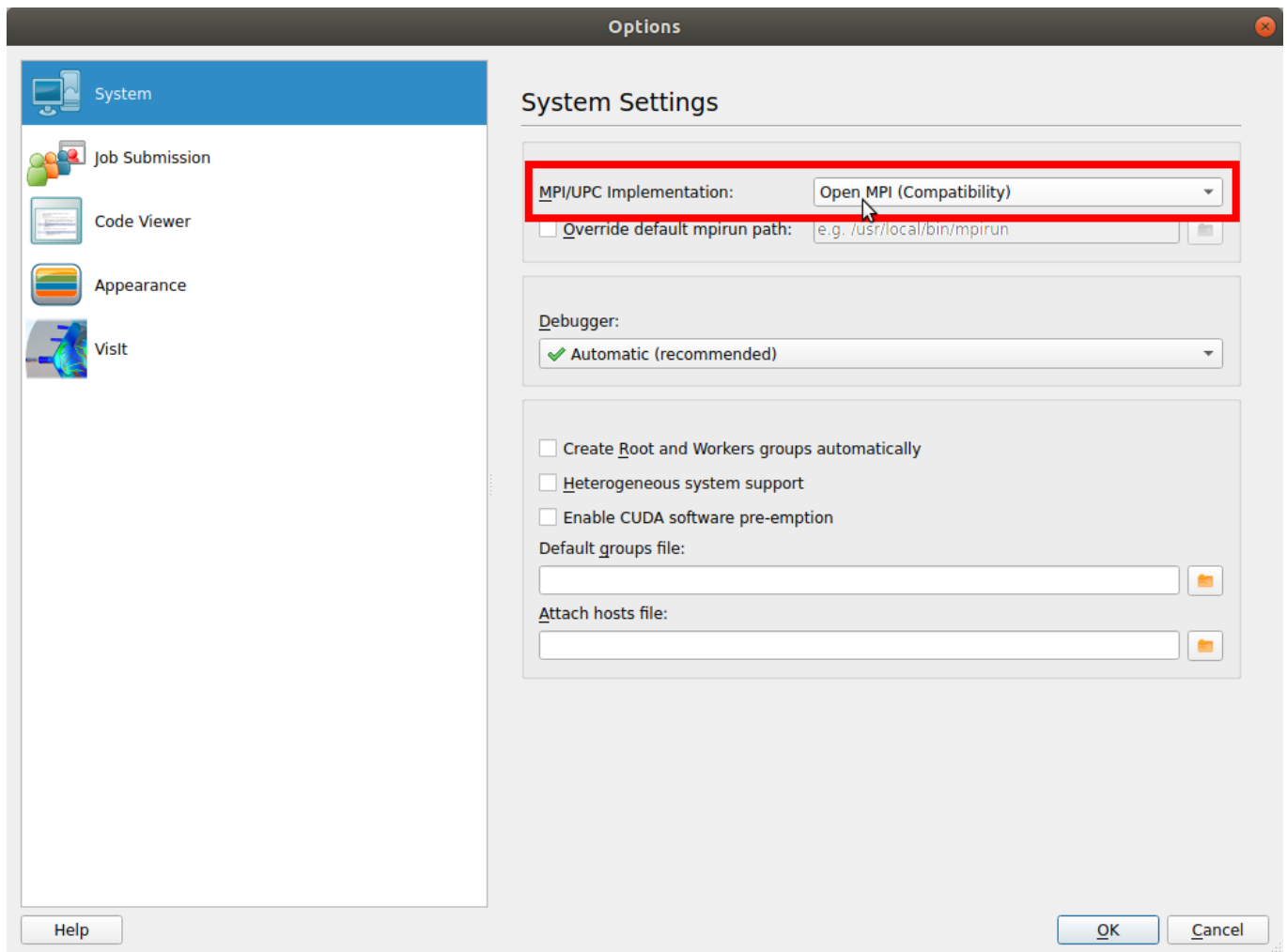
Figure 132: Setting the MPI Implementation in System Settings
