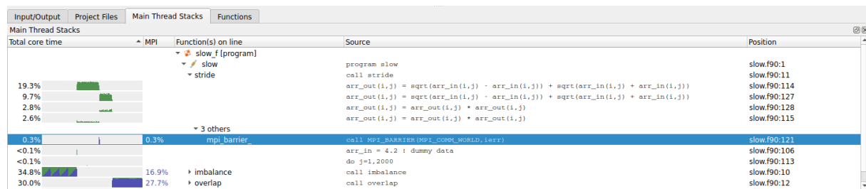
Figure 111: MAP Stacks View
