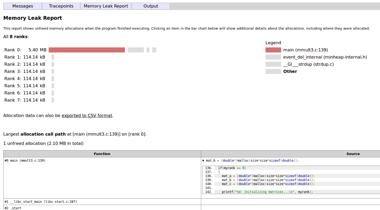
Figure 93: Memory leak report detail
