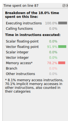
Figure 109: Selected Lines View
