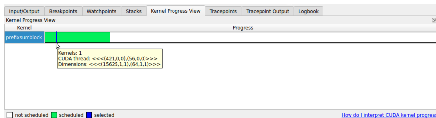
Figure 89: Kernel Progress Display
