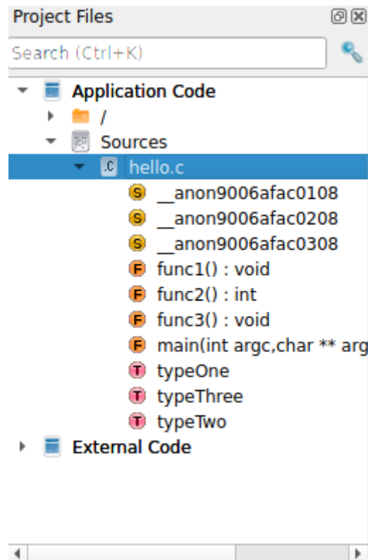
Figure 29: Function Listing
