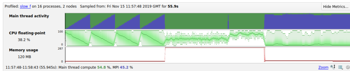
Figure 115: Metrics view
