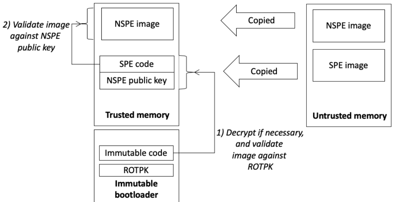
Figure 8: Example boot from untrusted memory
