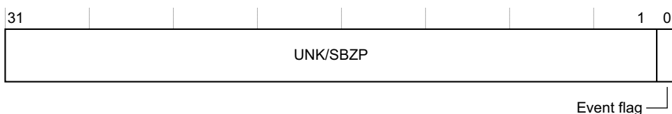
Figure 9-29 Global Timer Interrupt Status Register bit assignments
