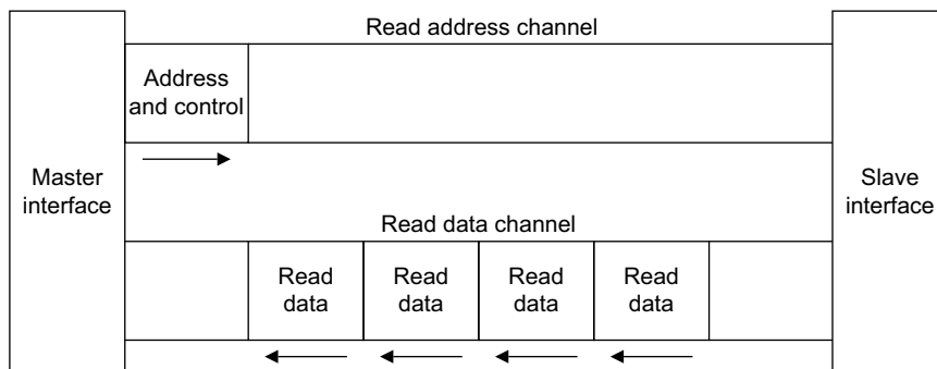
Figure A1-2 Channel architecture of reads
