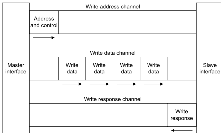
Figure A1-1 Channel architecture of writes
