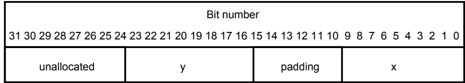
Figure 15-2 Bitfield allocation 1
