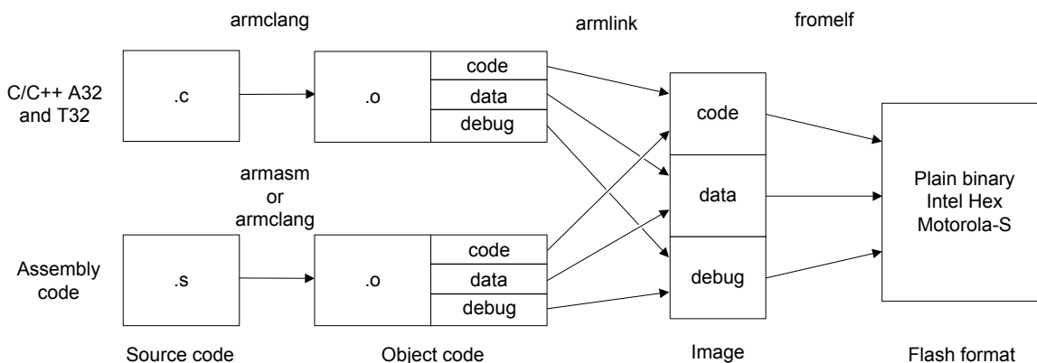
Figure 1-1 Compiler toolchain
