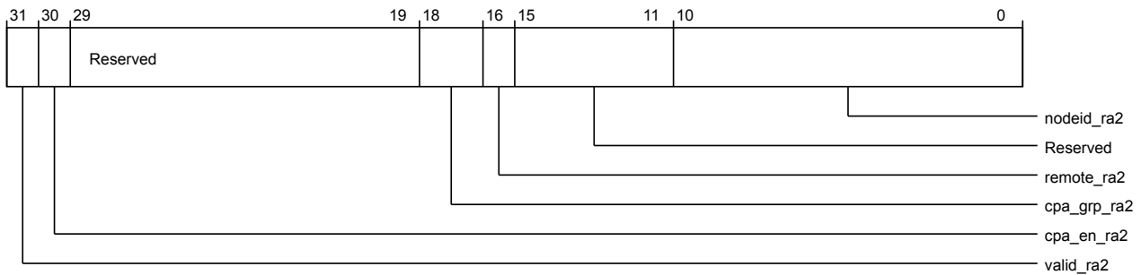
Figure 3-415 por_hnf_por_hnf_rn_phys_id1 (low)
