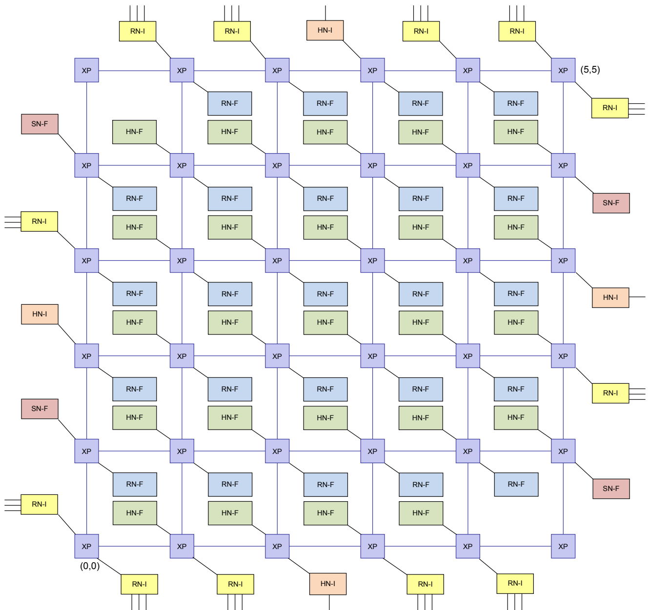
Figure 2-3 Example 6 × 6 mesh configuration
