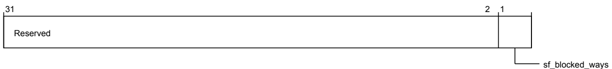
Figure 3-477 por_hnf_por_hnf_sf_cxg_blocked_ways (low)
