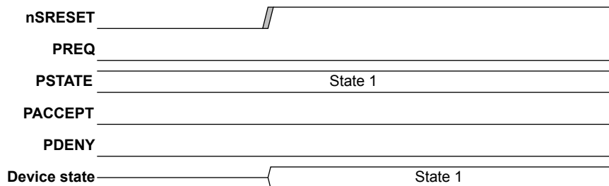
Figure 2-59 Reset state initialization
