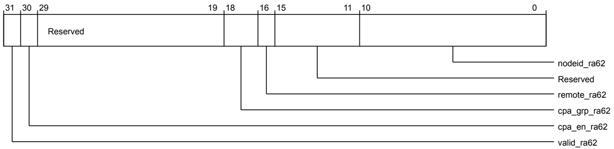
Figure 3-475 por_hnf_por_hnf_rn_phys_id31 (low)
