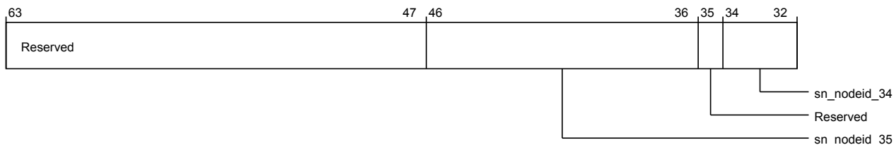
Figure 3-918 por_rnsam_sys_cache_grp_sn_nodeid_reg8 (high)
