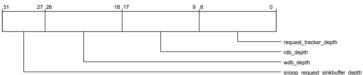
Figure 3-975 por_cxg_ha_por_cxg_ha_unit_info (low)
