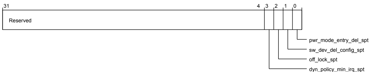
Figure 3-315 por_hnf_por_hnf_ppu_idr1
