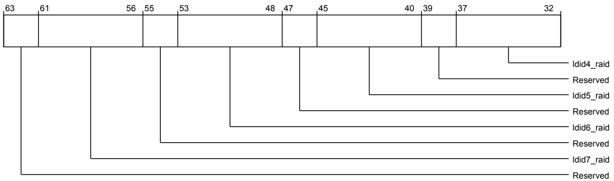
Figure 3-1130 por_cxg_ra_por_cxg_ra_rnd_ldid_to_raid_reg0 (high)
