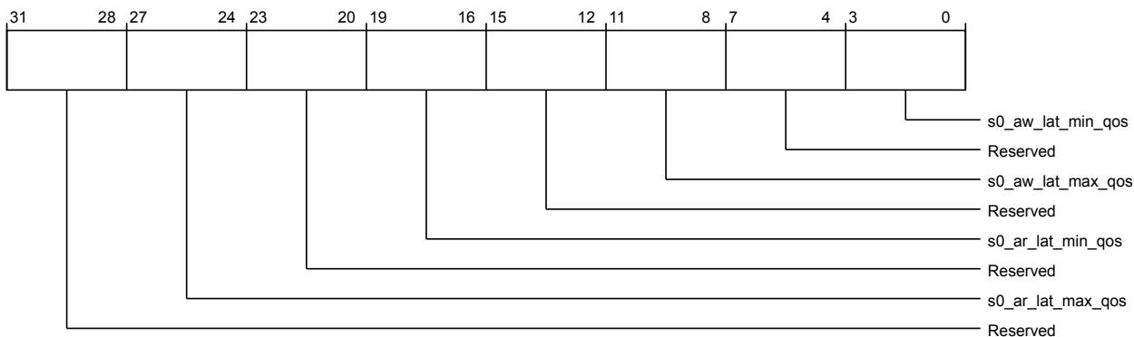
Figure 3-739 por_rnd_por_rnd_s0_qos_lat_range (low)
