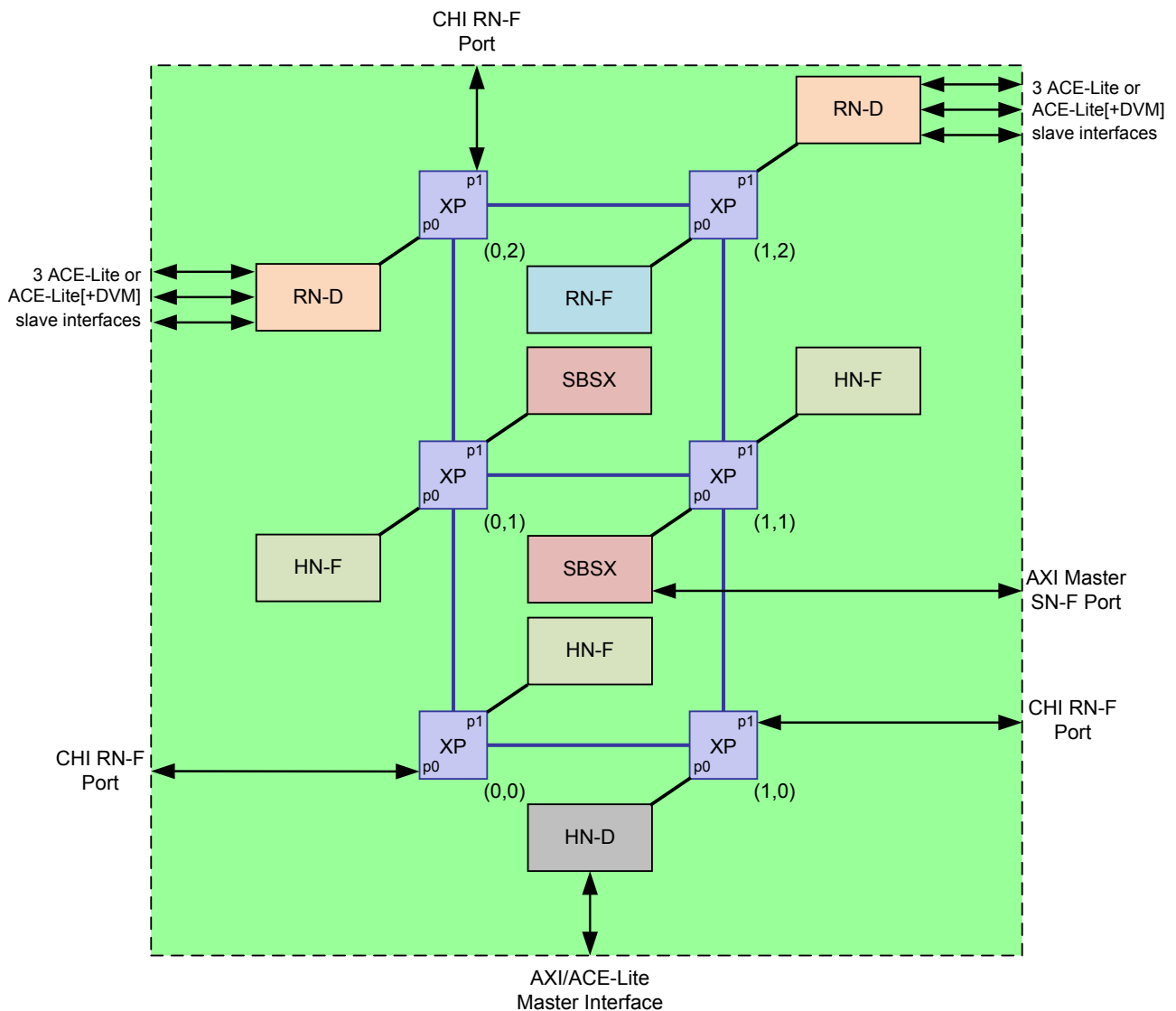
Figure 2-50 CMN-600 clock domain – fully synchronous
