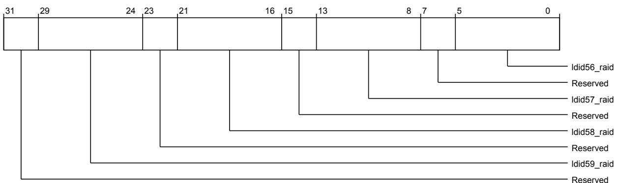
Figure 3-1121 por_cxg_ra_por_cxg_ra_rnf_ldid_to_raid_reg7 (low)
