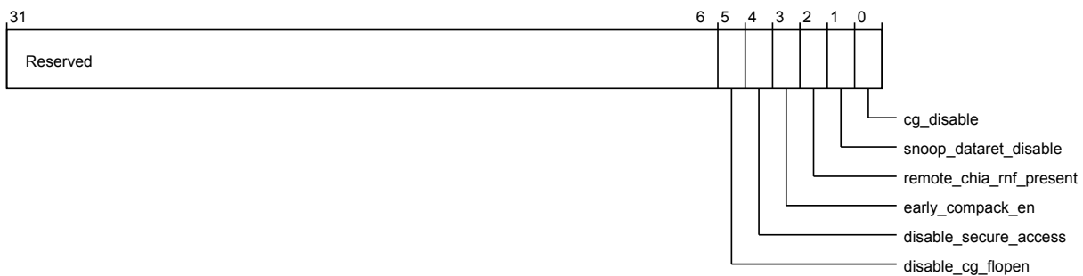
Figure 3-971 por_cxg_ha_por_cxg_ha_aux_ctl (low)
