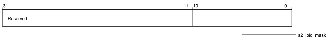
Figure 3-731 por_rnd_por_rnd_s2_port_control (low)
