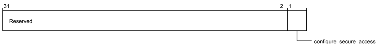
Figure 3-18 por_cfgm_por_cfgm_secure_access (low)
