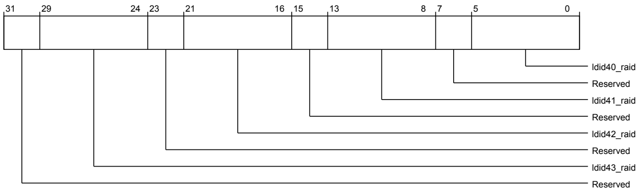
Figure 3-1117 por_cxg_ra_por_cxg_ra_rnf_ldid_to_raid_reg5 (low)
