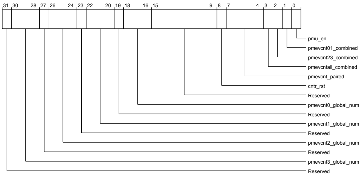
Figure 3-709 por_mxp_por_dtm_pmu_config (low)
