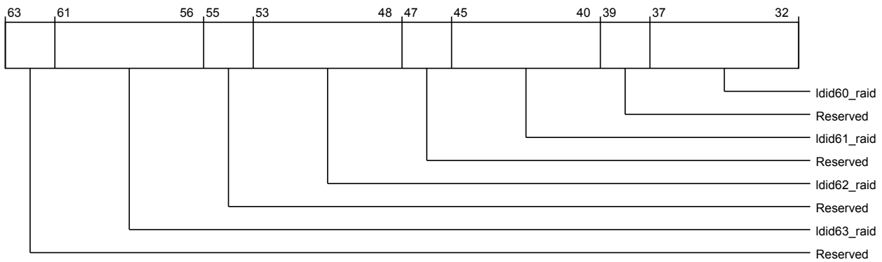
Figure 3-1120 por_cxg_ra_por_cxg_ra_rnf_ldid_to_raid_reg7 (high)
