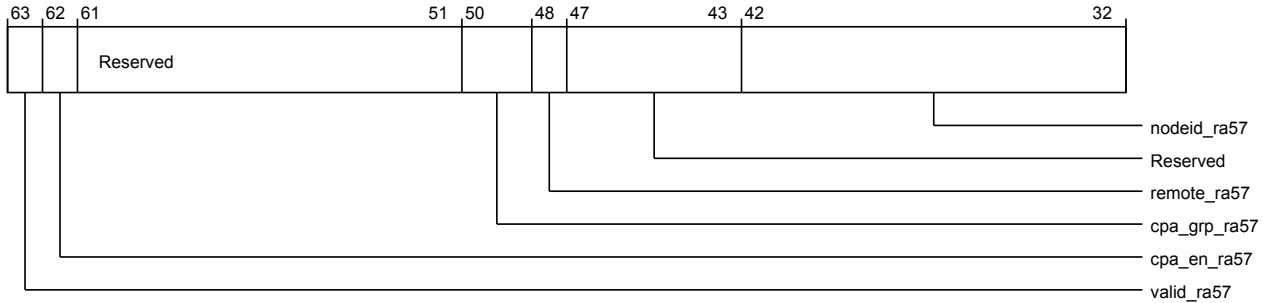
Figure 3-468 por_hnf_por_hnf_rn_phys_id28 (high)
