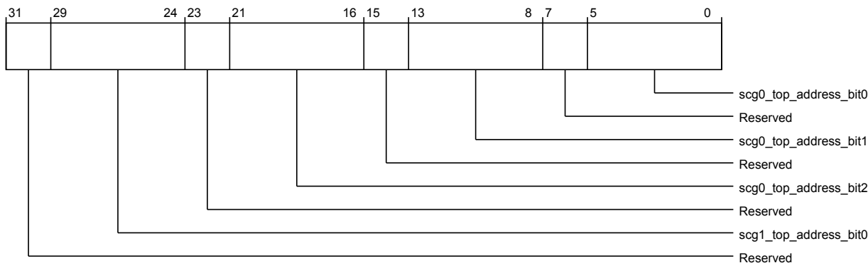
Figure 3-871 por_rnsam_sys_cache_grp_sn_sam_cfg0 (low)
