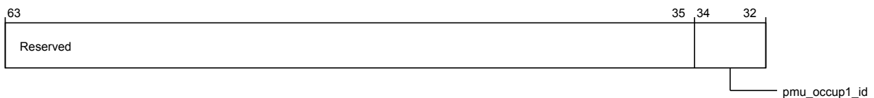
Figure 3-510 por_hnf_por_hnf_pmu_event_sel (high)
