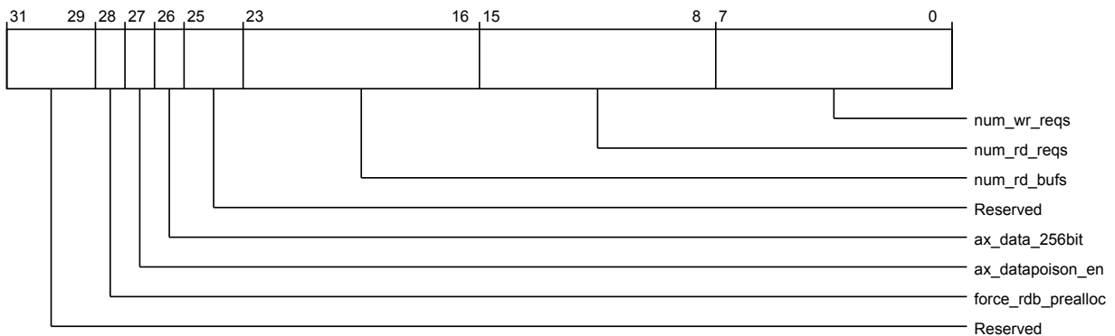
Figure 3-721 por_rnd_por_rnd_unit_info (low)
