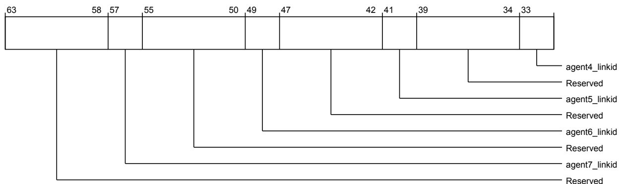
Figure 3-992 por_cxg_ha_por_cxg_ha_agentid_to_linkid_reg0 (high)
