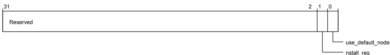
Figure 3-815 por_rnsam_rnsam_status (low)
