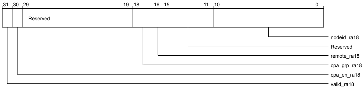
Figure 3-431 por_hnf_por_hnf_rn_phys_id9 (low)
