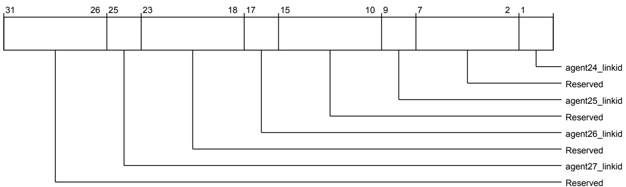
Figure 3-1097 por_cxg_ra_por_cxg_ra_agentid_to_linkid_reg3 (low)
