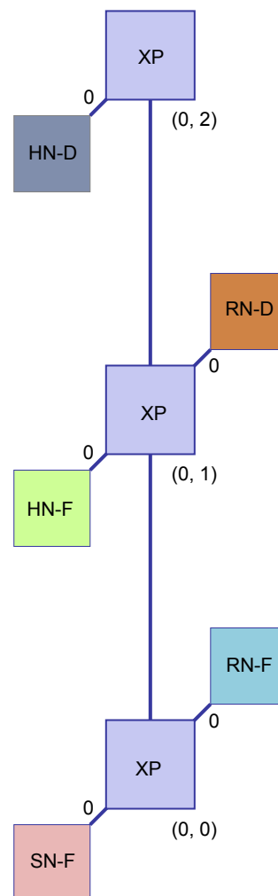
Figure 2-5 1 \times 3 mesh example
