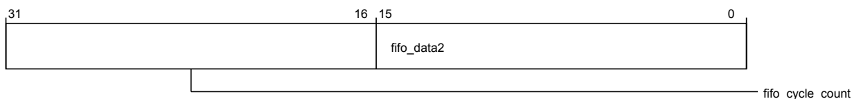
Figure 3-667 por_mxp_por_dtm_fifo_entry1_2 (low)
