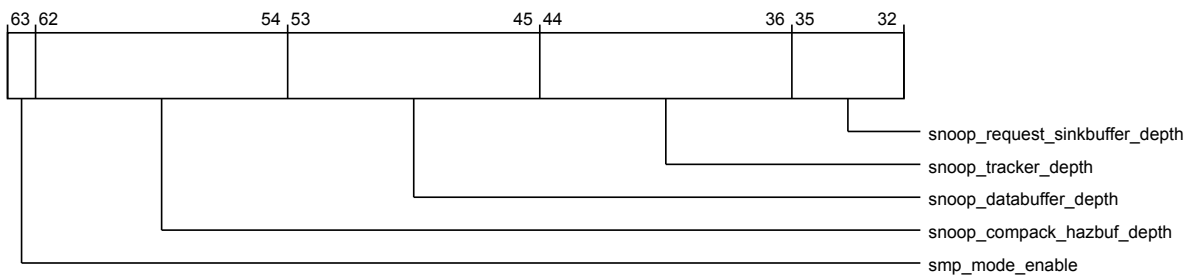
Figure 3-974 por_cxg_ha_por_cxg_ha_unit_info (high)
