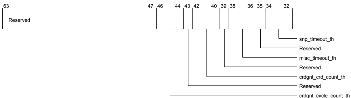
Figure 3-1168 por_cxla_por_cxla_aux_ctl (high)
