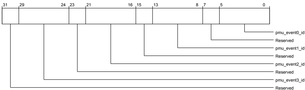
Figure 3-1147 por_cxg_ra_pmu_event_sel (low)
