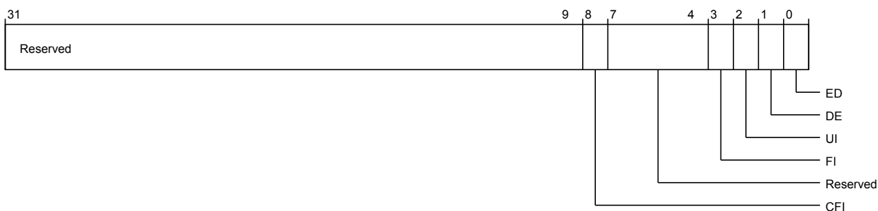
Figure 3-535 por_hni_errctlr (low)
