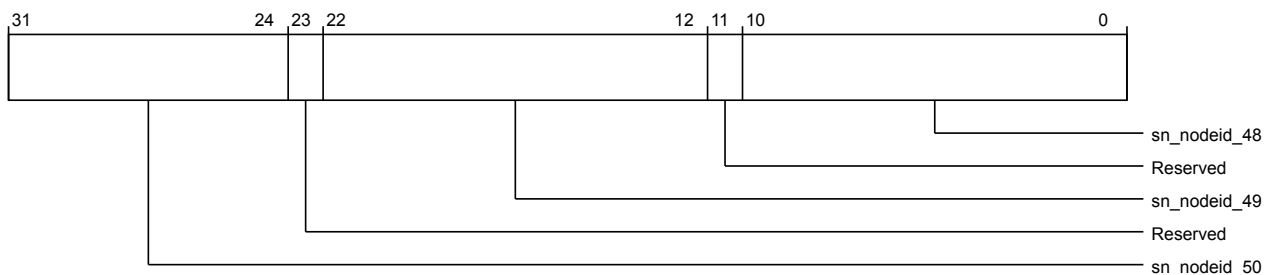
Figure 3-927 por_rnsam_sys_cache_grp_sn_nodeid_reg12 (low)
