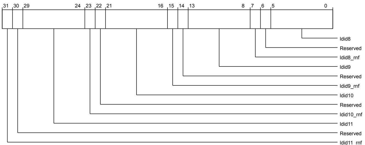
Figure 3-979 por_cxg_ha_por_cxg_ha_rnf_raid_to_ldid_reg1 (low)
