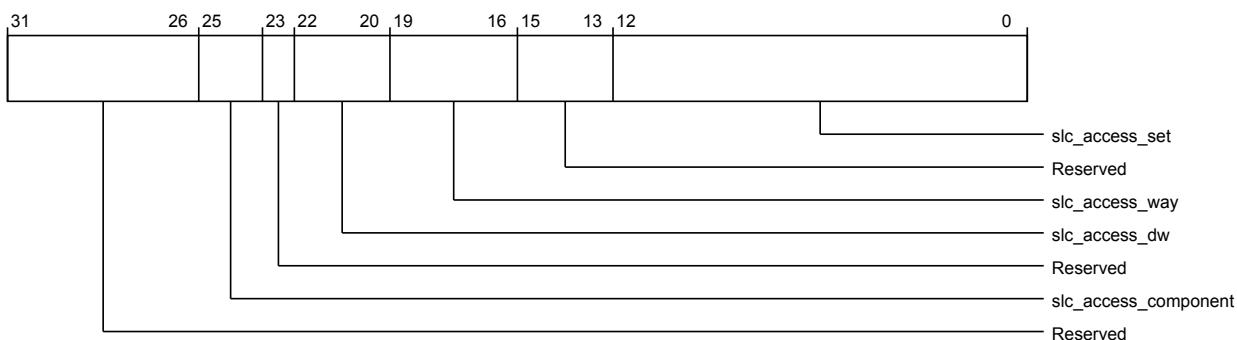
Figure 3-499 por_hnf_por_hnf_cfg_slcsf_dbgrd (low)
