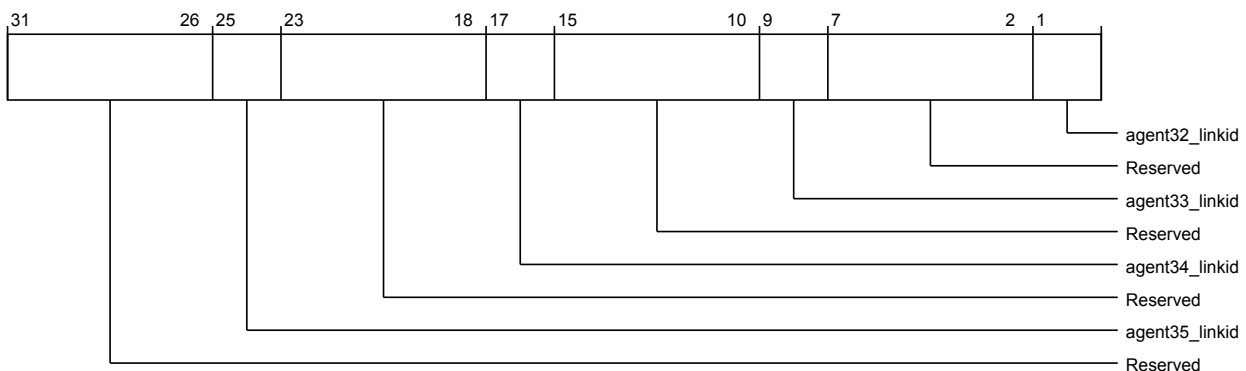
Figure 3-1001 por_cxg_ha_por_cxg_ha_agentid_to_linkid_reg4 (low)
