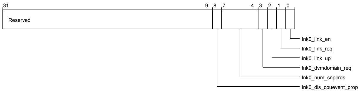
Figure 3-1149 por_cxg_ra_por_cxg_ra_cxprtcl_link0_ctl (low)
