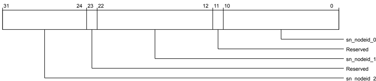
Figure 3-855 por_rnsam_sys_cache_grp_sn_nodeid_reg0 (low)
