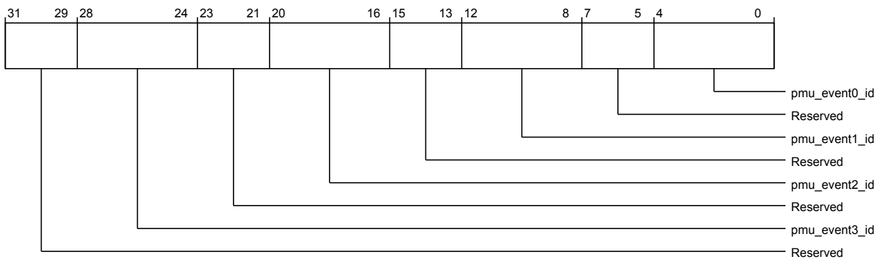
Figure 3-511 por_hnf_por_hnf_pmu_event_sel (low)
