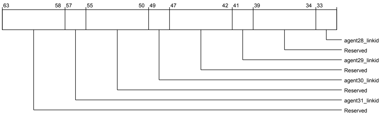
Figure 3-1096 por_cxg_ra_por_cxg_ra_agentid_to_linkid_reg3 (high)
