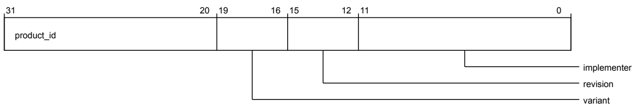
Figure 3-316 por_hnf_por_hnf_ppu_iidr
