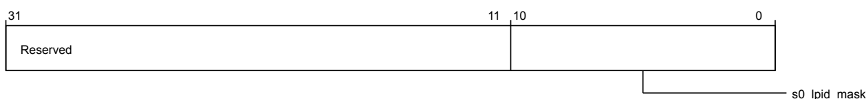
Figure 3-727 por_rnd_por_rnd_s0_port_control (low)
