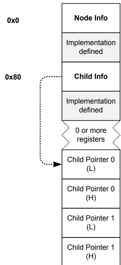
Figure 2-19 Basic node structure with fixed offsets
