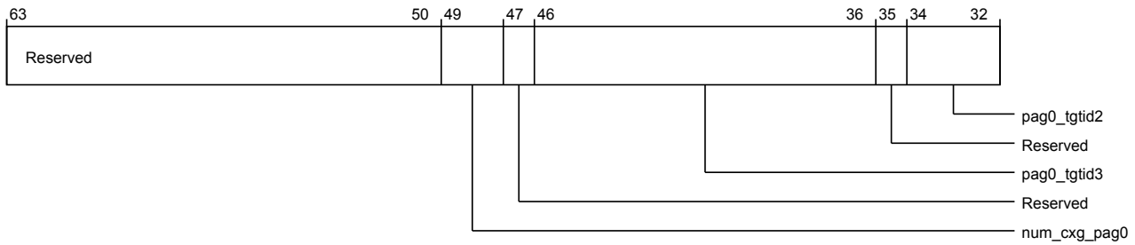
Figure 3-888 por_rnsam_cml_port_aggr_grp0_reg (high)
