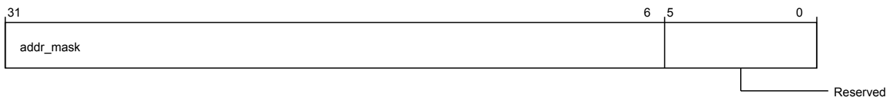
Figure 3-885 por_rnsam_cml_port_aggr_grp0_add_mask (low)
