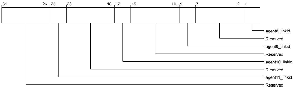
Figure 3-1181 por_cxla_por_cxla_agentid_to_linkid_reg1 (low)
