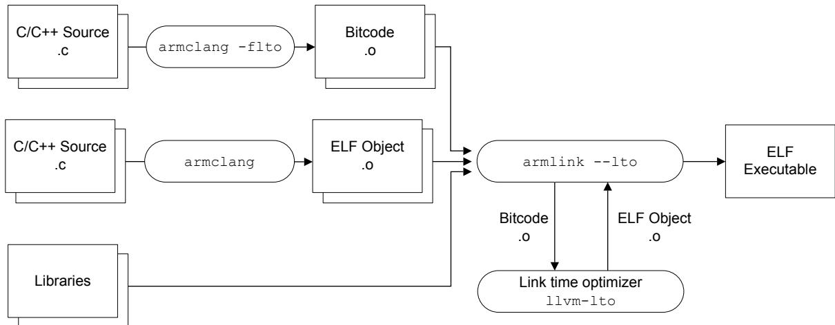
Figure 6-1 Link time optimization
