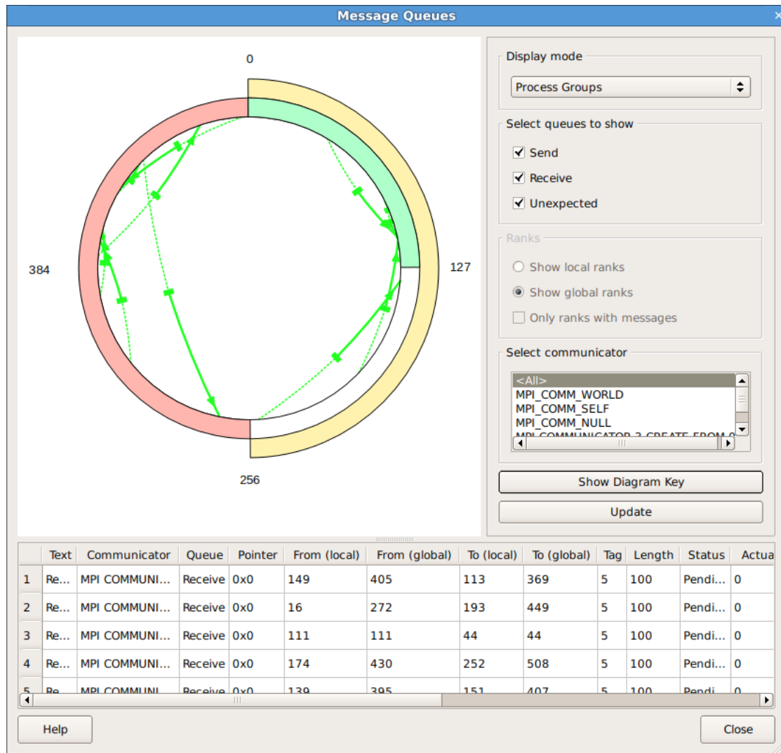
Figure 79: Message Queue Window
