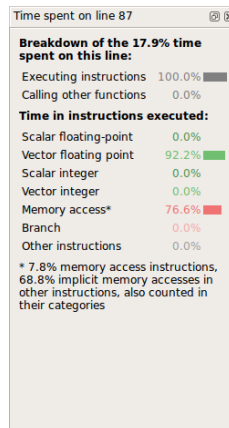
Figure 109: Selected Lines View
