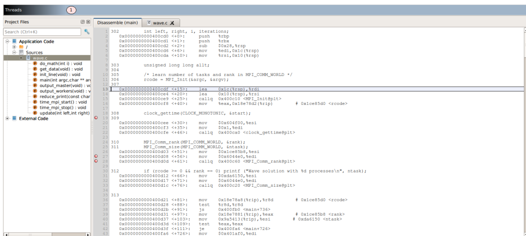
Figure 28: The disassembly viewer tab shows the disassembly of the current symbol with the source code interleaved.
