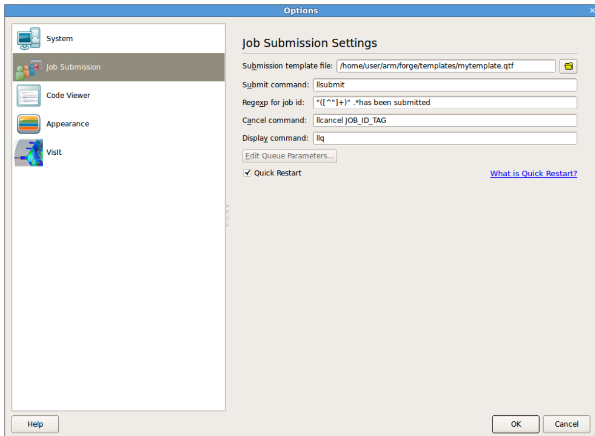
Figure 124: Queuing Systems
