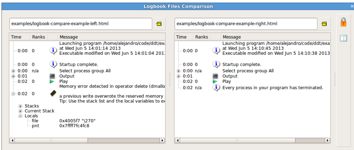
Figure 78: Logbook comparison window with tracepoint difference selected
