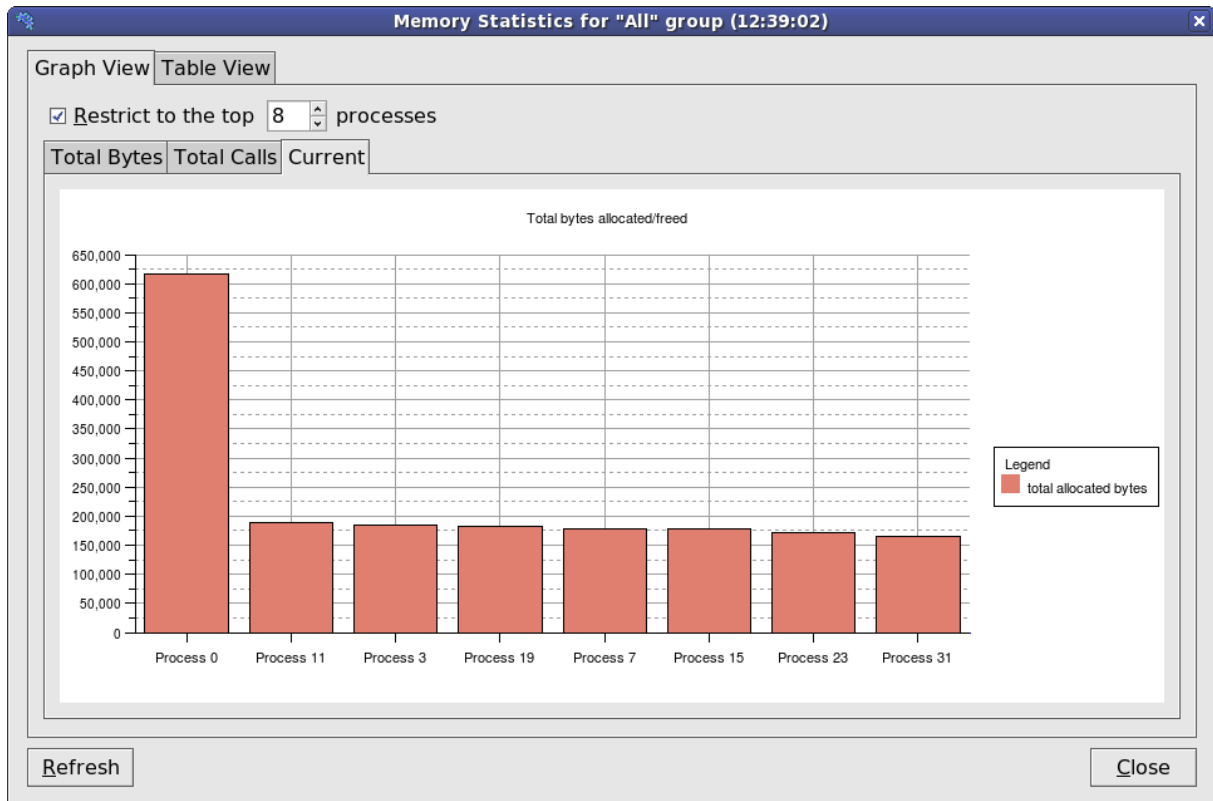
Figure 85: Memory Statistics
