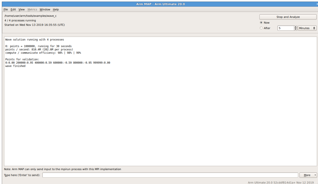
Figure 97: Running window
