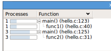
Figure 51: DDT Parallel Stack View
