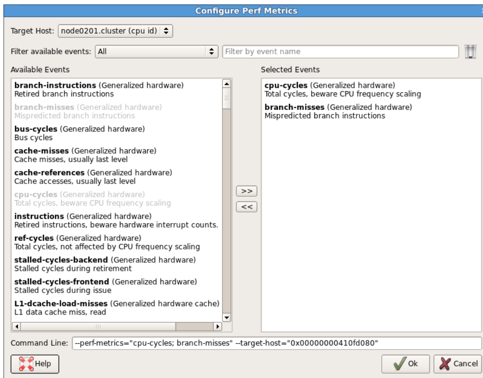
Figure 117: Configure Perf metrics window
