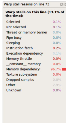
Figure 110: Selected lines view (GPU kernel)
