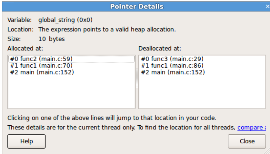
Figure 82: Pointer details
