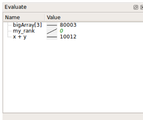
Figure 59: Evaluating Expressions
