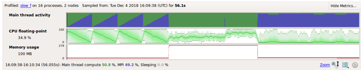
Figure 115: Metrics view
