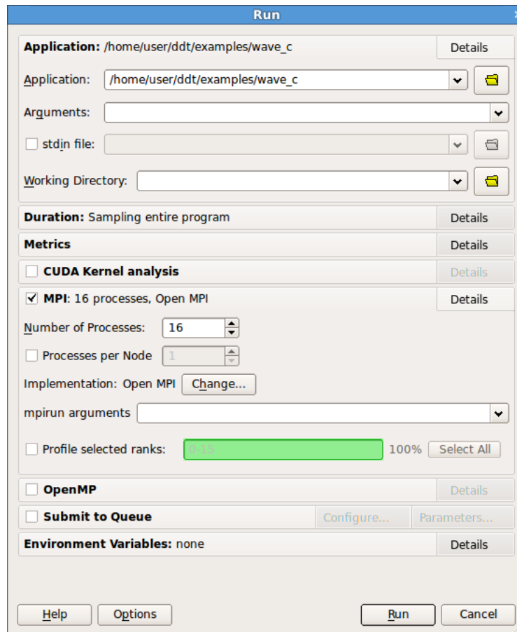
Figure 96: Run window
