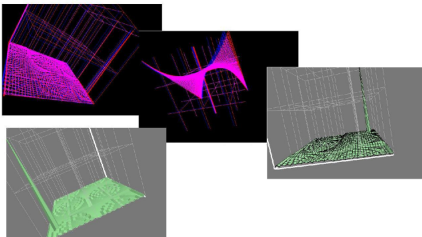
Figure 69: DDT Visualization
