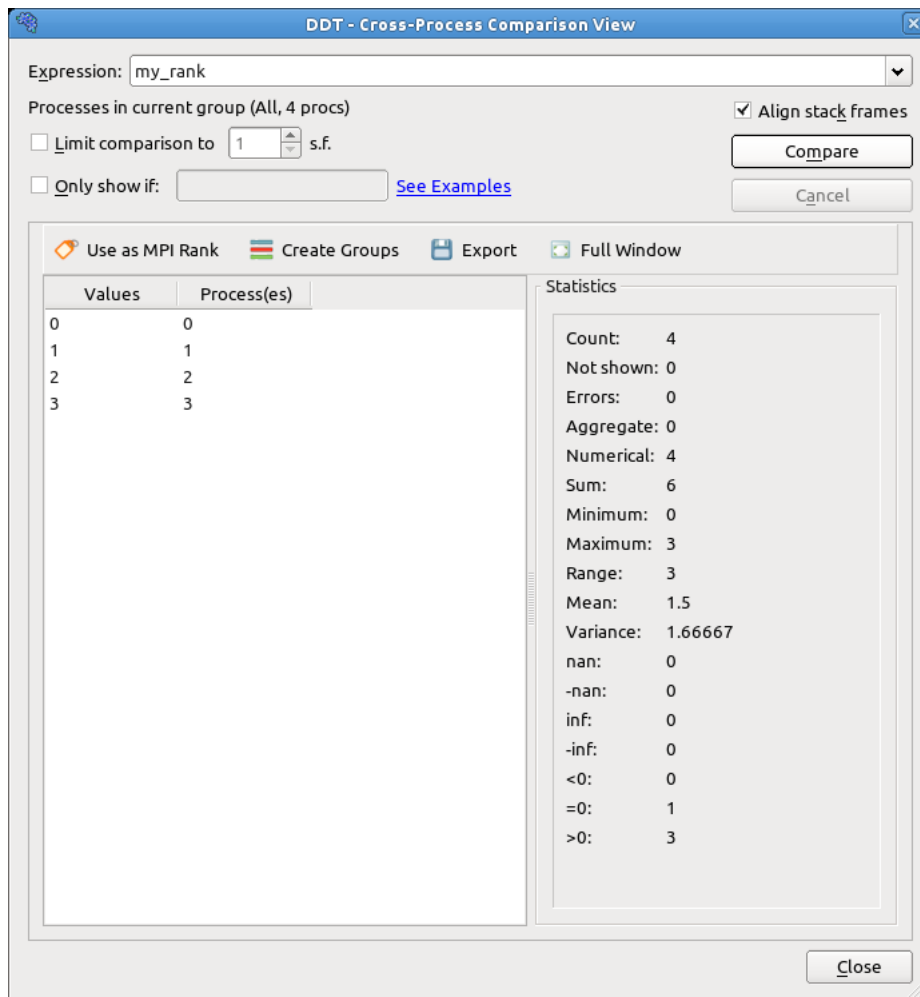
Figure 70: Cross-Process Comparison—Compare View
