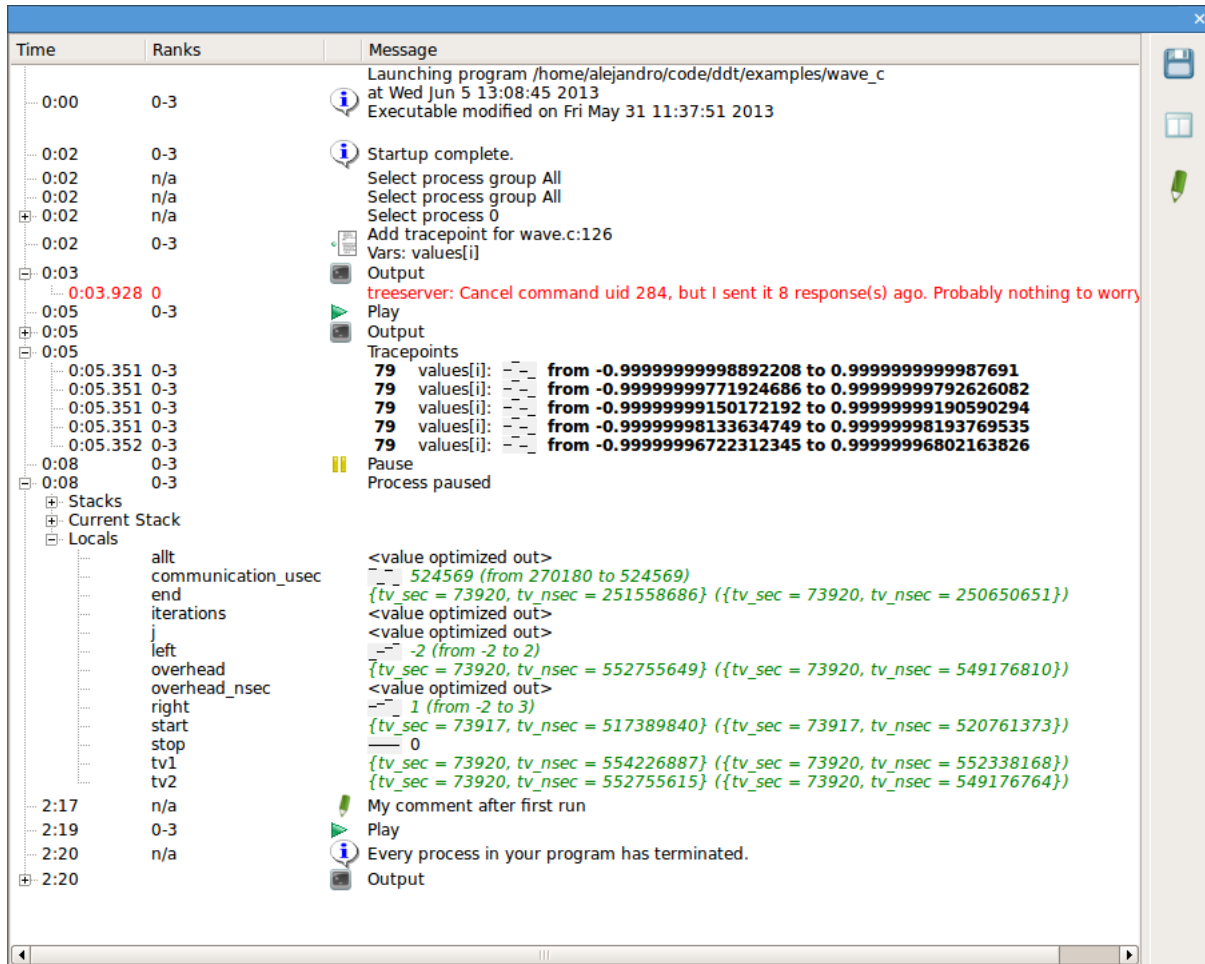
Figure 77: Logbook example of a debug session
