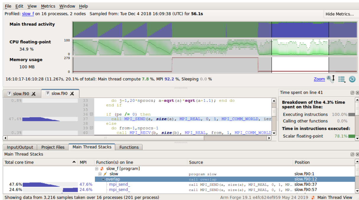
Figure 116: Map with a region of time selected
