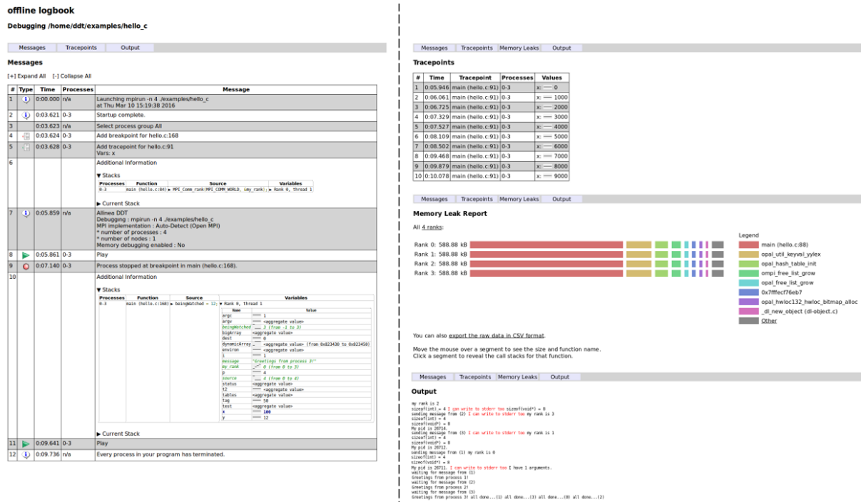
Figure 91: Offline Mode HTML output
