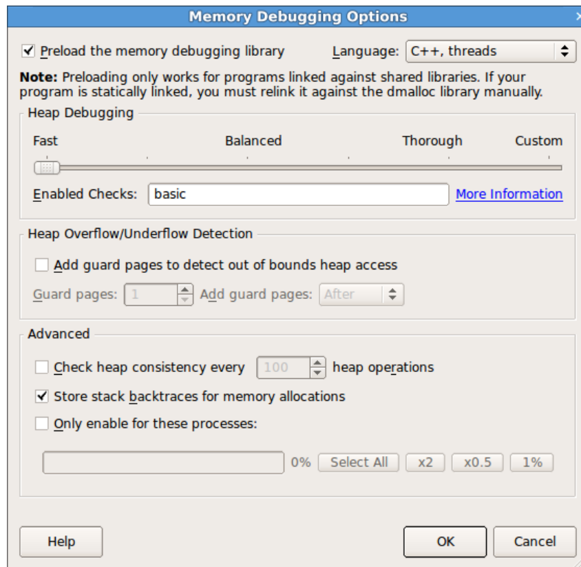
Figure 80: Memory Debugging Options
