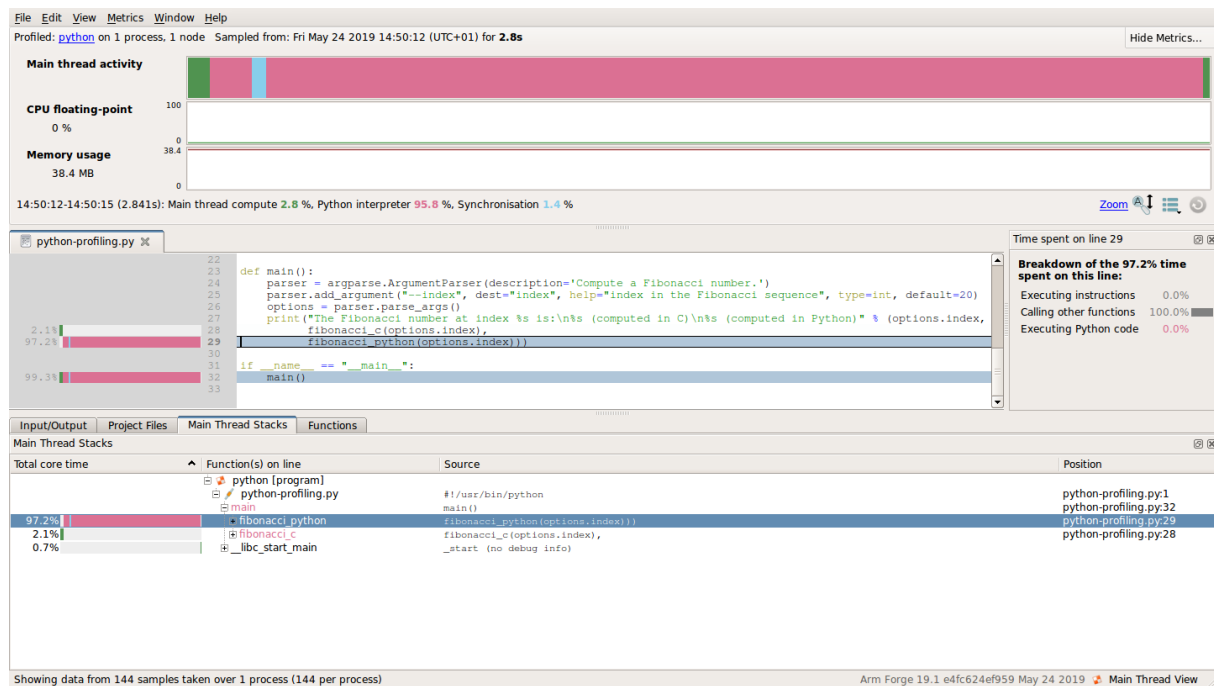
Figure 123: Viewing Python profiling results
