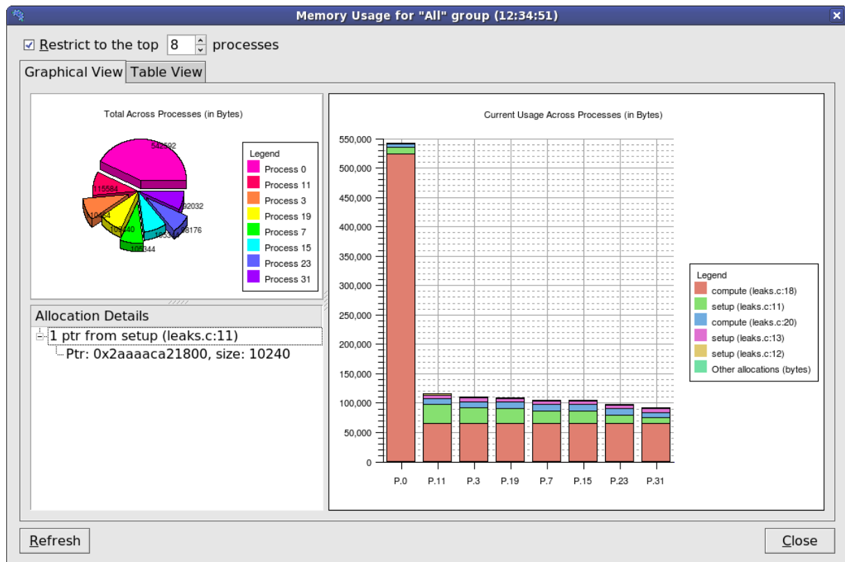
Figure 84: Memory Usage Graphs
