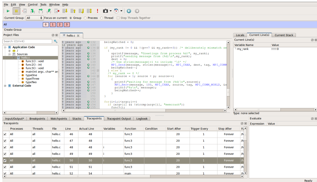
Figure 47: DDT with version control tracepoints
