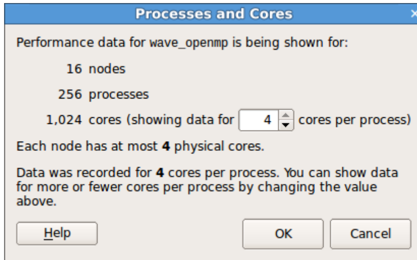
Figure 118: Process and Cores Window
