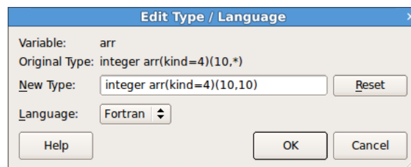
Figure 61: Edit Type window
