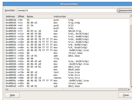
Figure 73: Disassemble Tool
