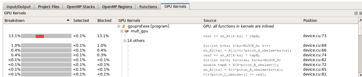
Figure 121: GPU kernels view (with CUDA kernel analysis)
