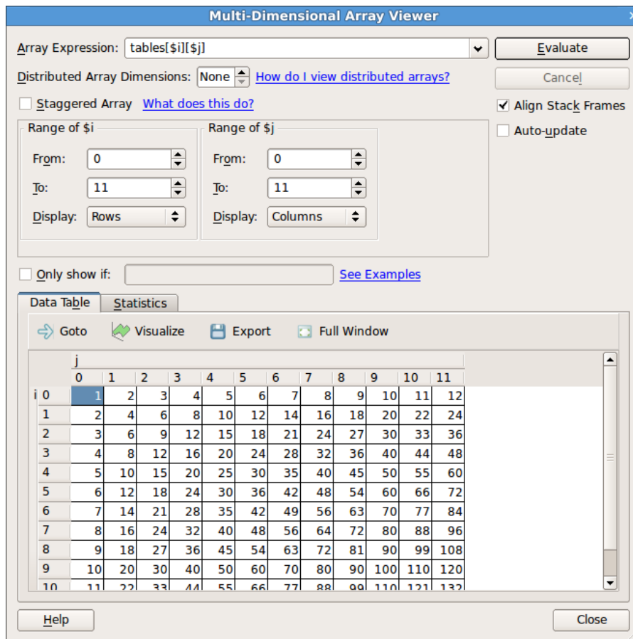
Figure 64: Multi-Dimensional Array Viewer
