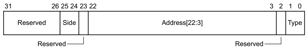
Figure 4-54 Correctable Fault Location Register - TCM, bit assignments
