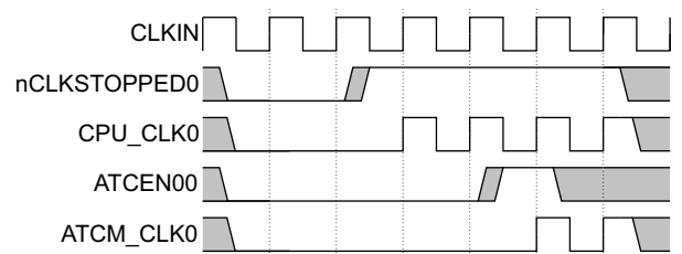
Figure 2-6 Standby, wake-up
