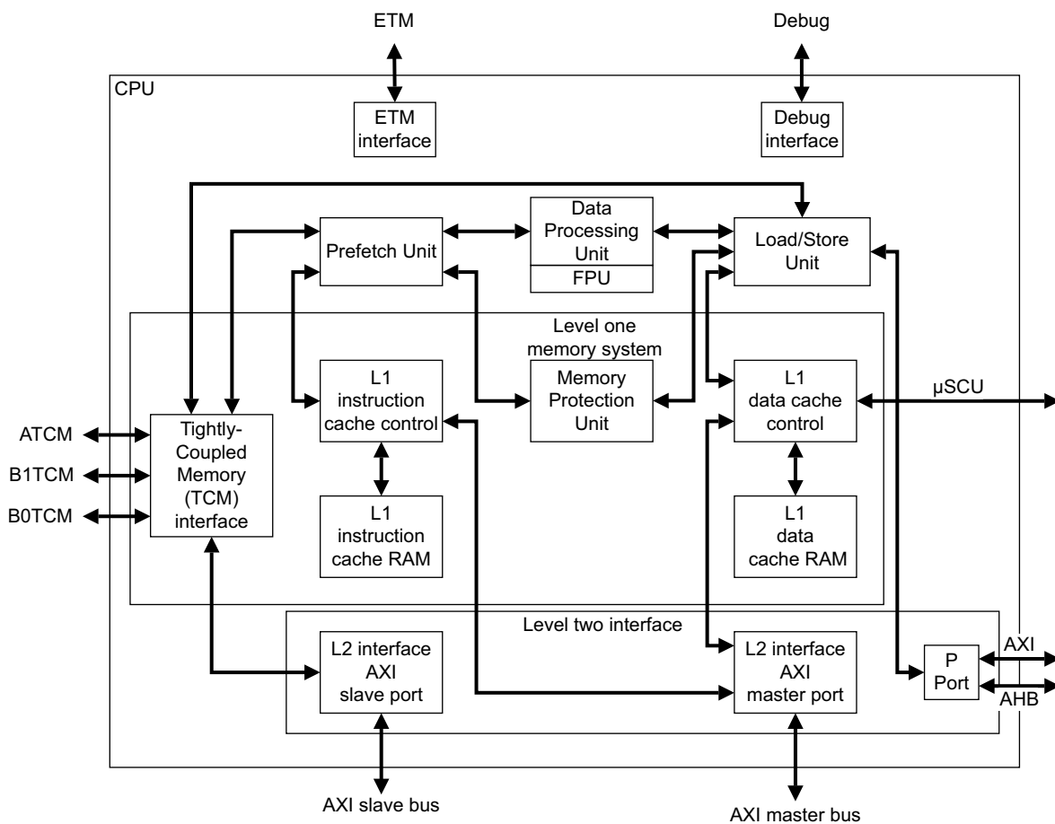
Figure 2-2 CPU block diagram
