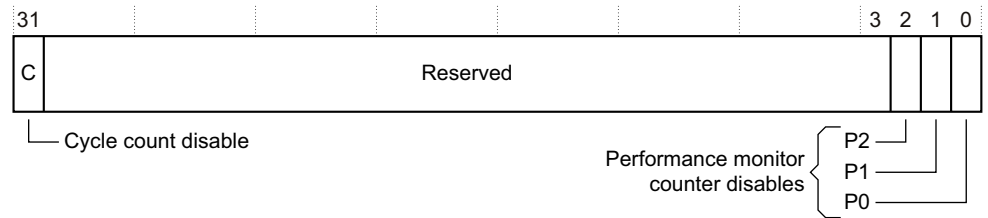
Figure 6-3 PMCNTENCLR Register bit assignments
