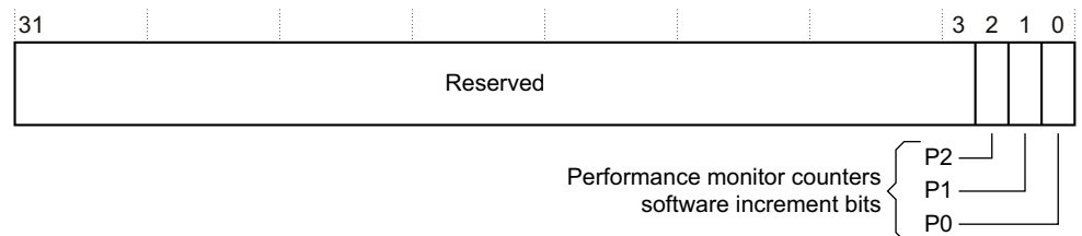
Figure 6-5 PMSWINC Register bit assignments
