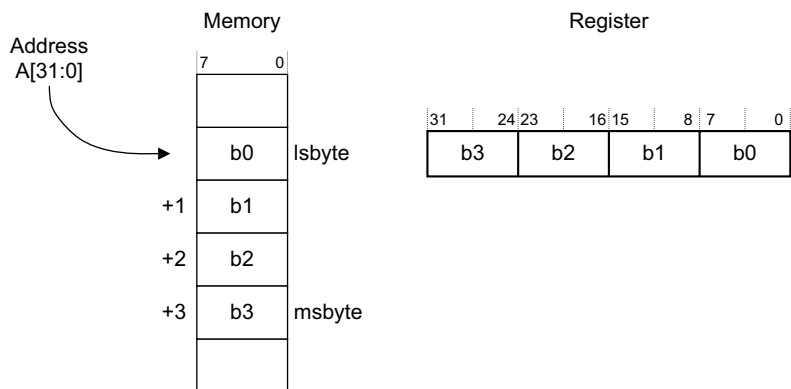
Figure 3-2 Little-endian format
