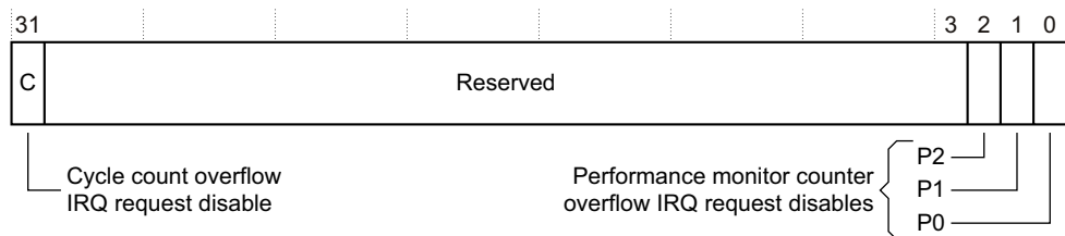
Figure 4-48 VAL IRQ Enable Clear Register bit assignments
