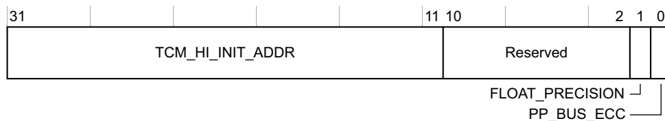
Figure 4-55 Build Options 1 Register bit assignments
