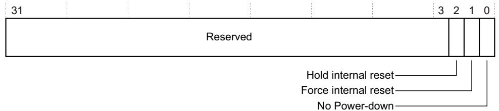
Figure 12-14 DBGPRCR Register bit assignments
