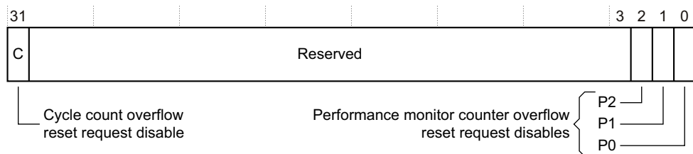
Figure 4-50 nVAL Reset Enable Clear Register bit assignments
