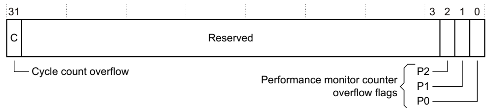
Figure 6-4 PMOVSr Register bit assignments
