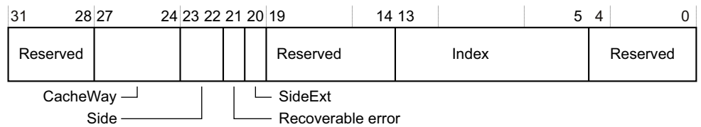
Figure 4-33 Auxiliary fault status registers bit assignments
