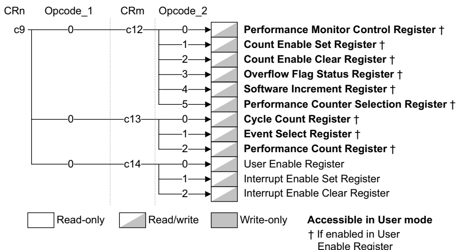
Figure 4-5 System performance monitor registers
