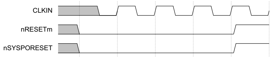
Figure 2-4 Power-on reset
