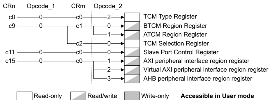
Figure 4-4 TCM control and configuration registers
