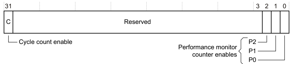
Figure 6-2 PMCNTENSET Register bit assignments
