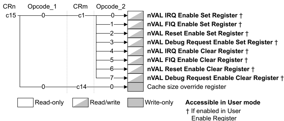
Figure 4-6 System validation registers
