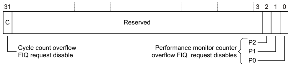
Figure 4-49 nVAL FIQ Enable Clear Register bit assignments
