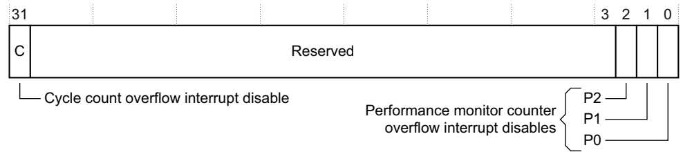
Figure 6-10 PMINTENCLR Register bit assignments
