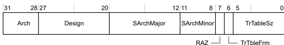
Figure 5-1 JIDR bit assignment
