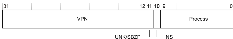
Figure 4-23 TLB VA Register bit assignments
