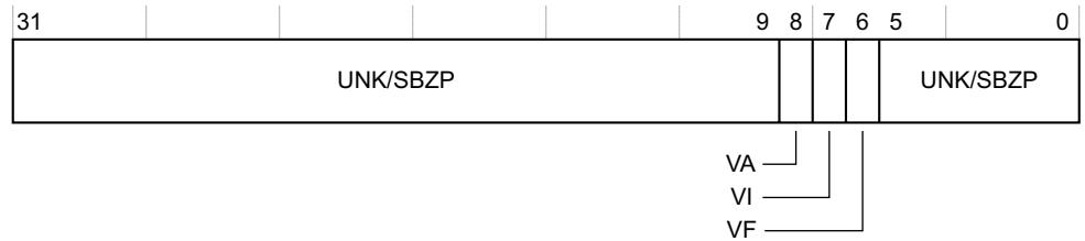
Figure 4-18 VIR bit assignments
