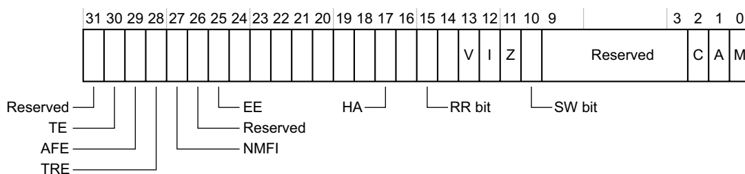
Figure 4-6 SCTLR bit assignments
