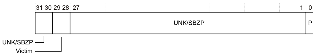
Figure 4-12 TLB Lockdown Register bit assignments
