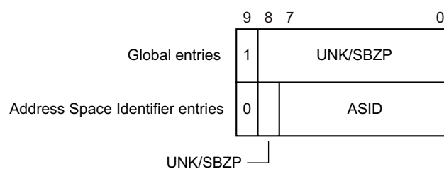
Figure 4-24 Memory space identifier format
