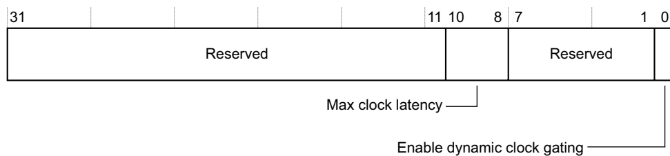
Figure 4-19 Power Control Register bit assignments
