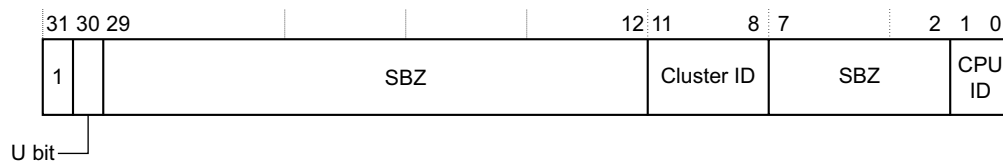
Figure 4-2 MPIDR bit assignments
