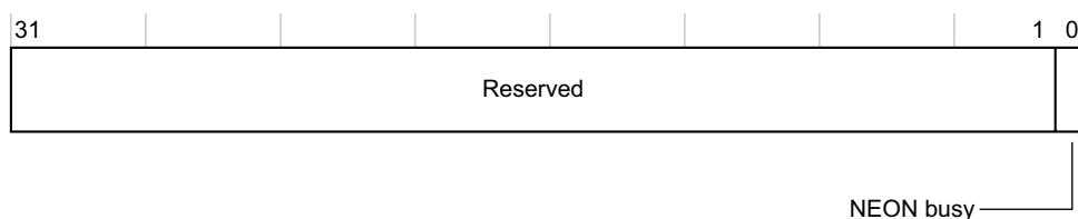
Figure 4-20 NEON busy register bit assignments
