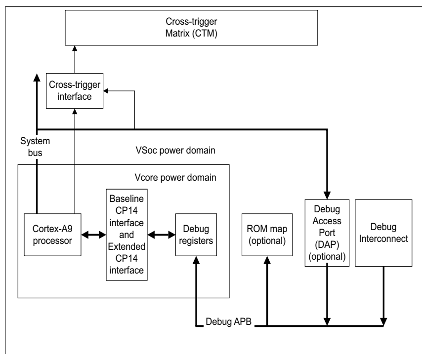
Figure 10-1 Debug registers interface and CoreSight infrastructure
