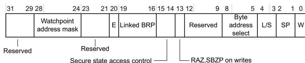
Figure 10-3 Watchpoint Control Registers bit assignments
