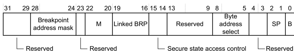
Figure 10-2 Breakpoint Control Registers bit assignments
