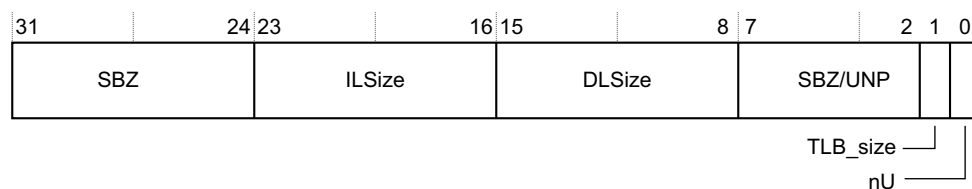
Figure 4-1 TLBTR bit assignments
