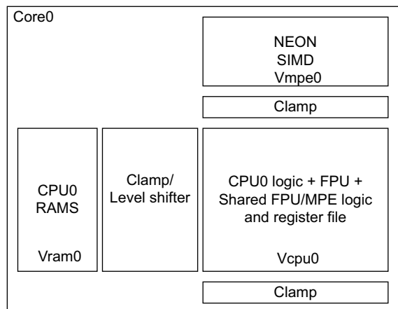
Figure 2-4 Power domains for Cortex-A9 r2 designs
