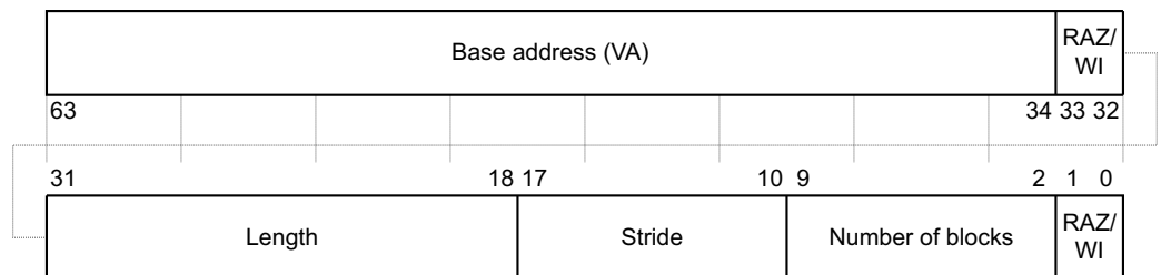
Figure 9-1 Program new channel operation bit assignments
