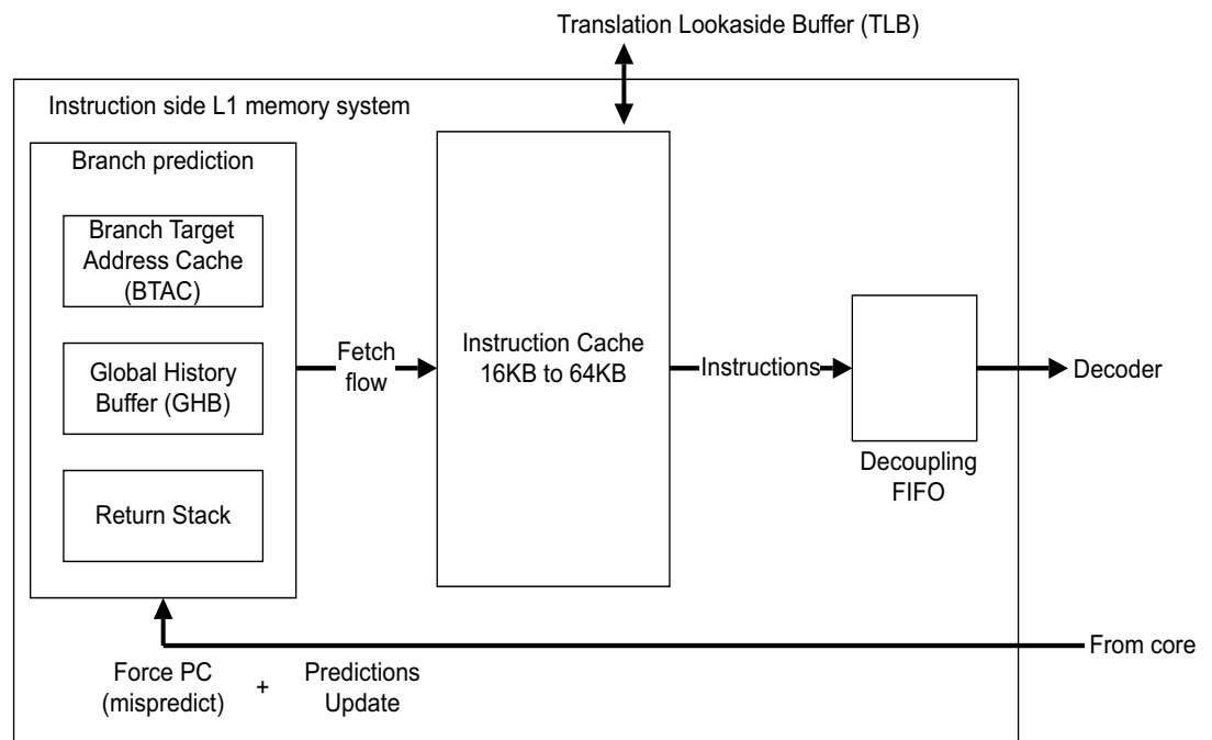
Figure 7-1 Branch prediction and instruction cache
