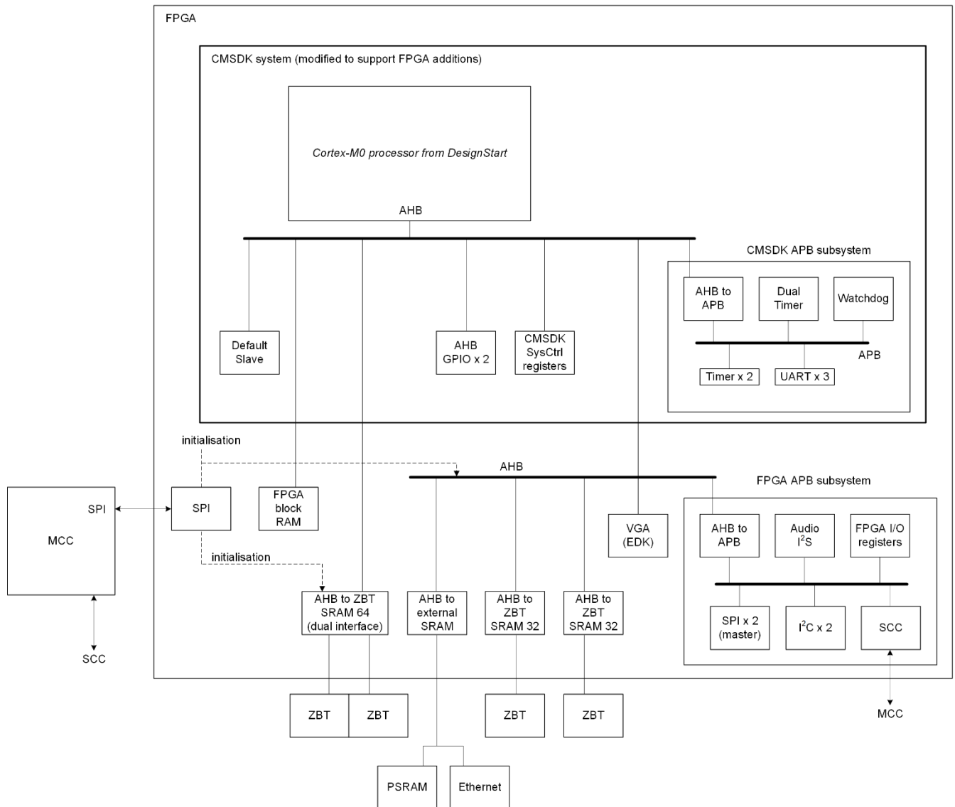
Figure 2-1 System overview
